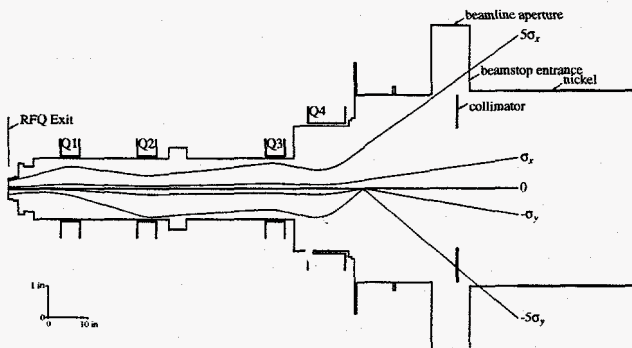
Figure 2: The 1- \sigma (rms) and 5- \sigma beam profiles compared to the minimum aperture in the HEBT beamline.
