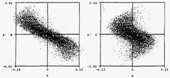
Figure 7: The x - x' phase-space scatter plots for bad tune at start of Q2 (left) and center of Q2 (right).
