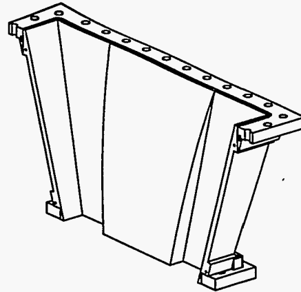
Figure 2. Second Ridged Waveguide Longitudinal Section View
