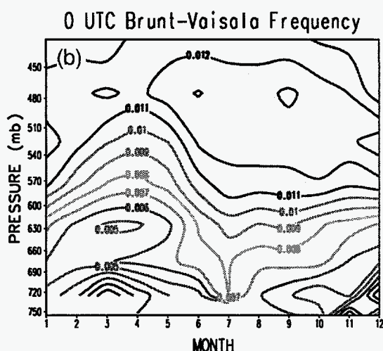
Figure 1. The Brunt Vaisala frequency in the lower troposphere over Mexico City as determined from 50 hPa rawinsonde observations for (a) 1200 UTC, and (b) 00 UTC.
