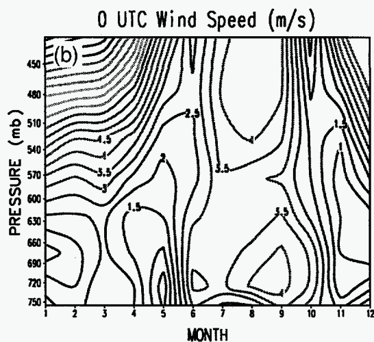
Figure 2. As in Fig. 1, but for wind speed.
