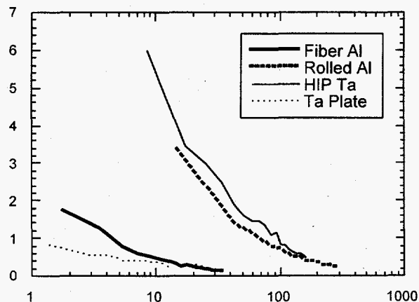
Fig. 9 Plot of D_R^N versus R/d ( d is the average grain diameter).
