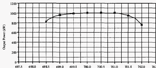
Figure 4: CPI klystron frequency response.
