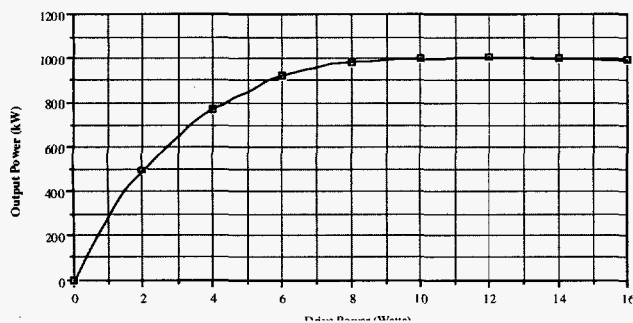
Figure 3: CPI klystron power transfer curve.
