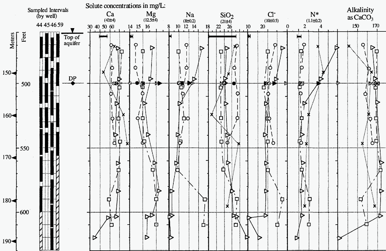
Figure 4a. Selected major solutes are plotted against depth sampled by the straddle-packer system. Solute concentrations are in mg/L; total phosphorous is plotted as P; total nitrogen as N. Sampled intervals are shown with solid bars; diagonal lines indicate intervals sampled with the upper packer inflated and the lower packer uninflated. Estimates of natural (background) solute concentrations are shown in parentheses and with range bars at the top of each plot. Thief and USGS pump samples (500') are illustrated with lined and filled symbols, respectively, for the respective wells. Symbols for wells: \square - USGS-44; \circ - well 45; \triangleright - well 46; \times - USGS-59. Solute concentrations for Mg, Na and Cl are not shown for well USGS-59 because they plot off the graphs (see Figure 4b).
