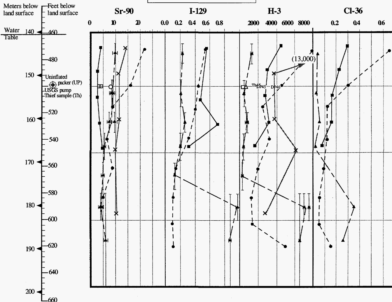
Figure 5. Plots of H-3, I-129 and Sr-90 vs. depth for wells USGS-44 through 46 and 59. Units are in pCi/L. Thief (TS) and U.S. Geological Survey open-hole submersible pumps sample (DP) analyses also plotted for comparison as follows: Open square, circle and triangle - USGS pump, uninflated packer and thief sampler, respectively for Well #44; Th45 and DP45, DP46 - thief and dedicated pump analyses for wells 45 and 46 (analyses plot at center of symbols).
