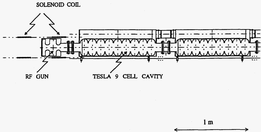
Figure 1: Schematic showing a general layout of an rf gun—focusing solenoid— superconducting linac system.
