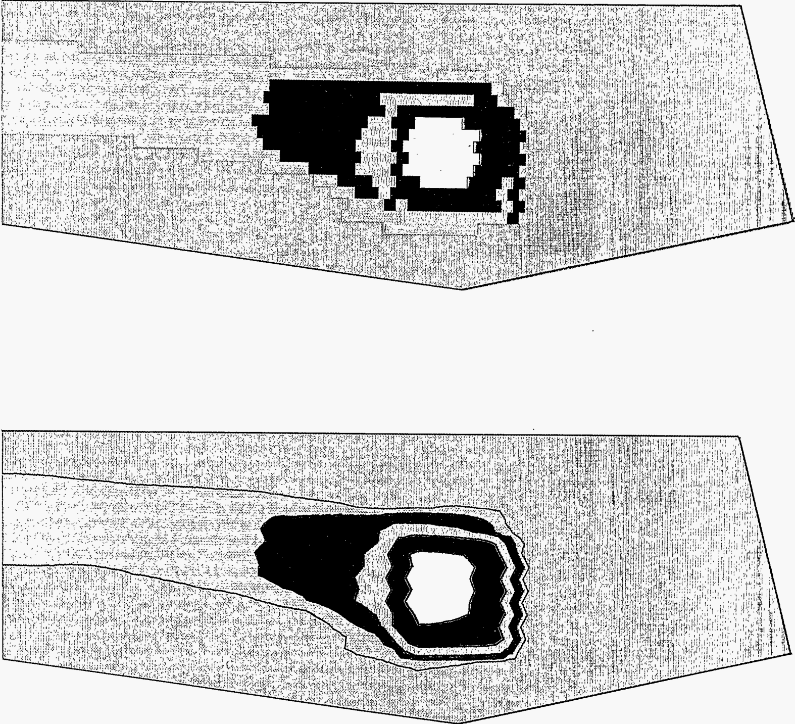
FIGURE 13. KIWI 30-FT GRIDDED AND 270-FT AVERAGED TRU ACTIVITIES. These are the same data as in Figure 12, except that the 241 Am counts have been collected into 270-ft averages centered on a 30-ft grid. The 270-ft averages approximate the spatial resolution of the aerial system at 100 ft AGL. The data are presented both as squares centered on the grid loci and as contour levels derived from the gridded data. Note how well the contour levels in the GZ area match those of Figure 2 in reference 6 (or the aerial data presented as part of Figure 5 in this document).
