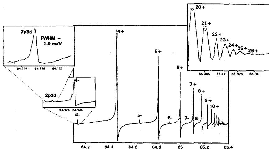
Figure 18. Photoionization yield measurements of doubly excited autoionizing states of helium. A resolution of 1 meV at 64 eV is obtained for the very narrow (few \mu\text{eV} ) 2p3d ( 2,-1, ) state. (Schulz et al., 1996.)
