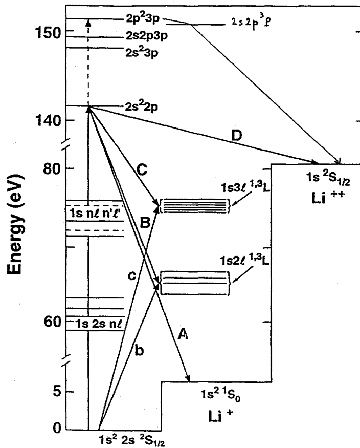
Figure 23. Energy levels of lithium showing multiply excited states.
