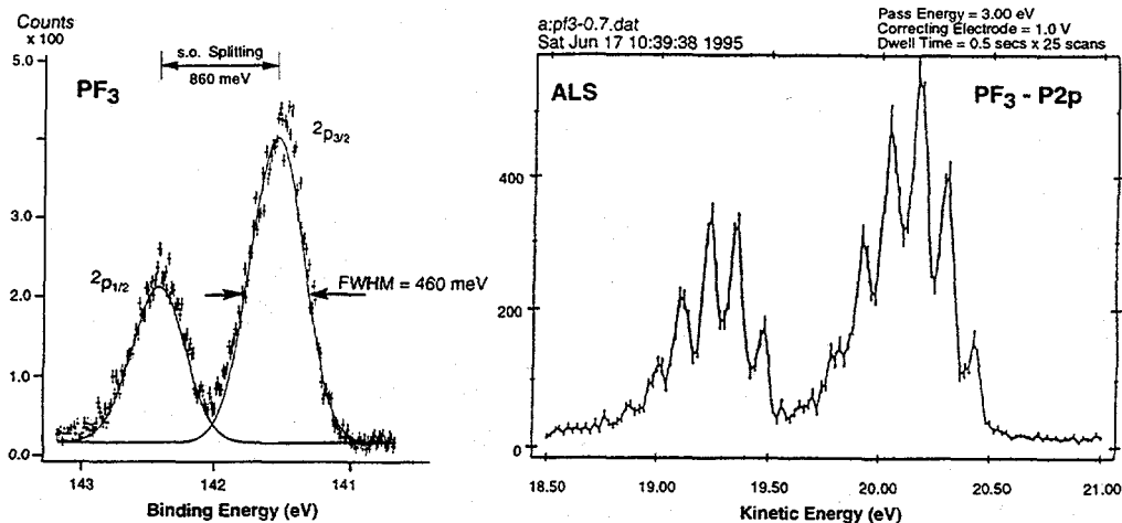
Figure 12. Photoemission from \text{PF}_3 showing fine structure splitting and (ALS spectrum only vibrational) ligand-field splitting. (Canadian Grashopper spectrum courtesy of Ron Cavell; ALS spectrum obtained by Bozek, et al., 1995.)
