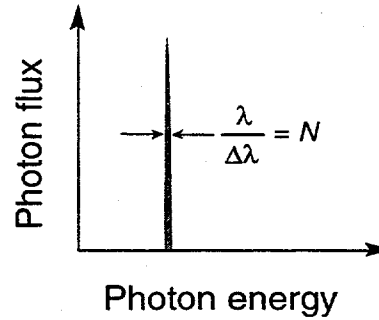
Figure 5. Synchrotron light sources produce photon beams from bend magnets, undulators and wigglers. Radiation emitted from an undulator is spatially contained in a narrow cone, producing an extremely bright and essentially monochromatic (with harmonics) photon beam.
