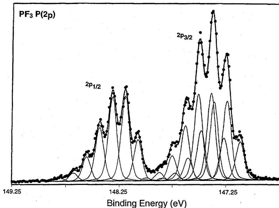
Figure 13. Photoemission from \text{PF}_3 showing vibrational and ligand-field splitting. (Bozek et al., 1995.)
