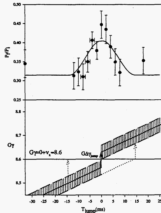
Figure 2. Energy jump data and schematics. In the top half, solid points are the experiment data, the solid line is the predicted curve. Bottom half shows the energy jump scheme.
