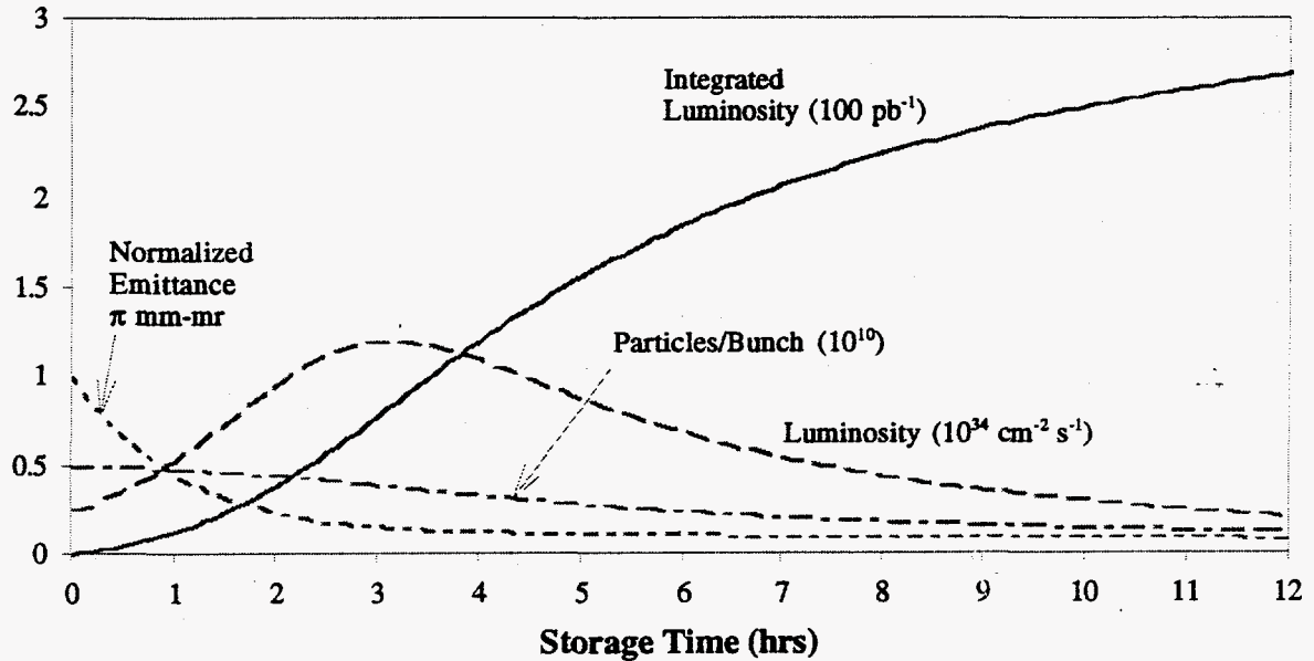
Fig. 3: Beam parameters during a store for high-field RLHC.
