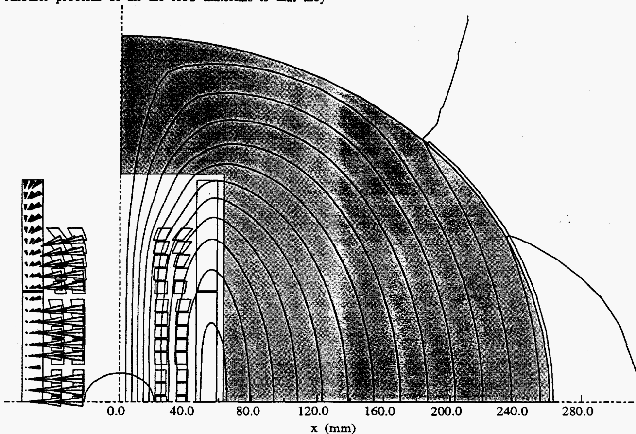
Fig. 5: High-field magnet cross section [23]
