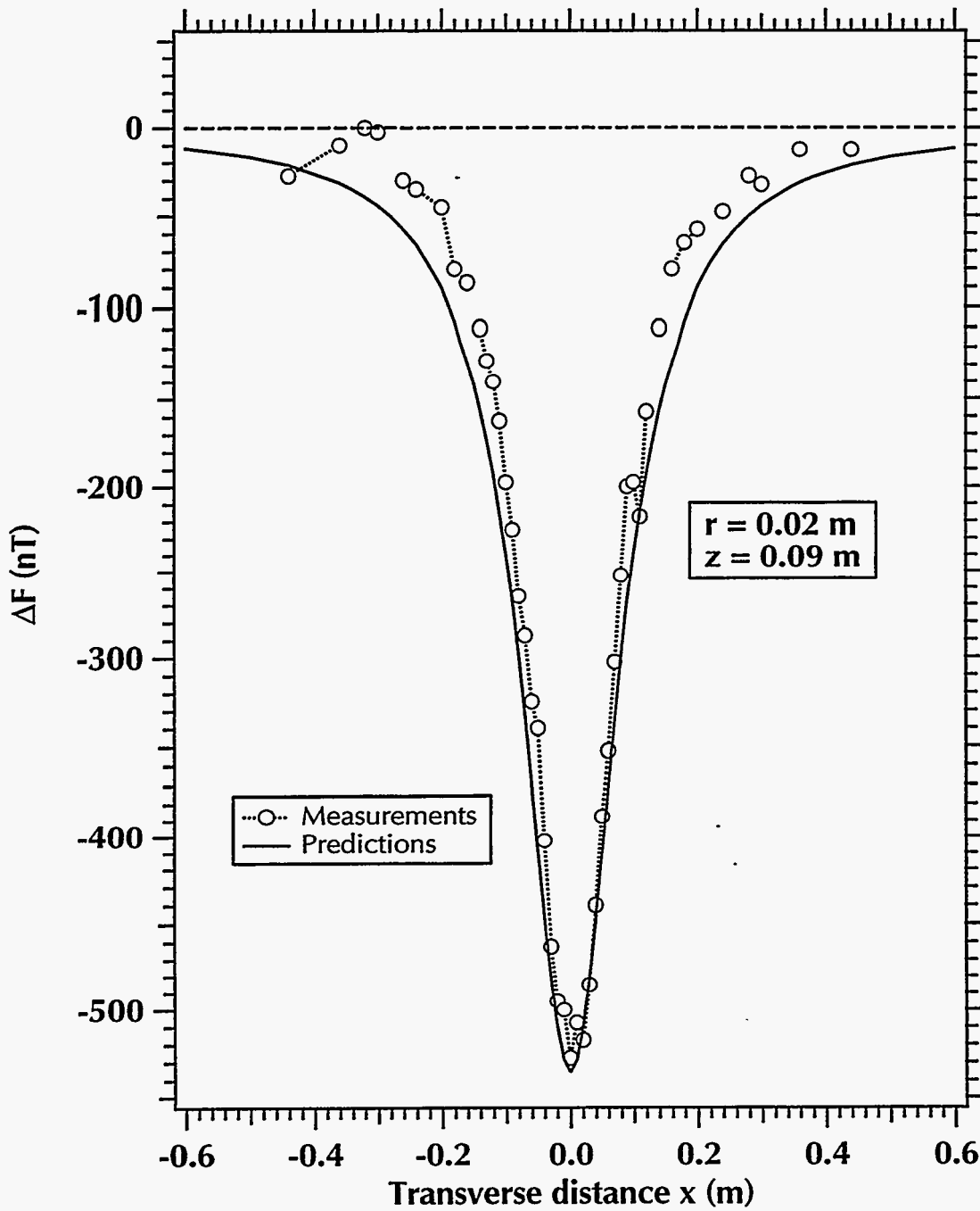
Figure 6.15. Calculated and measured \Delta F for a semi-infinite cylinder with r = 0.02 \text{ m} at a depth z = 0.09 \text{ m} .
