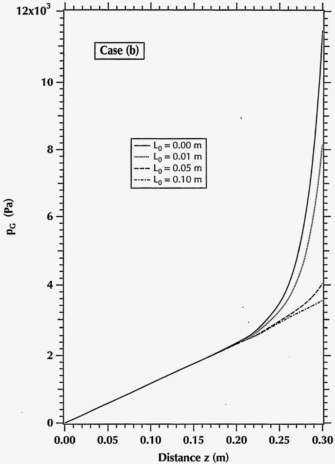
Figure 3.8. p_G (gauge) distribution in case (b) of the vertical FG column of Figure 3.6 with L_d = 0.3 m (EMG 805 TM ferrofluid and PM1 magnet).
