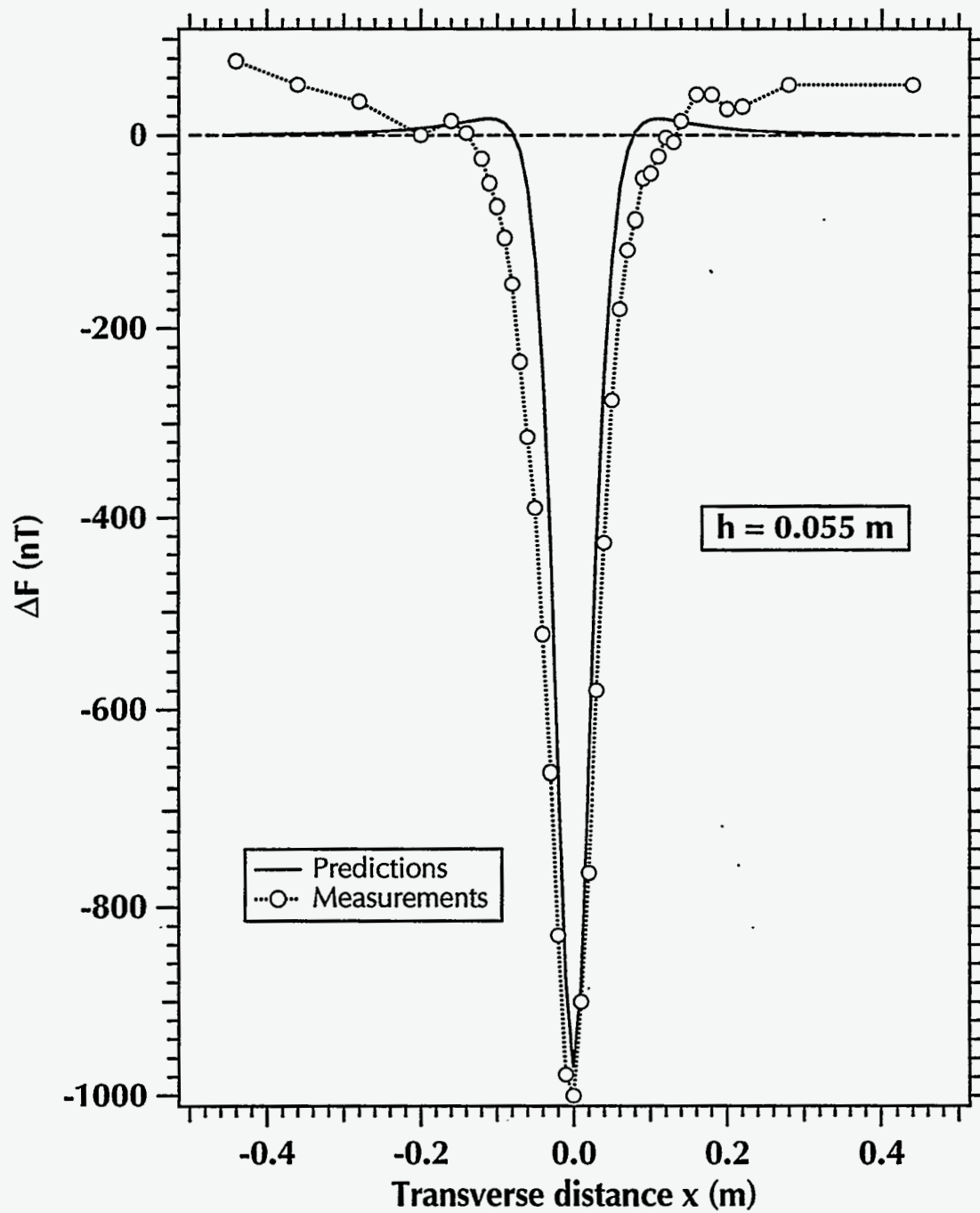
Figure 6.9. Calculated and measured \Delta F for a sphere with V = 100 \text{ ml} at a depth h = 0.055 \text{ m} .
