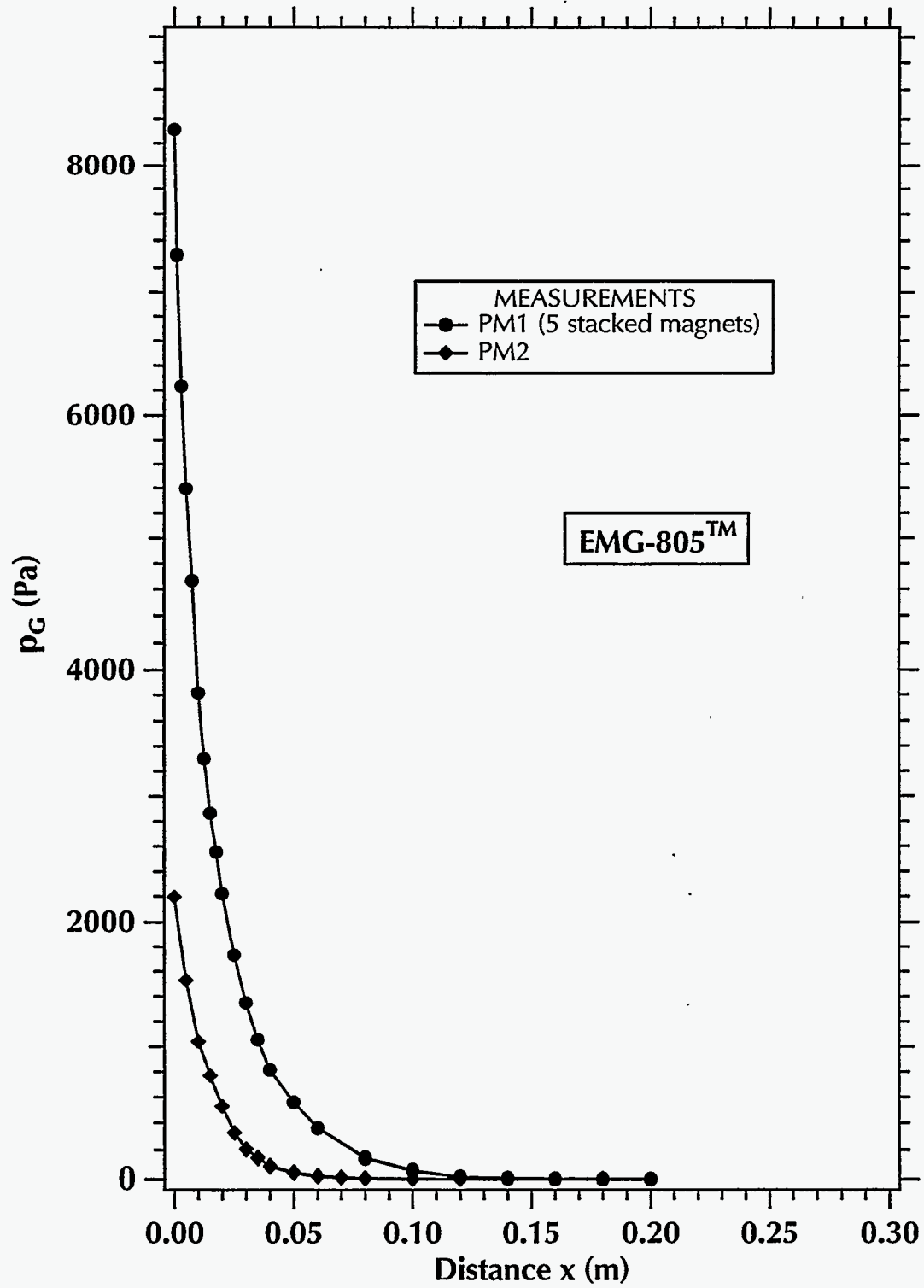
Figure 4.8. Magnetopressure (gauge) measurements using the EMG 805™ ferrofluid.
