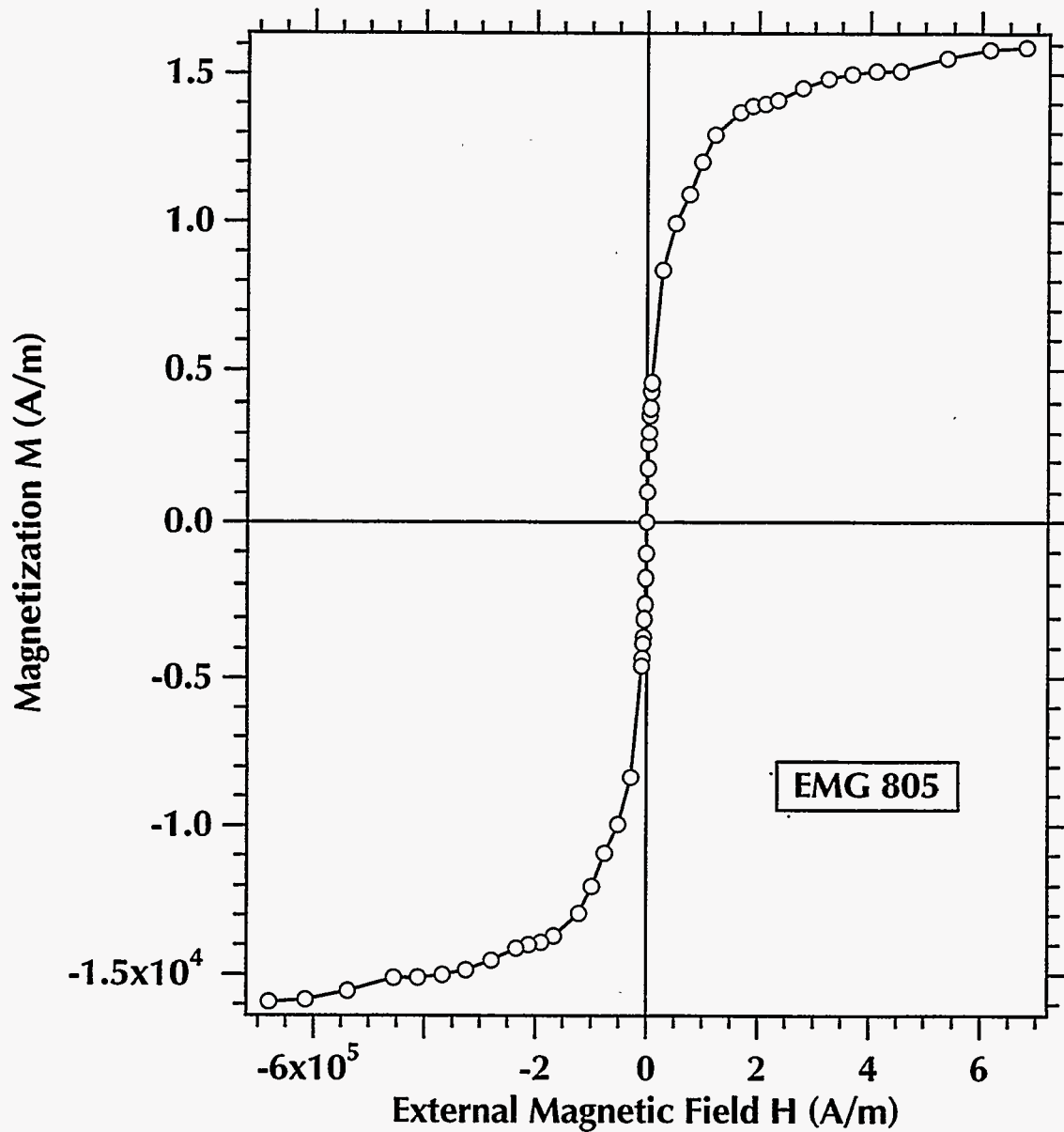
Figure 2.1. Typical magnetization ( M - H ) curve [Nunes and Yu, 1989] for an aqueous ferrofluid (EMG 805 TM , Ferrofluidics Corporation, Nashua, NH).
