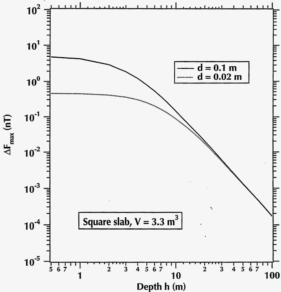
Figure 6.5. Dependence of \Delta F(a, d, x = 0, h) on the depth h to a square slab anomaly of width a , thickness d and constant volume V = 3.3 \text{ m}^3 .
