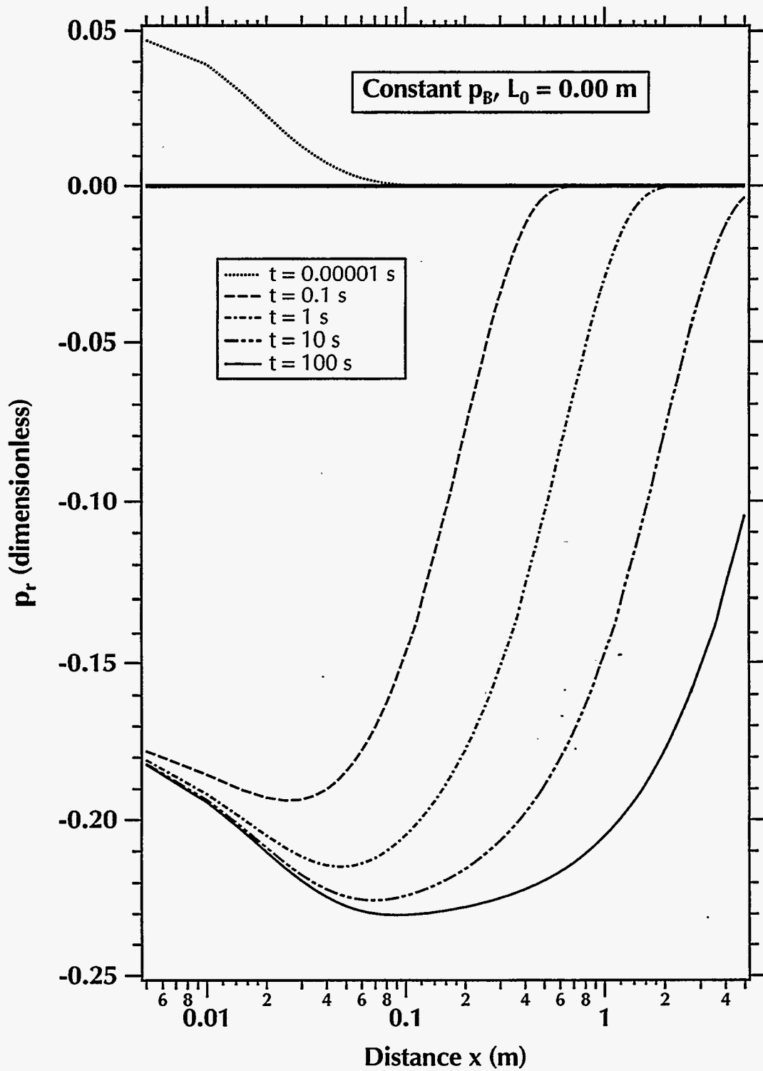
Figure 3.11. p_r distribution for L_0 = 0 m in the horizontal FG column of Figure 3.4 when the pressure at the x = 0 boundary is defined (EMG 805 TM ferrofluid and PM1 magnet).
