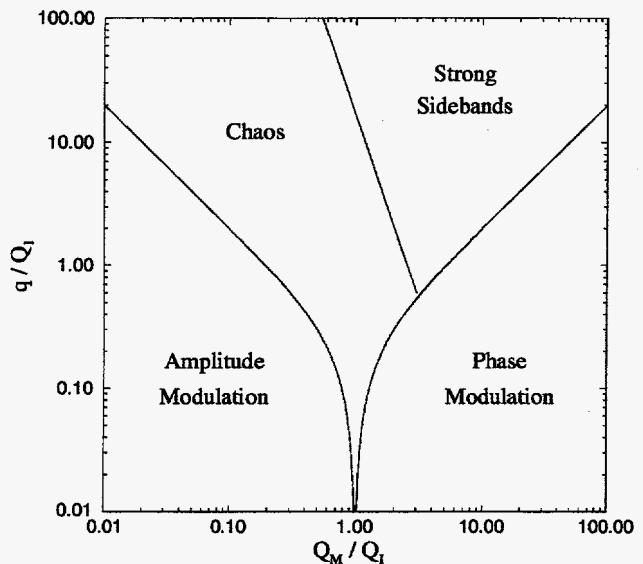
Figure 1: Dynamical phases in the tune modulation parameter plane ( q, Q_M ), for a resonance of order N = 5 .
