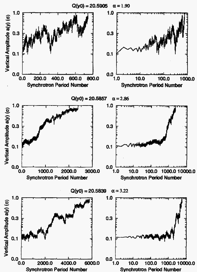
Figure 6: Exponential vertical amplitude growth for particles launched within a horizontal chaotic band. The base tune is Q_{x0} = 20.597 in all cases, so that the horizontal motion sits in the middle of the Q_x = 20.6 resonance. Note the different timescales.
