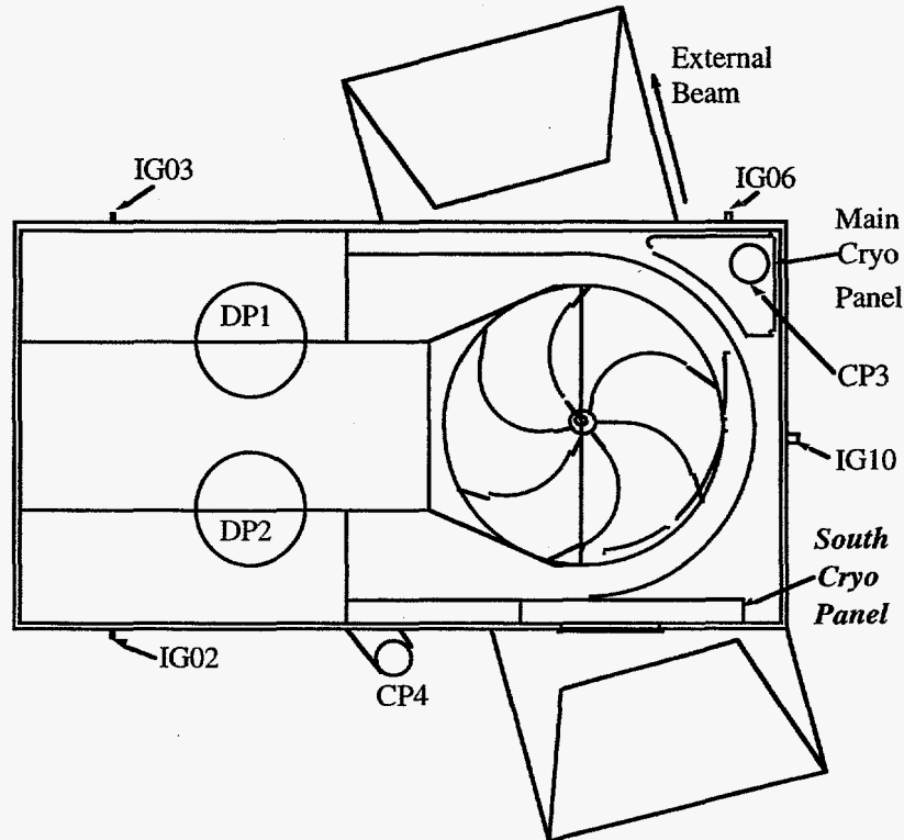
Fig. 3. A plan view of the 88-Inch Cyclotron with the current pumping layout showing the newly installed "South Cryo Panel" and ion gauge IG10 located in between the two cryo panels.
