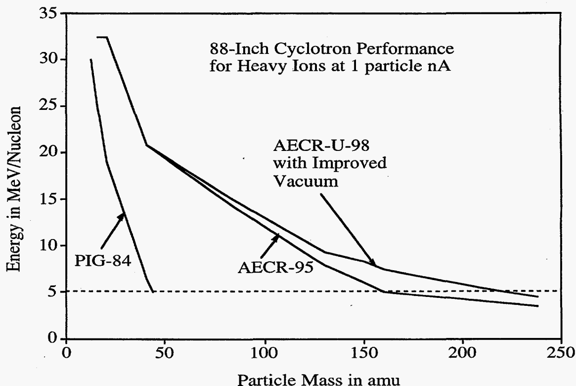
Fig. 1. This shows the energy-mass curves for the cyclotron at an intensity of 1 particle nA.
