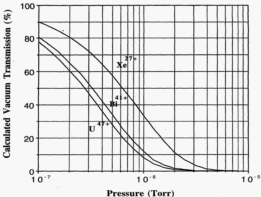
Fig. 6. Calculated beam vacuum transmission versus pressure for \text{Xe}^{27+} , \text{Bi}^{41+} and \text{U}^{47+} ion beams accelerated by the 88-Inch Cyclotron. Improvement ratios are in good agreement with the measured data.
