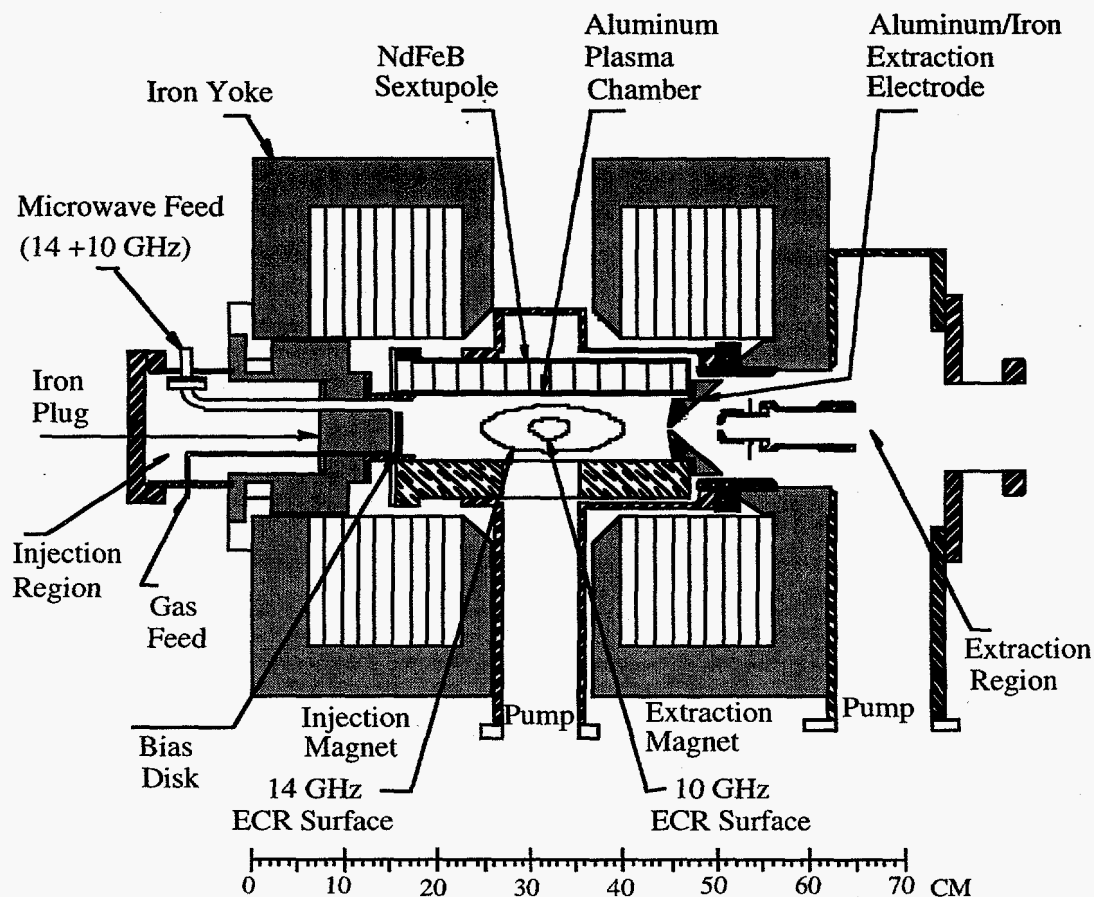
Fig. 2. An elevation view of the LBNL AECR-U ion source.
