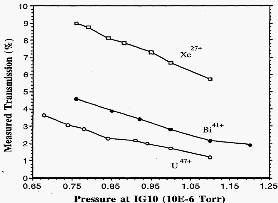
Fig. 4. Measured acceleration transmission versus pressure in the 88-Inch Cyclotron for \text{Xe}^{27+} , \text{Bi}^{41+} and \text{U}^{47+} ion beams.
