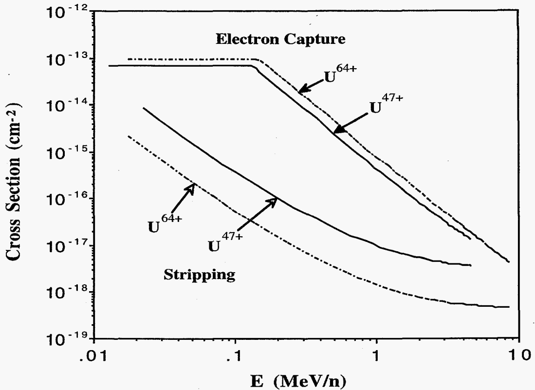
Fig. 5. Calculated electron capture and stripping cross sections for U 47+ and U 64+ ions versus beam energies.
