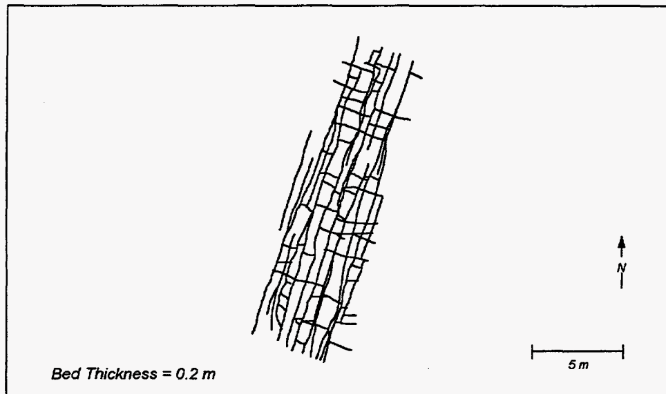
Figure 4.3. Fracture network map made of the outcrop at Scullys Gap, 33 km South of Kemmerer, Wyoming. More than one set of fractures is present, reflecting fractures that are related to regional and local tectonics, as well as fractures that are associated with weathering. Regional fractures are the longest fractures. The azimuth of the regional fracture trend is N19°E. Bed thickness of the sandstone layer at this outcrop is 0.2 m.
