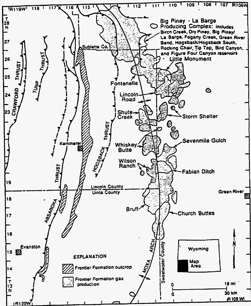
Figure 2.6. Frontier formation gas production from the Moxa Arch and La Barge platform in west Green River Basin. Frontier formation outcrops in the Thrust Belt are also shown. There are more than 25 field names for producing areas on the Moxa arch and La Barge platform, but field boundaries are often defined by lease ownership and unitized areas rather than geologic changes. Reservoirs with >5 BCF cumulative production through December 1990 are labeled. Barlow & Haun, Inc. file maps.
