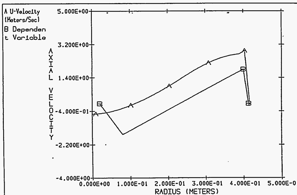
Figure 3-34. MEASURED AND CALCULATED AXIAL VELOCITY COMPONENT 1.07 METERS FROM THE BURNER IN THE CCRL TUNNEL FURNACE
