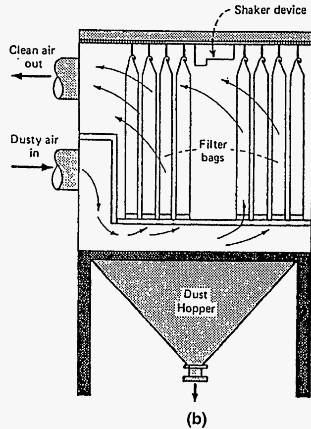
Figure 7-32. FELTED MEDIA SHOWING DISTRIBUTION OF DUST (a) AND SINGLE-COMPARTMENT BAGHOUSE FILTER WITH SHAKER (b)
