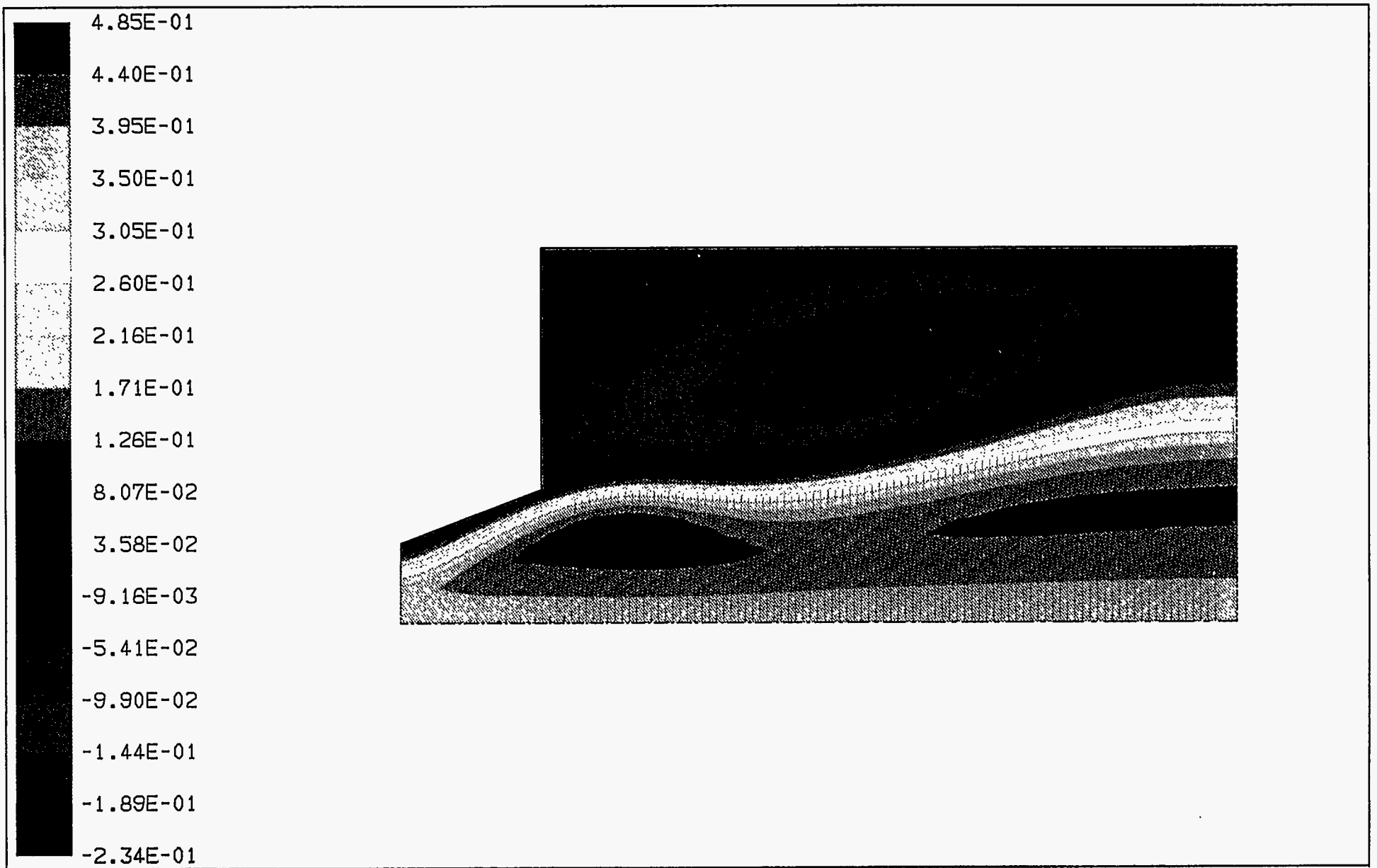
Figure 3-40. STREAM FUNCTION, IN SQUARE METERS/SECOND, IN THE DEMONSTRATION BOILER FOR A TURBULENCE INTENSITY OF 30%
