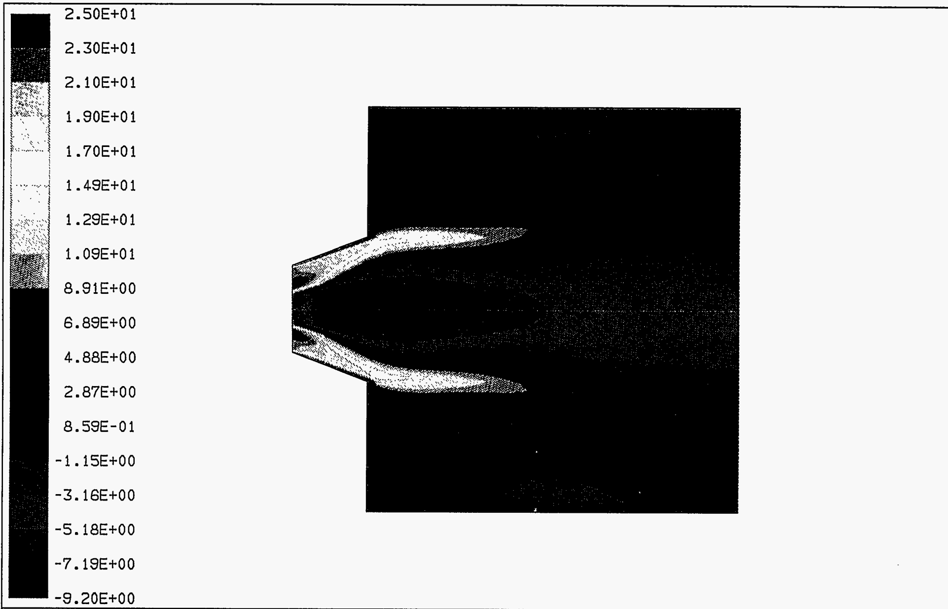
Figure 3-49. RECIRCULATION ZONES, IN METERS/SECOND, IN THE DEMONSTRATION BOILER FOR TERTIARY TO SECONDARY AIR SPLITS OF 65 TO 35%
