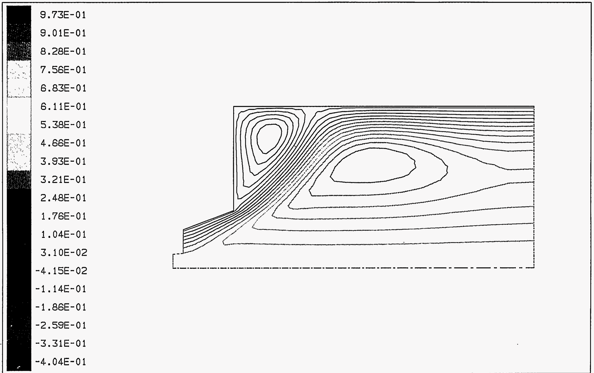
Figure 3-42. STREAM FUNCTION, IN SQUARE METERS/SECOND, IN THE DEMONSTRATION BOILER SHOWING THE RECIRCULATION ZONES
