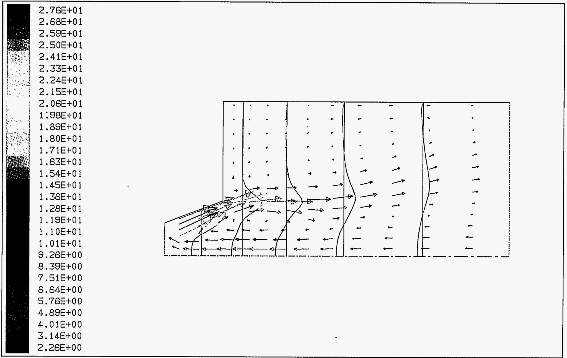
Figure 3-44. VELOCITY VECTORS, IN METERS/SECOND, FOR BURNER CONFIGURATION B
