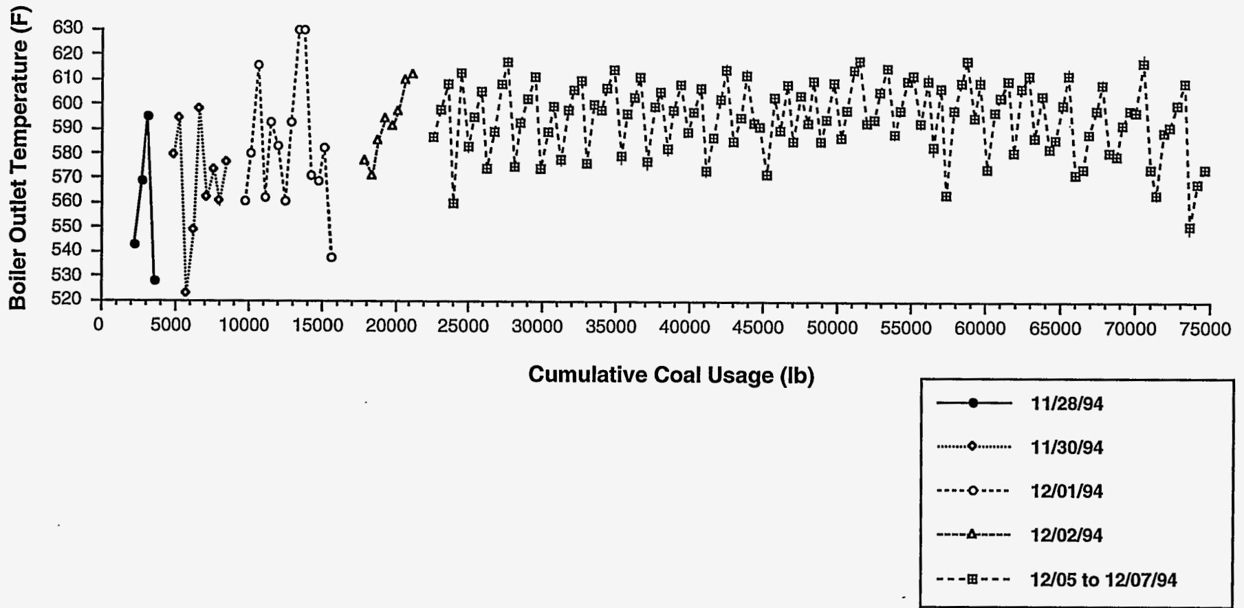
Figure 3-11. BOILER OUTLET TEMPERATURE AS A FUNCTION OF COAL CONSUMPTION WHEN FIRING AT 12.7 TO 12.8 MILLION BTU/H
