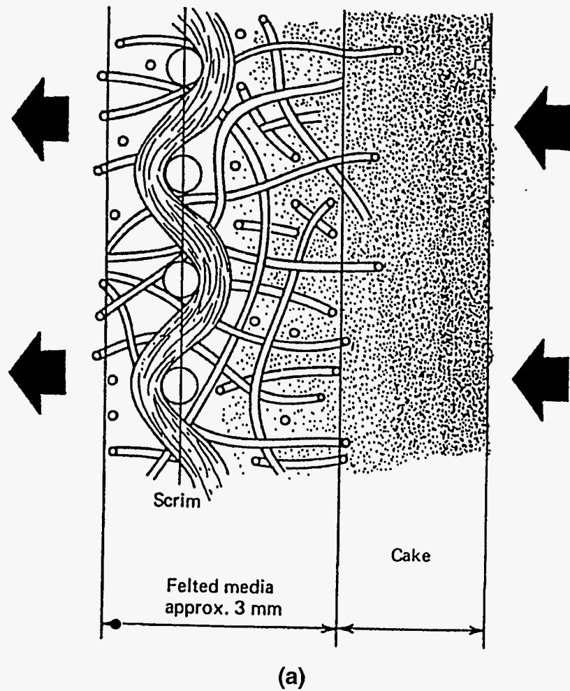
Figure 7-32. FELTED MEDIA SHOWING DISTRIBUTION OF DUST (a) AND SINGLE-COMPARTMENT BAGHOUSE FILTER WITH SHAKER (b)
