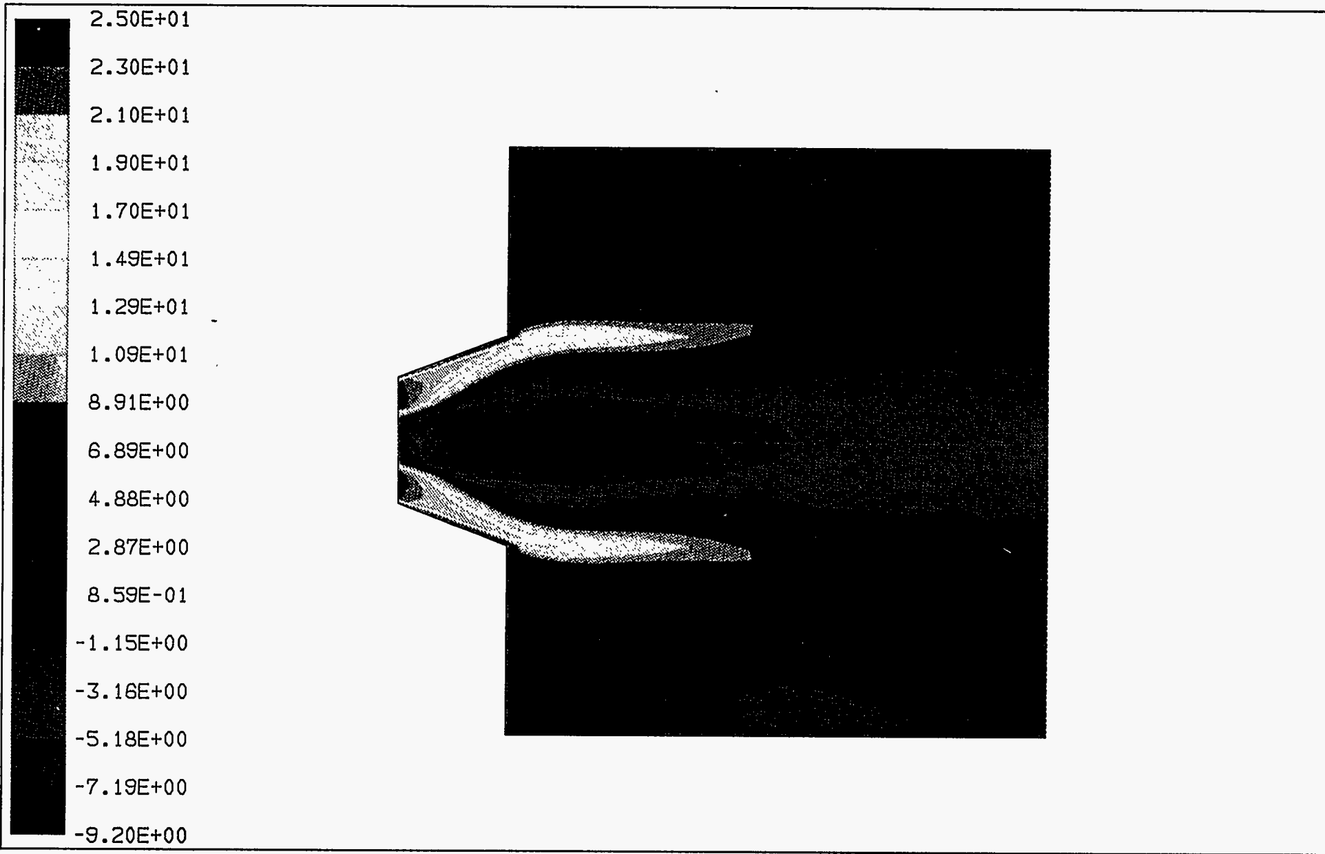
Figure 3-50. RECIRCULATION ZONES, IN METERS/SECOND, IN THE DEMONSTRATION BOILER FOR TERTIARY TO SECONDARY AIR SPLITS OF 70 TO 30%
