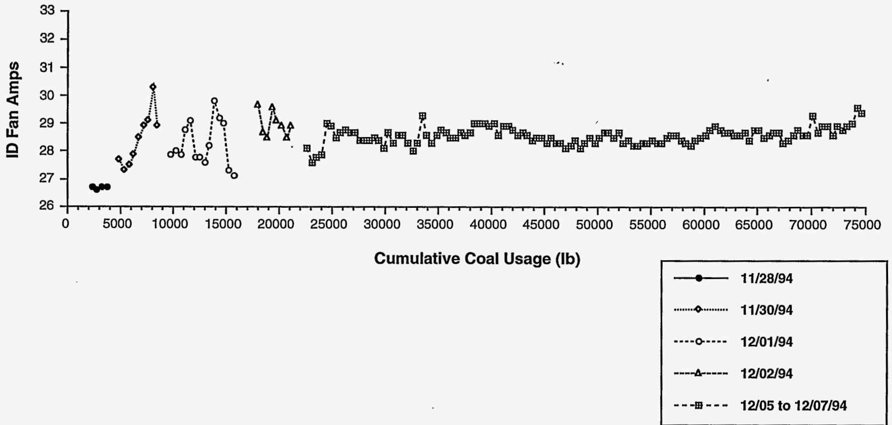
Figure 3-9. ID FAN AMPERAGE AS A FUNCTION OF COAL CONSUMPTION WHEN FIRING AT 12.7 TO 12.8 MILLION BTU/H
