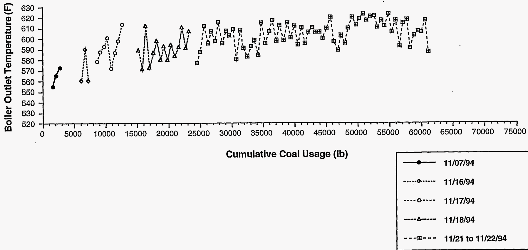
Figure 3-5. BOILER OUTLET TEMPERATURE AS A FUNCTION OF COAL CONSUMPTION WHEN FIRING AT 15.0 TO 16.4 MILLION BTU/H
