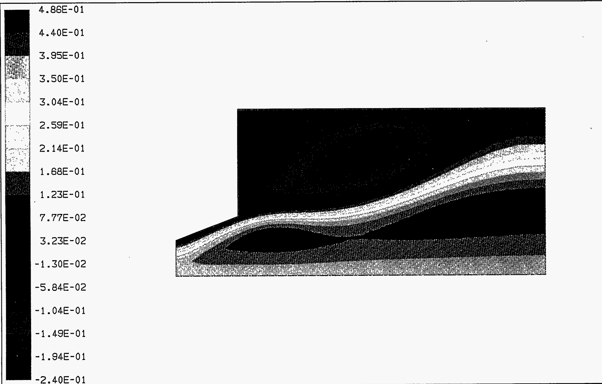
Figure 3-41. STREAM FUNCTION, IN SQUARE METERS/SECOND, IN THE DEMONSTRATION BOILER FOR A TURBULENCE INTENSITY OF 35%
