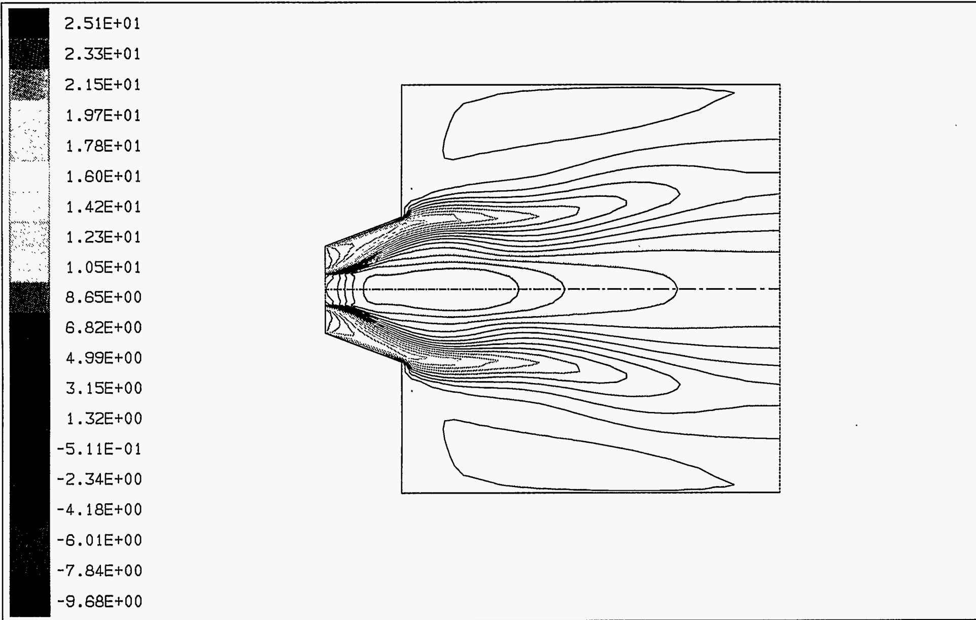
Figure 3-53. AXIAL VELOCITY CONTOURS, IN METERS/SECOND, UNDER FORCED VORTEX CONDITIONS
