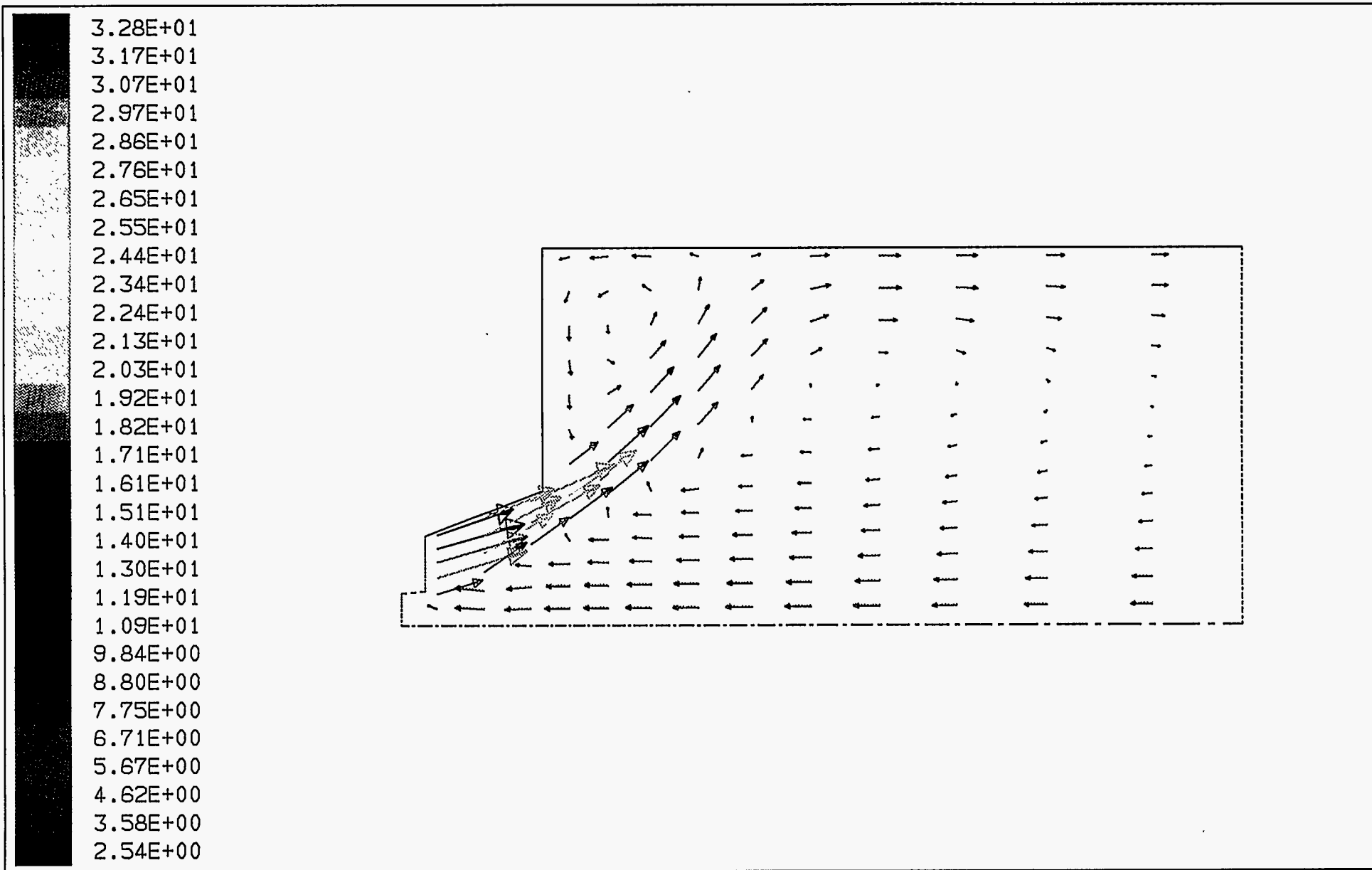
Figure 3-45. VELOCITY VECTORS, IN METERS/SECOND, FOR BURNER CONFIGURATION C
