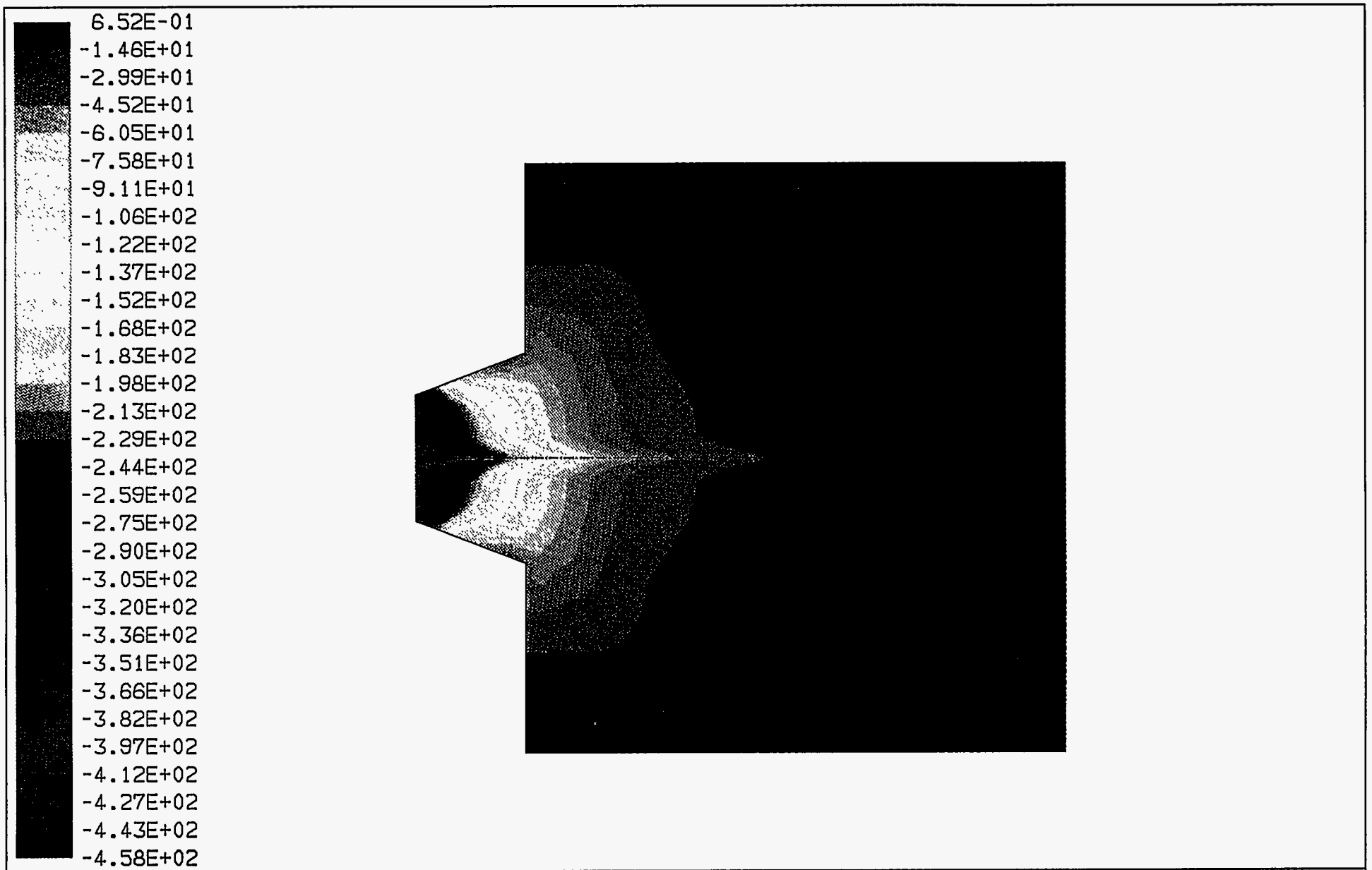
Figure 3-46. STATIC PRESSURE IN THE DEMONSTRATION BOILER WITH A SWIRL NUMBER OF ZERO
