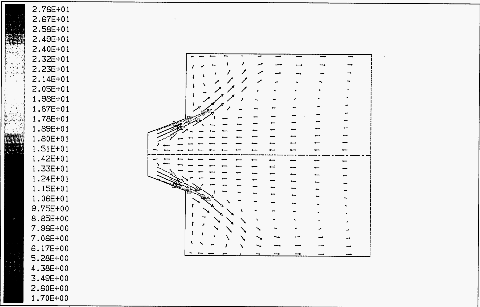
Figure 3-55. GAS VELOCITY VECTORS, IN METERS/SECOND, WITH COAL PARTICLE INJECTION
