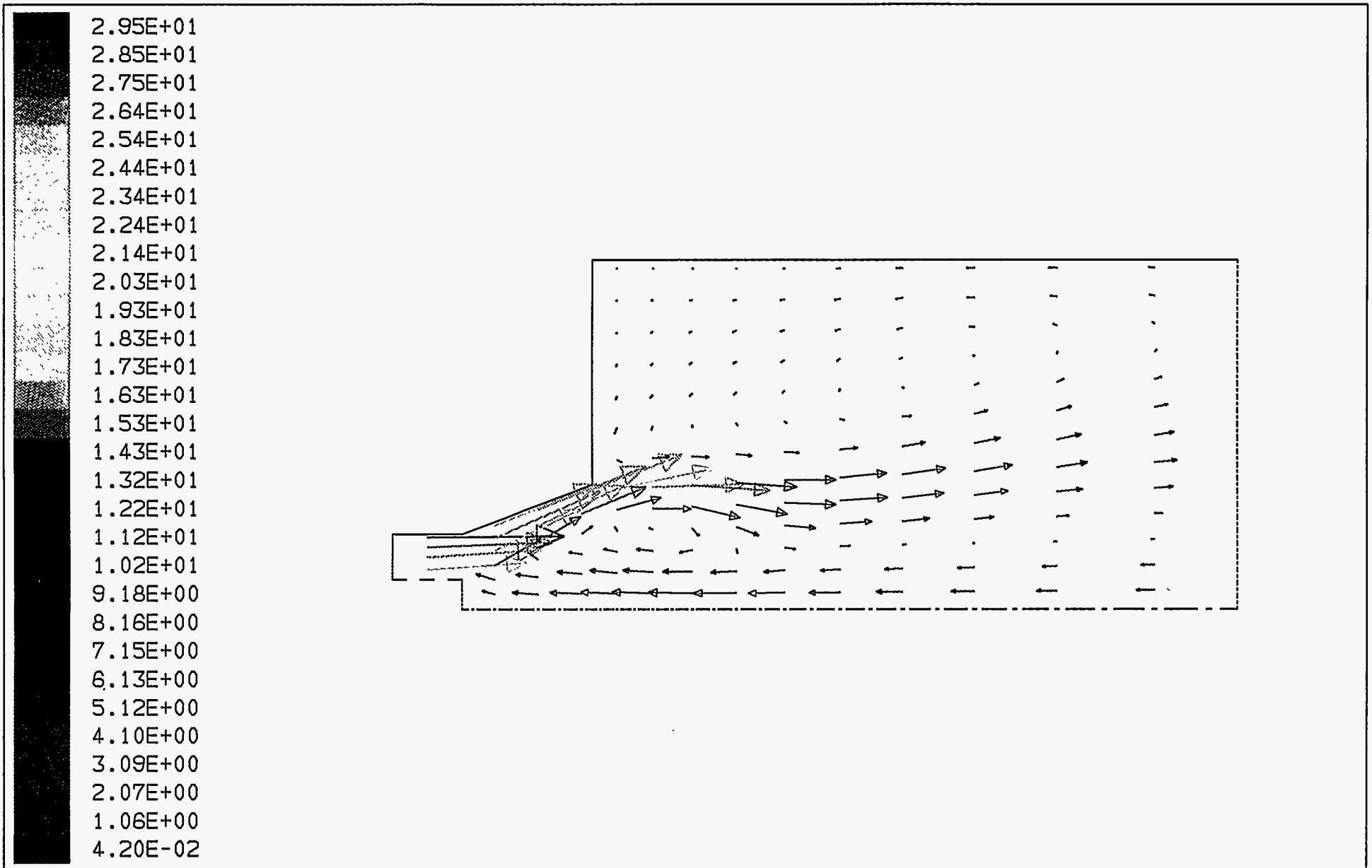
Figure 3-43. VELOCITY VECTORS, IN METERS/SECOND, FOR BURNER CONFIGURATION A
