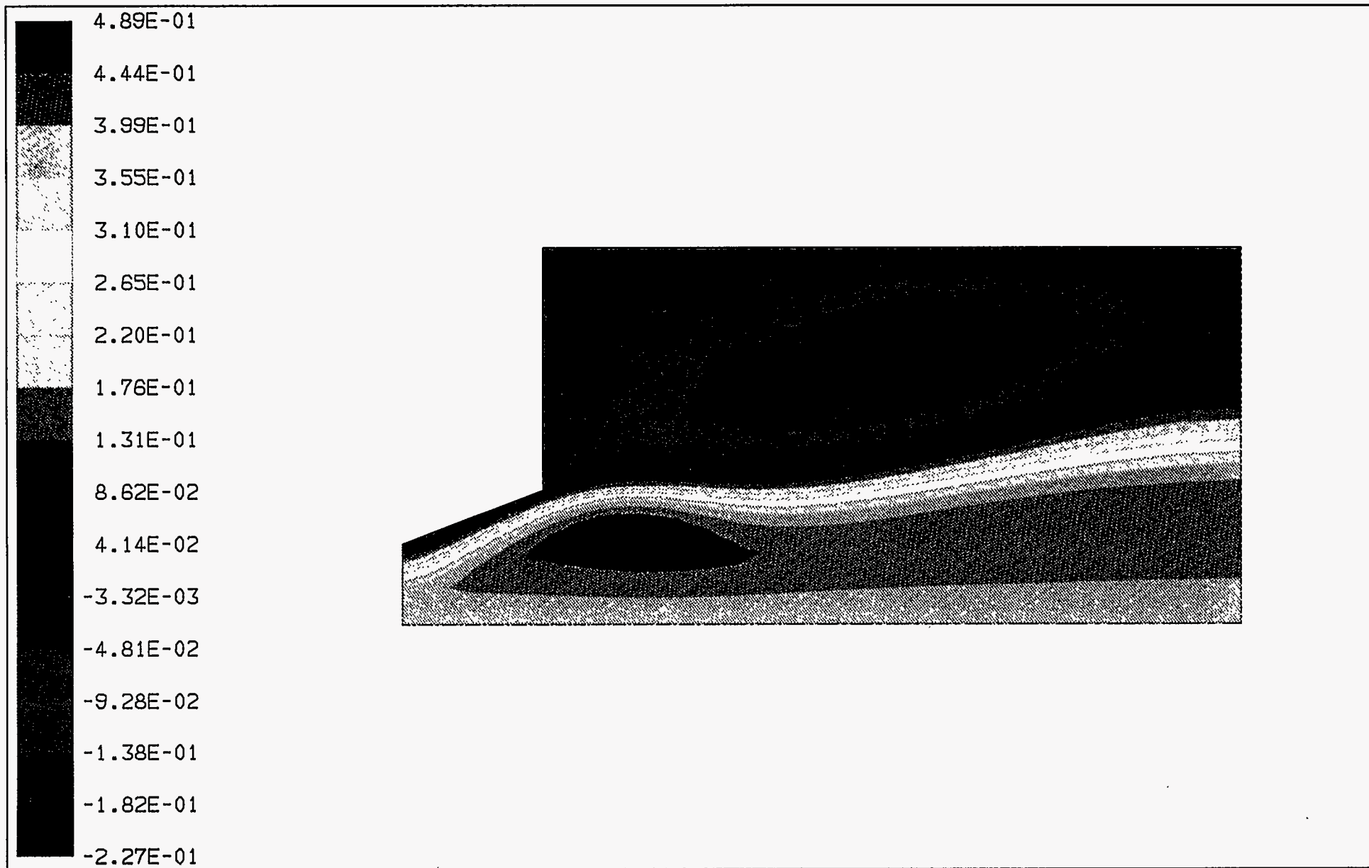
Figure 3-37. STREAM FUNCTION, IN SQUARE METERS/SECOND, IN THE DEMONSTRATION BOILER FOR A CHARACTERISTIC LENGTH OF 0.43 TIMES THE BURNER ANNULAR GAP
