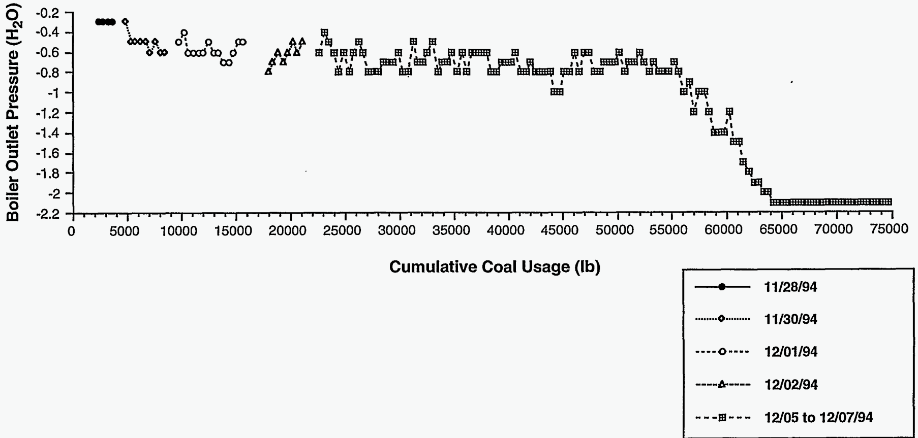
Figure 3-8. BOILER OUTLET PRESSURE AS A FUNCTION OF COAL CONSUMPTION WHEN FIRING AT 12.7 TO 12.8 MILLION BTU/H
