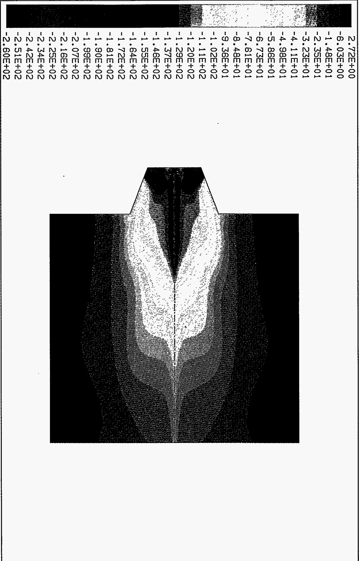
Figure 3-47. STATIC PRESSURE IN THE DEMONSTRATION BOILER WITH A SWIRL NUMBER OF 0.6
