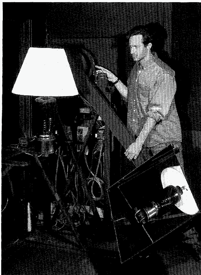
Figure 6. Researcher checks the alignment of LBL's recently completed mirror-based goniophotometer. A goniophotometer is used to measure the angular distribution of light (candlepower) emanating from a lighting fixture.
