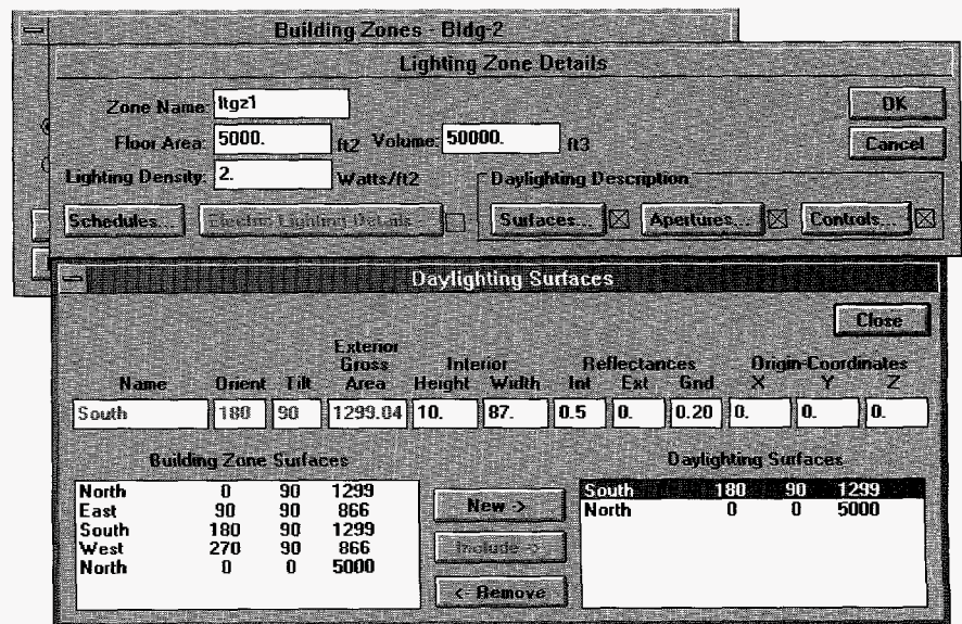
Figure 3. Prototype user interface for describing a daylighting system.
