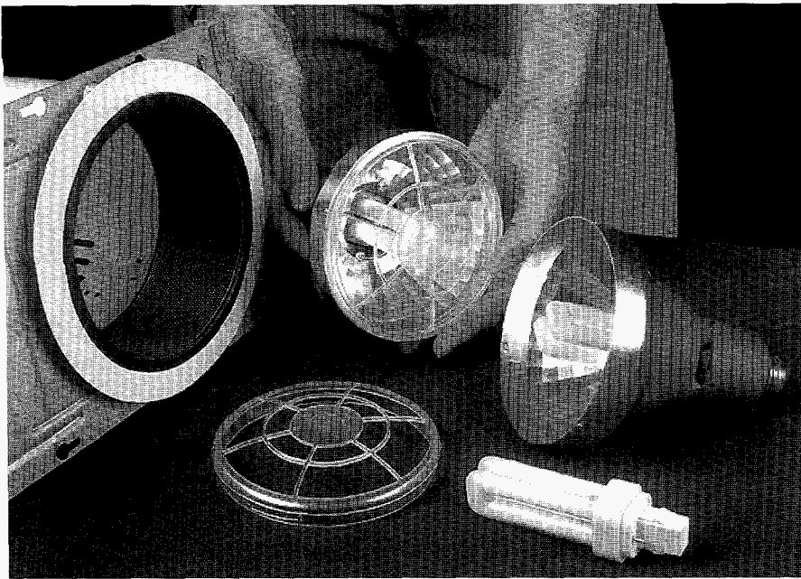
Figure 7. An improved compact fluorescent lamp fixture recently patented by LBL and licensed to the Lumatech Corporation. The fixture contains vents in the reflector that prevent hot air from being trapped in the fixture and a specially designed lens that allows airflow while reducing glare.
