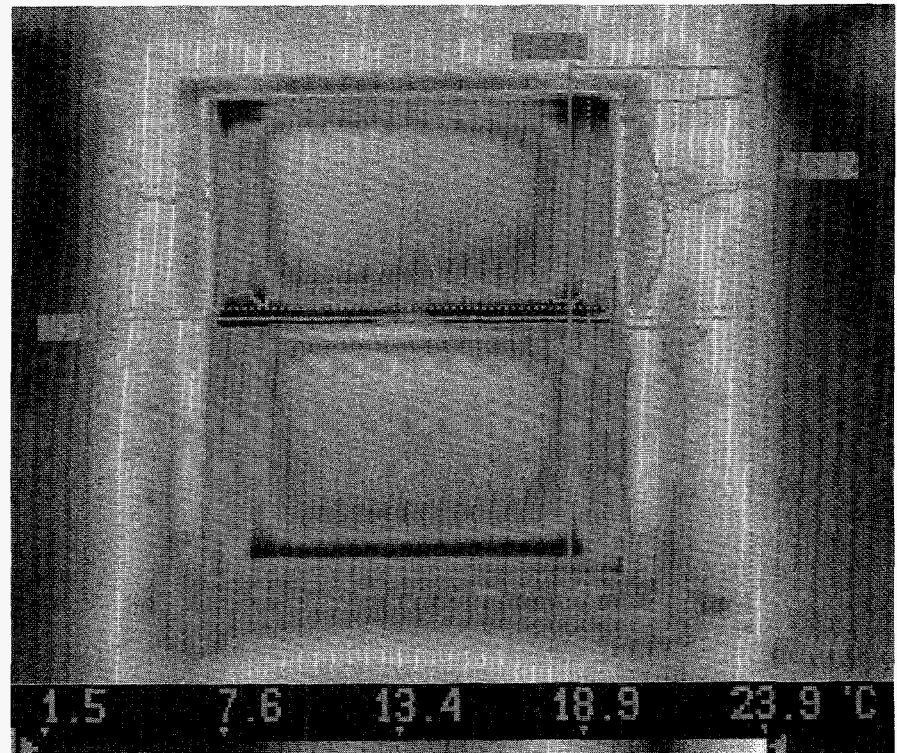
Figure 2. Infrared image shows the warm side of a standard 2 × 4 wall with an energy-efficient double-hung window in the center. While the wall and center-of-glass areas are at constant warm temperatures (shown by red or yellow-red), other surfaces are colder (shown by blue, green, and violet), indicating thermal bridging through window frame and window framing materials. Current research focuses on the development of integrated window/wall systems which minimize two-dimensional framing effects and contain recessed night insulation and exterior summer shading devices.
