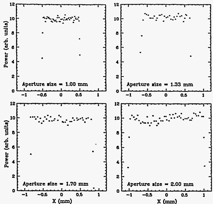
Figure 1. Profiles of the laser beam spot as viewed on a CCD camera. The plots are cuts through the center of the laser beam image for each of the four apertures.
