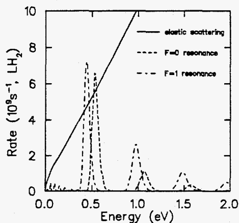
Figure 1: Predicted resonance structure of \mu t + D_2 at 3 K and density of liquid hydrogen[11], compared with rate of energy loss, for two hyperfine states of \mu t .
