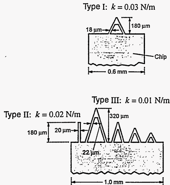
Figure 5. Schematic view of the 0.6 \mu\text{m} thick \text{Si}_3\text{N}_4 microcantilevers used for evaluation of thermal response. Note that results from only the two left-most microcantilevers (out of five total) on the lower chip are presented.
