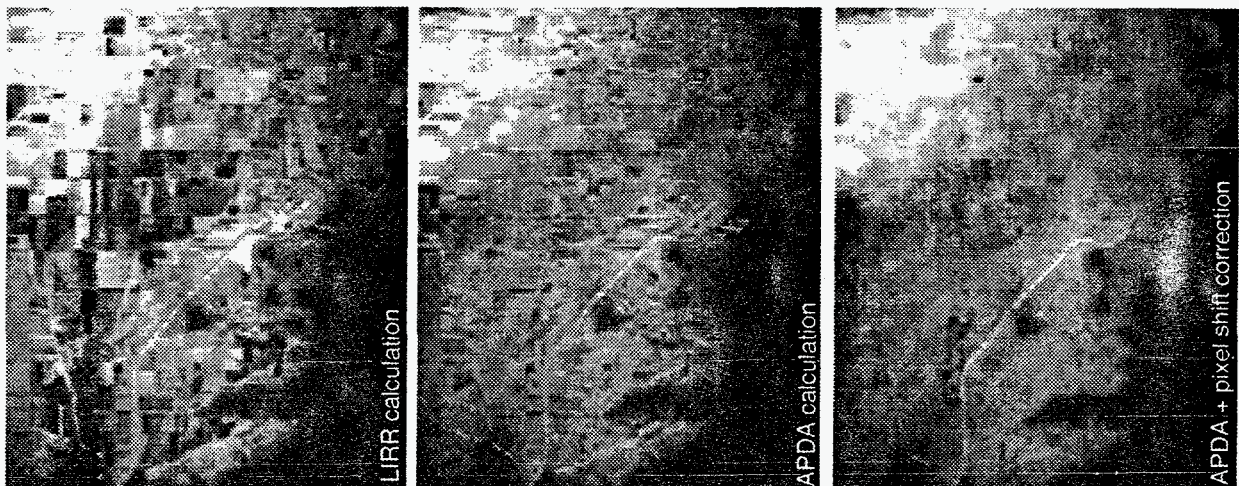
Figure 3: LIRR(61,62;55,56,68,69) calculation over the 1995 AVIRIS scene at Camarillo (near Oxnard, CA). Left: raw calculation; middle: only atmospheric pre-correction applied; right: path radiance and pixel shift correction combined. All images are smoothed with a filter size of 5x5 Pixels. The water vapor total column ranges between 17.5 \text{kg}/\text{m}^2 (dark areas) and 19.5 \text{kg}/\text{m}^2 (white areas), the mountain area appears black. The images are enhanced to show variations over the plain between Camarillo (northern image border) and Point Mugu (south); see also slide in the appendix.
