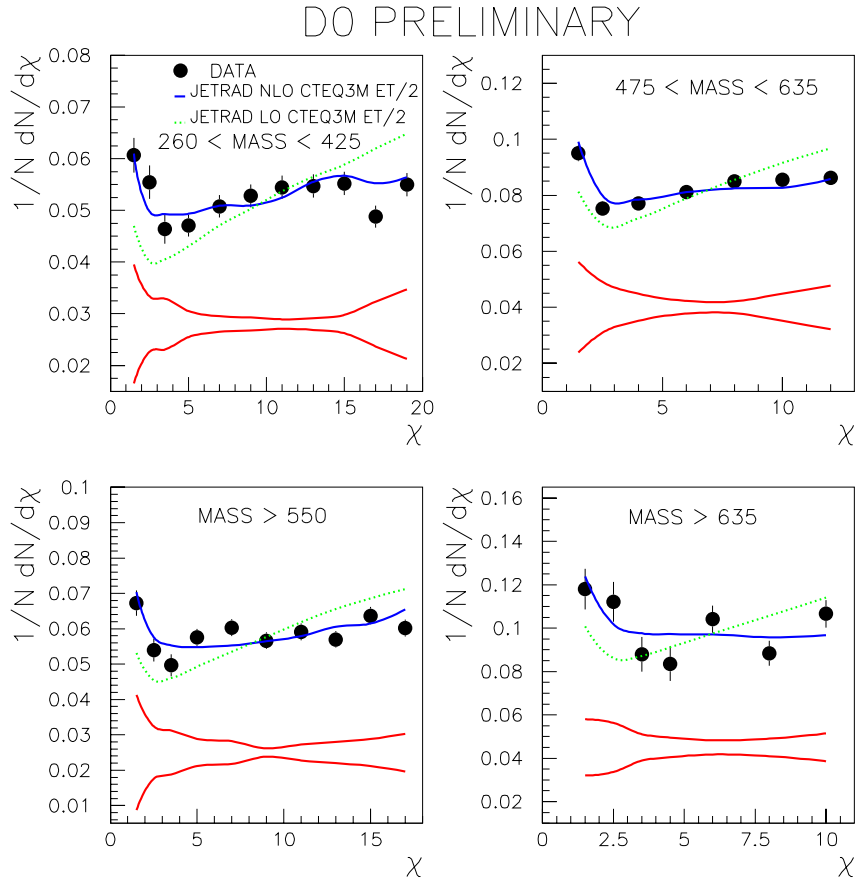
FIG. 5. Comparisons of data to NLO and LO predictions of QCD using JETRAD with CTEQ3M and a renormalization scale of E_T/2 . The errors bars are statistical. Shown at the bottom of each plot is the plus and minus 1\sigma systematic error band.
