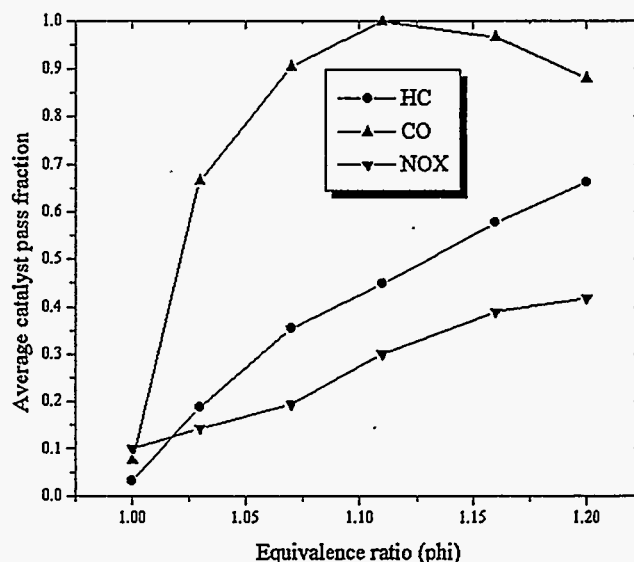
Figure A.6. Average catalyst pass fraction vs equivalence ratio for cars in the FTP-RP
