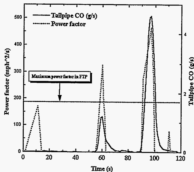
Figure A.8. CO emissions in three high-power episodes
