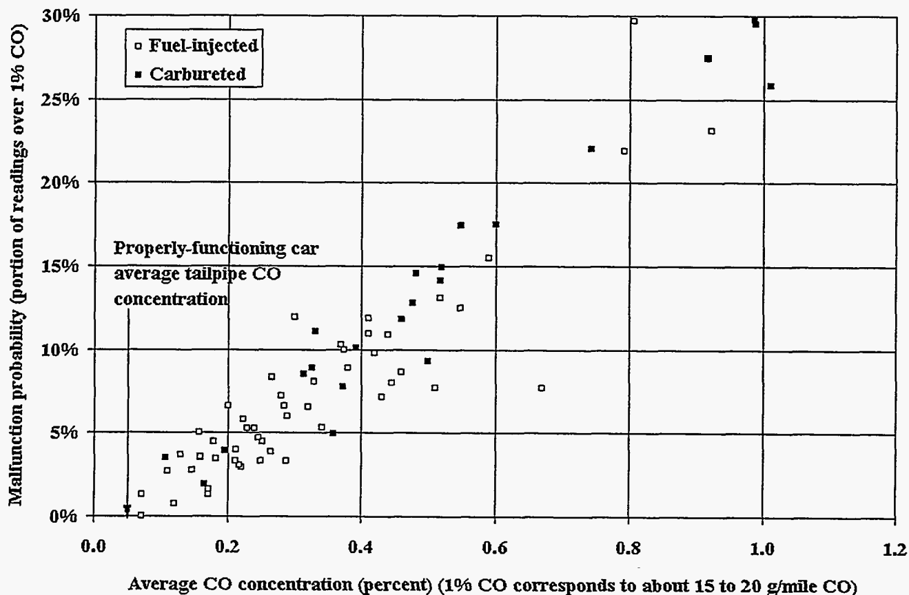
Figure B.3. Malfunction probability vs average CO concentration, 76 MY87-89 models with over 50 different vehicles observed in the 1991 CARB Remote Sensing Data
