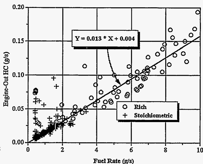
Figure A.3. Engine-out HC vs fuel rate for a sample MY93 car
