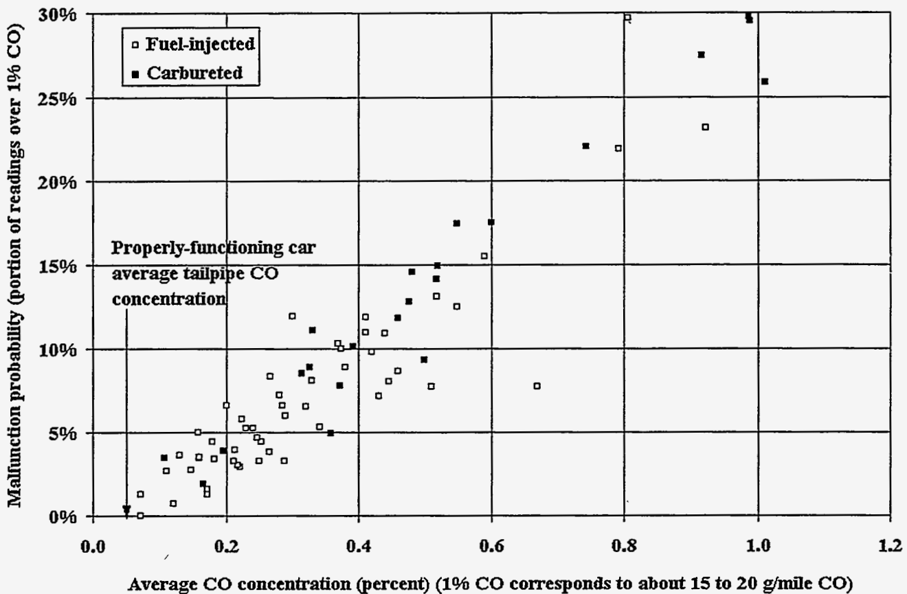
Figure 5.1. Malfunction probability vs average CO concentration, 76 MY87-89 models with over 50 different vehicles observed in the 1991 CARB Remote Sensing Data
