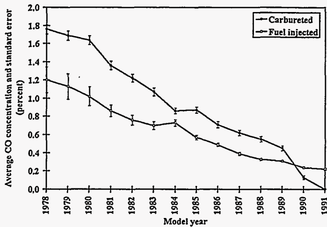
Figure A.12. Average CO emissions, by MY and fuel system and Figure A.13. Average CO emissions by MY and exhaust air injection
