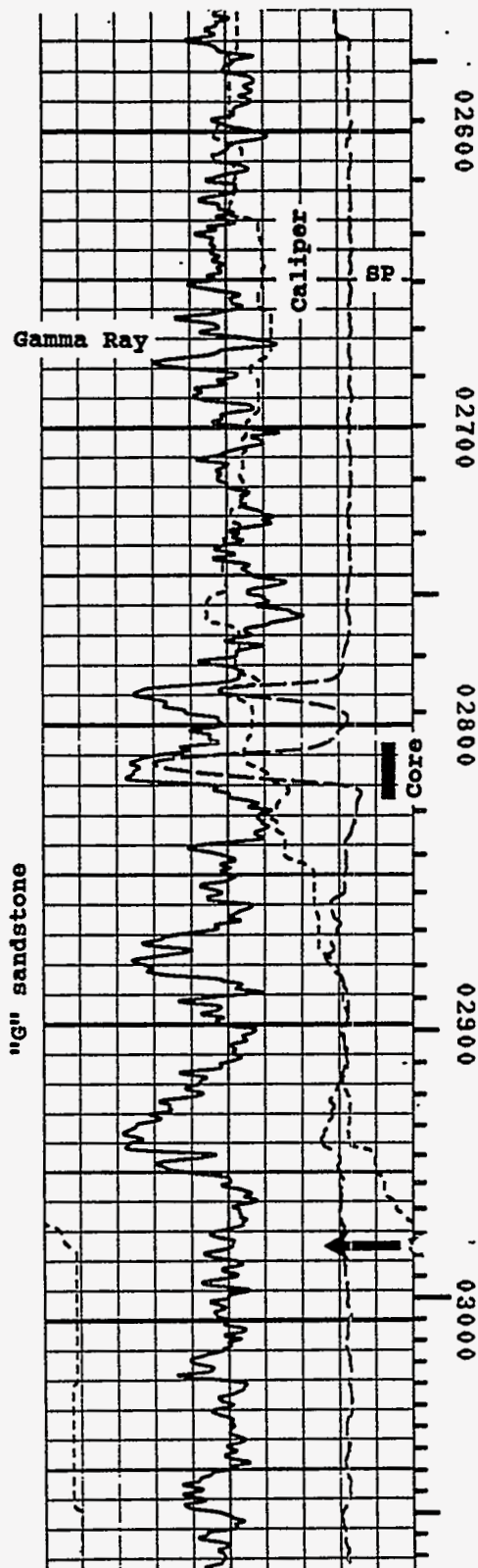
Figure 8. Geophysical log showing the location of the SSP core within the sandier "G" interval of the Wasatch Formation.
