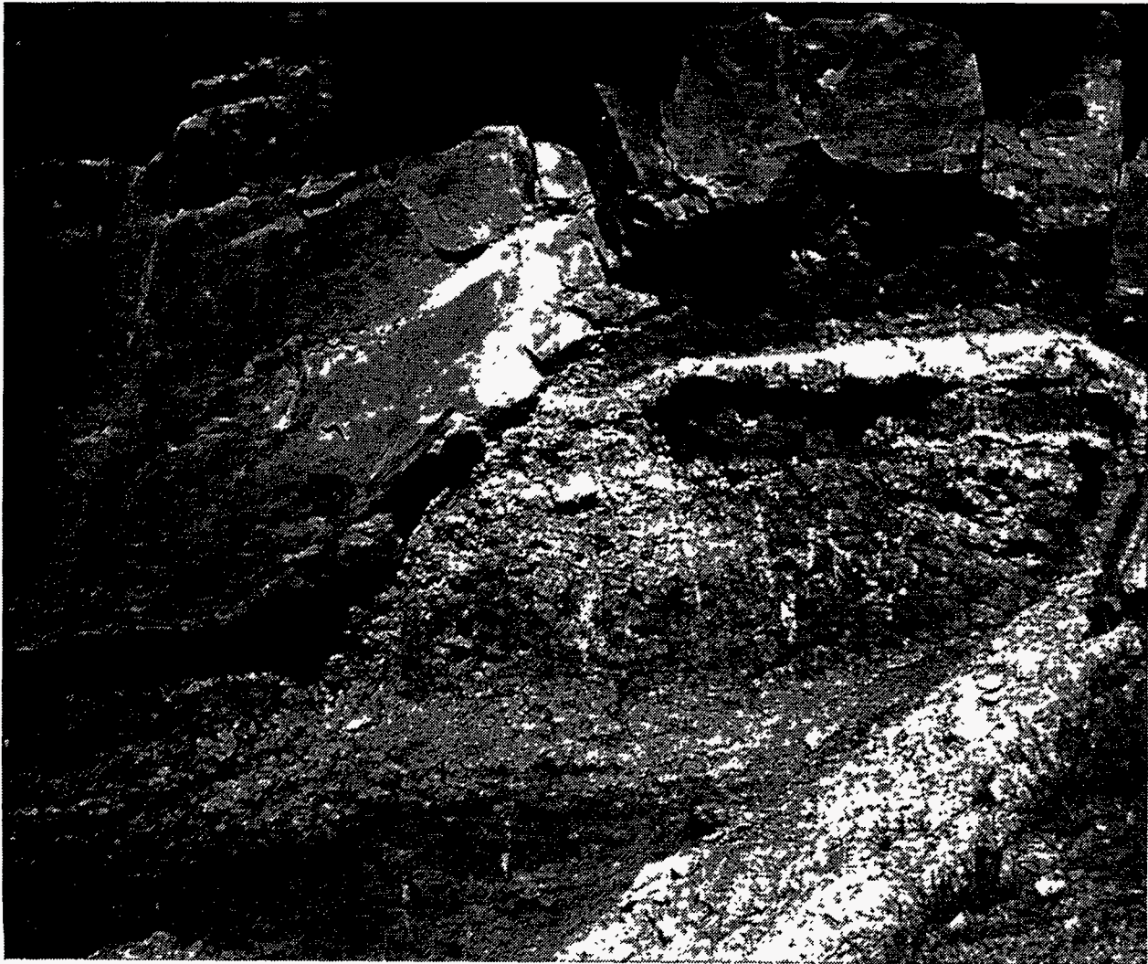
Figure 5a. Fluvial channel that cut down into a soil horizon. Note the anticlinal forms in the mudstones, indicative of vertisols, under the "wing" of the channel sandstone. Sandstone is about three meters thick at the left edge.
