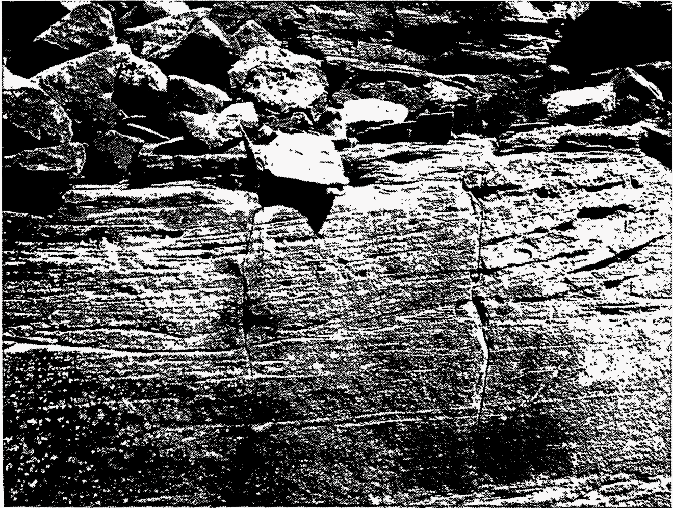
Figure 3c. Trough crossbed nested within planar-horizontally bedded sandstone, near the type section of the Molina Member.
