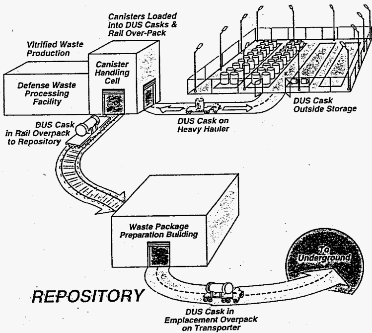
Figure 2. DU-Shielded Cask Scenario
