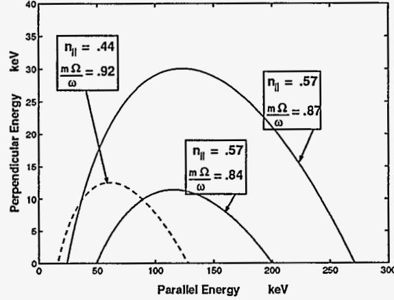
Figure 3: Solid lines illustrate the change in the resonance curve due to a change in the ratio \frac{m\Omega_{ce}}{\omega} at a constant n_{\parallel} . The dotted line illustrates the change in the resonance curve due to a change in the viewing angle ( n_{\parallel} ).
