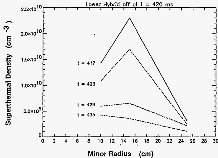
Figure 8: Radial profile of the superthermal density measured by the Oblique ECE system. The dotted lines show the time evolution of the density profile after the Lower Hybrid power is turned off at 420 ms.
