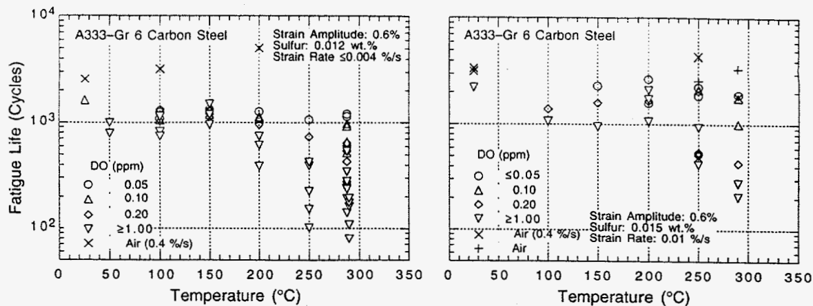
Figure 5—Change in fatigue life of A333-Gr 6 carbon steel with temperature and DO
