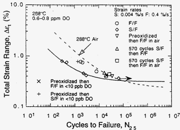
Figure 14— Environmental effects on formation of surface microcracks. Preoxidized specimens were exposed at 288°C for 30–100 h in water with 0.6–0.8 ppm DO.
