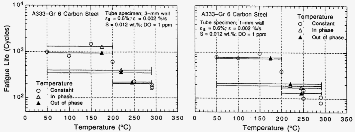
Figure 13—Effect of varying temperature on fatigue life of A333-Gr 6 carbon steel
