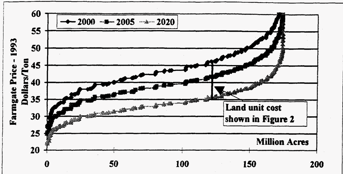
Figure 3: Potential Switchgrass Supply for the North Central Region
