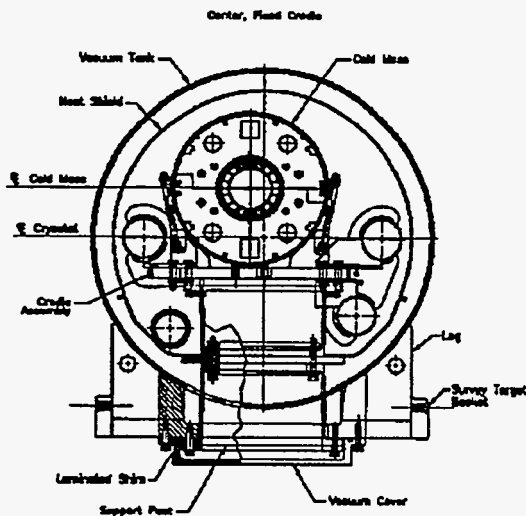
Figure 2. Arc dipole with cryostat cross section.
