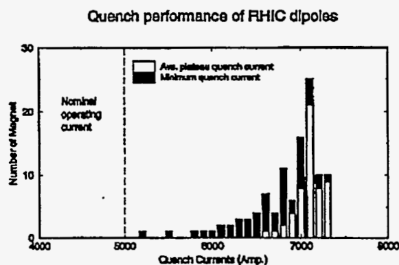
Figure 6. Dipole magnet quench current distributions.
