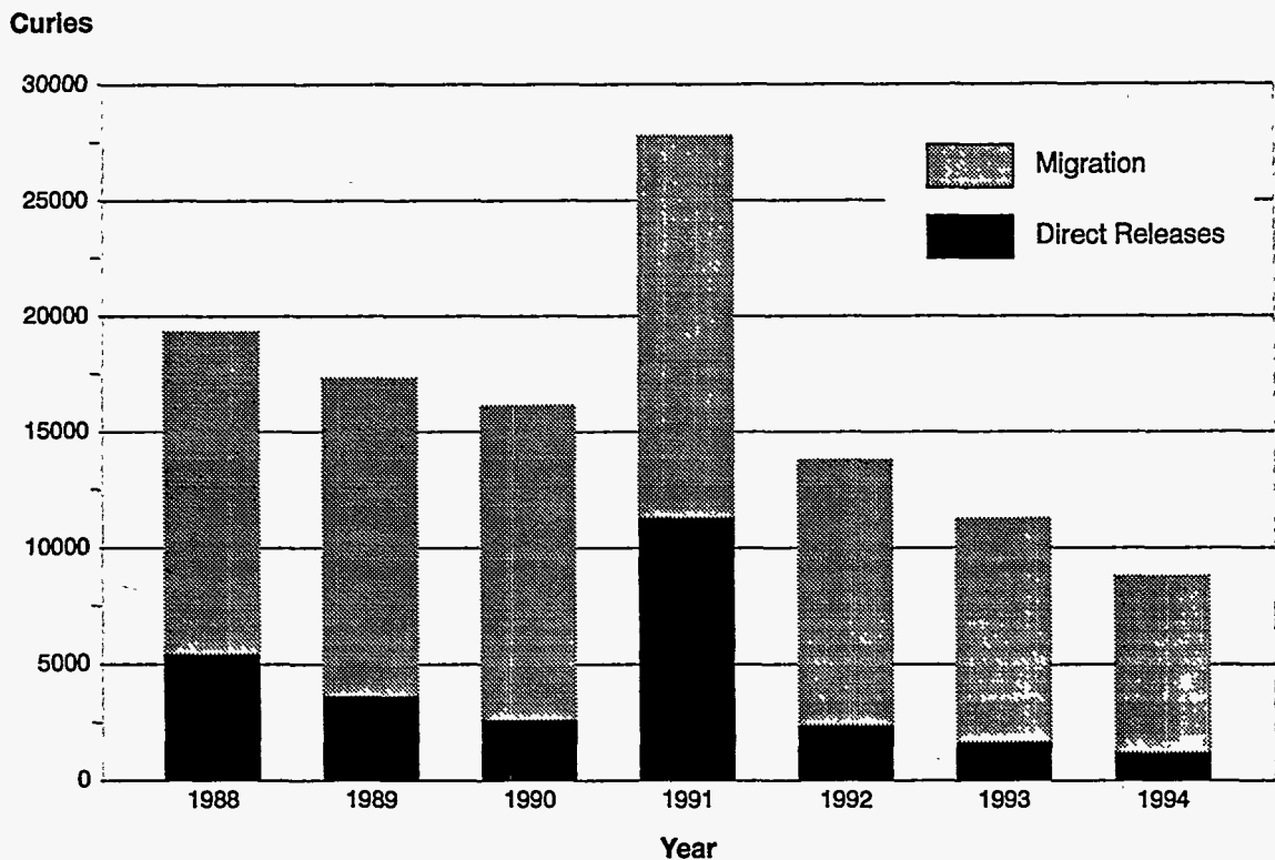
Figure 5-4 Total Tritium Releases to SRS Streams (Direct Discharges and Migration), 1988-1994
