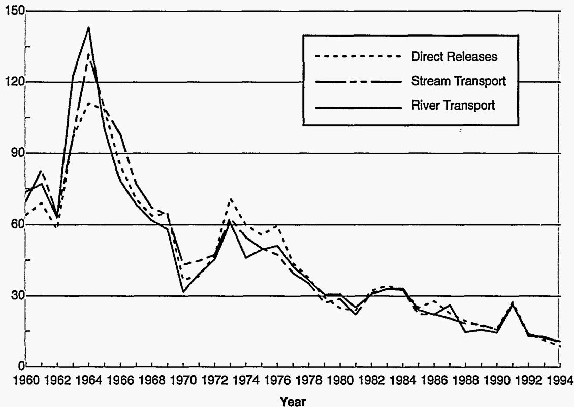
Figure 6-7 SRS Tritium Transport Summary, 1960-1994
