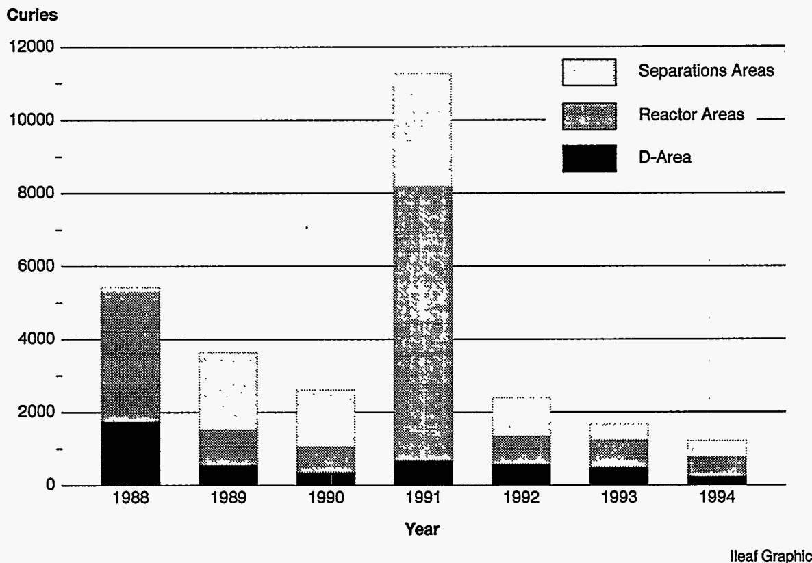
Figure 5-2 Direct Releases of Tritium to SRS Streams, 1988-1994
