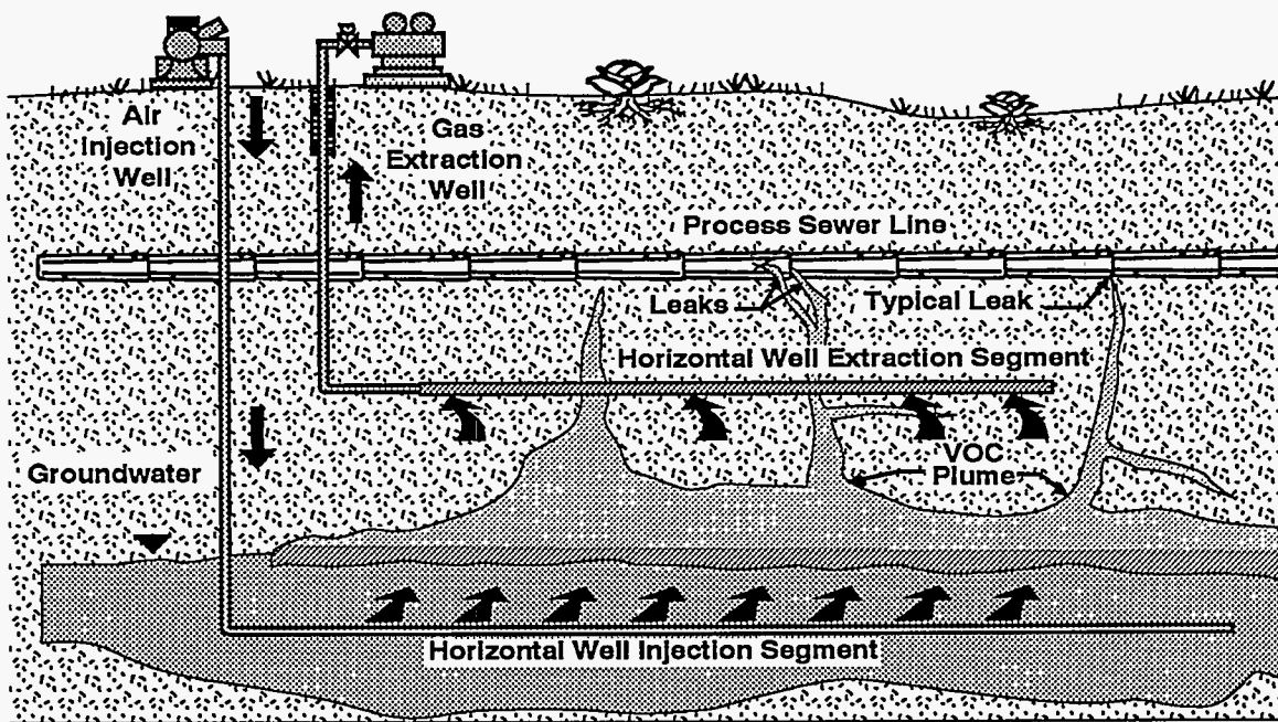
Figure 10-2 Horizontal Wells
