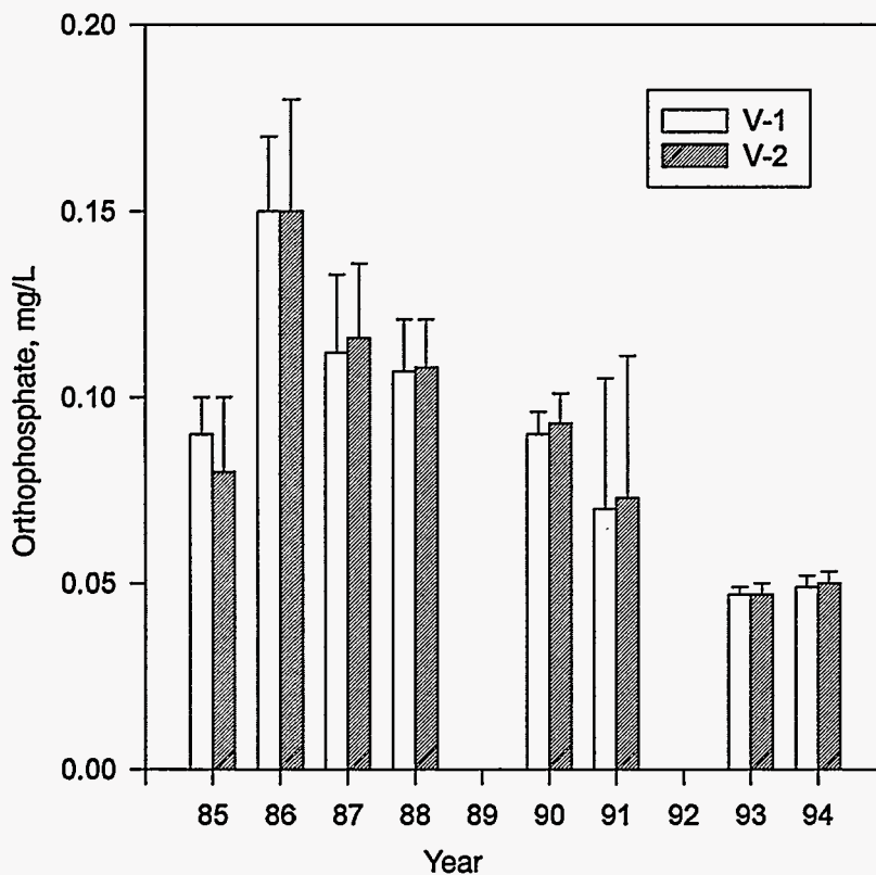
Figure 12-8 Orthophosphate Concentrations
