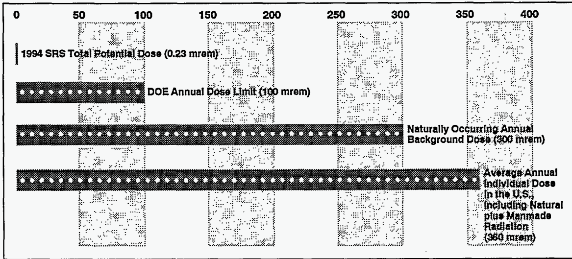
Figure 2 Comparison of Doses from SRS to Background and Federal Standards
