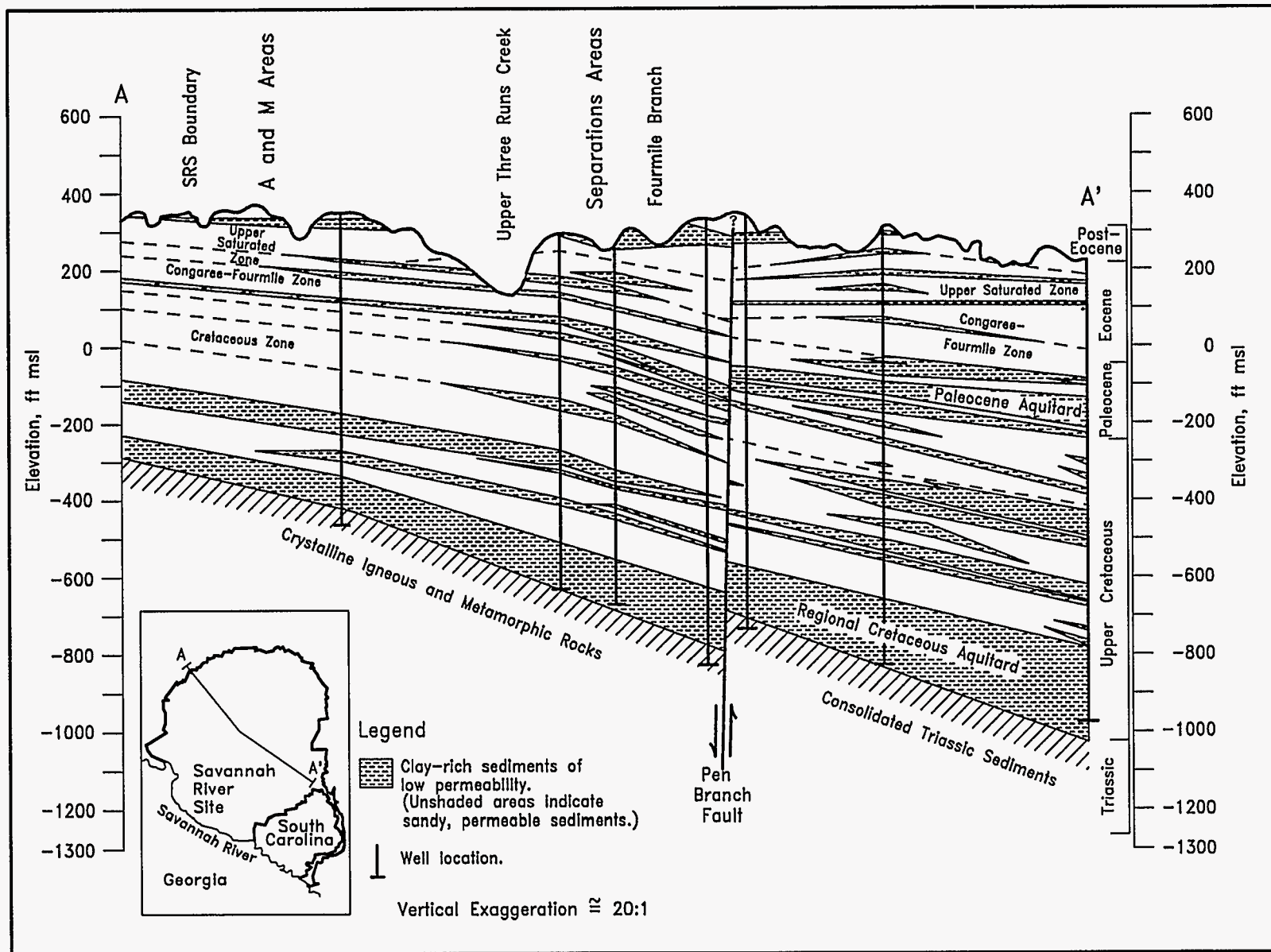
Figure 10-5 Geologic Cross Section of Coastal Plain Sediments at SRS
