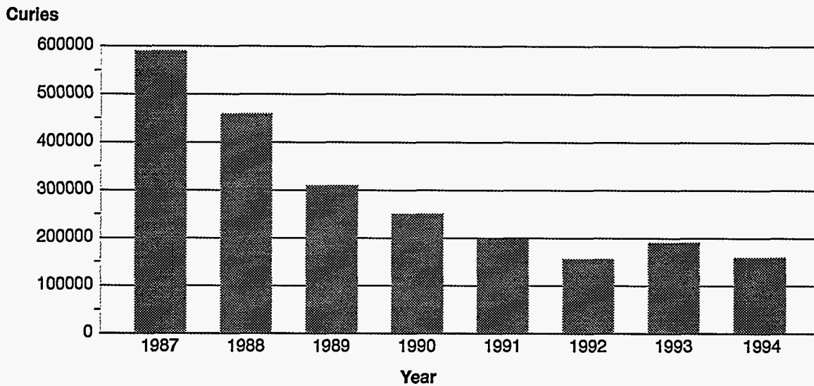
Figure 5-1 SRS Annual Atmospheric Tritium Releases, 1987-1994
