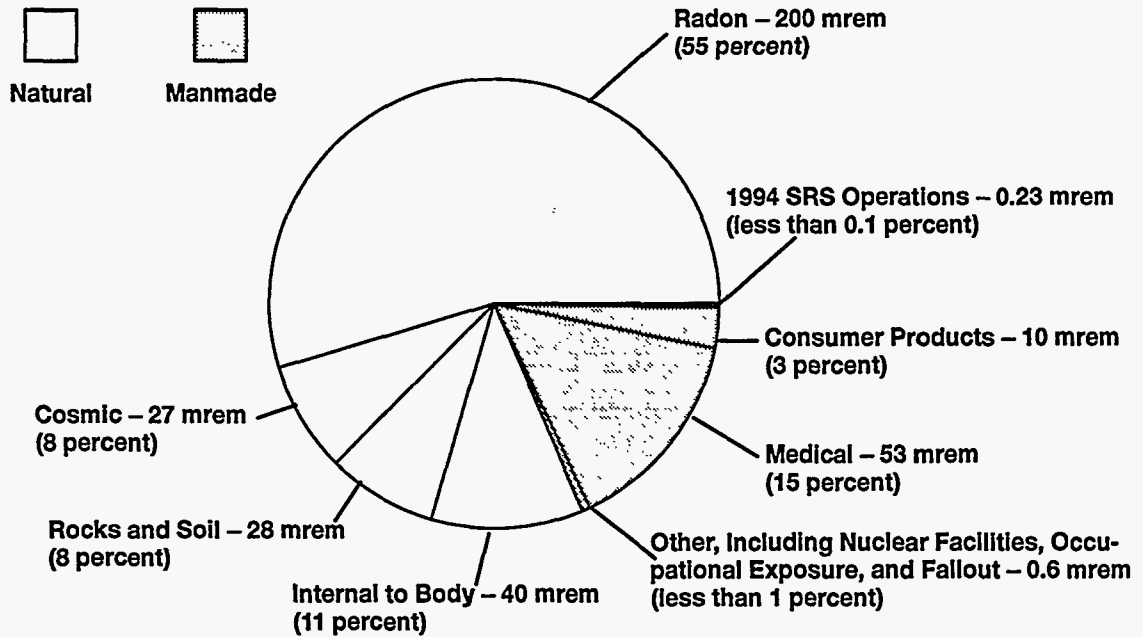
Figure 3 Contributions to the Average Individual Dose
