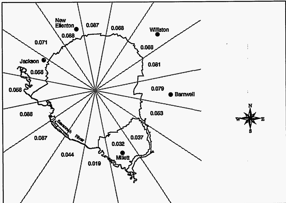
Figure 7-4 Sector-Specific Adult Maximally Exposed Individual Dose (mrem)
