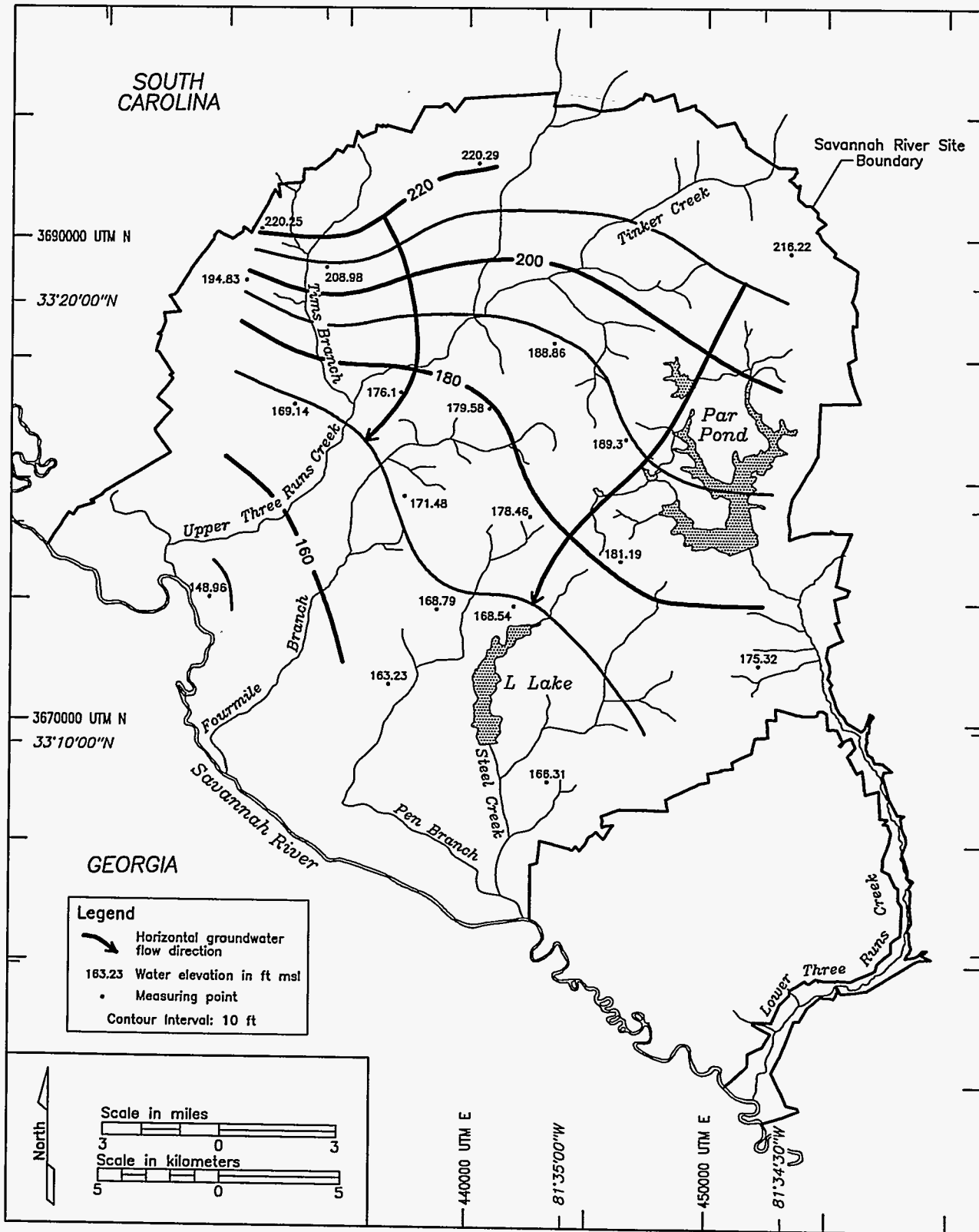
Figure 10-4 Potentiometric Surface and Horizontal Groundwater Flow Directions of the Cretaceous Zone at SRS During the First Quarter of 1994
