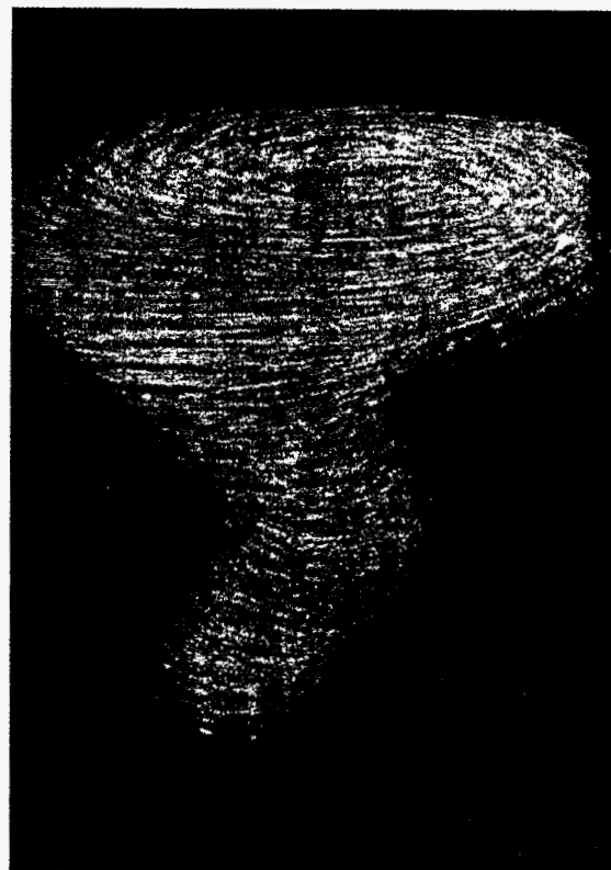
Figure 5-3 HSV Jittering = (0.3, 0.3, 0.3)
