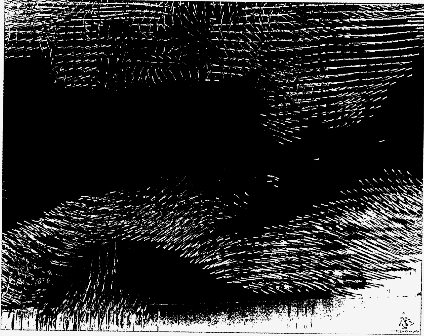
Figure 7-4 Hairs used to represent two time steps of the winds over Indonesia.
