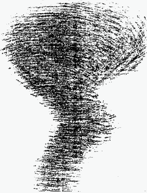
Figure 5-28 Opacity = 0.1
