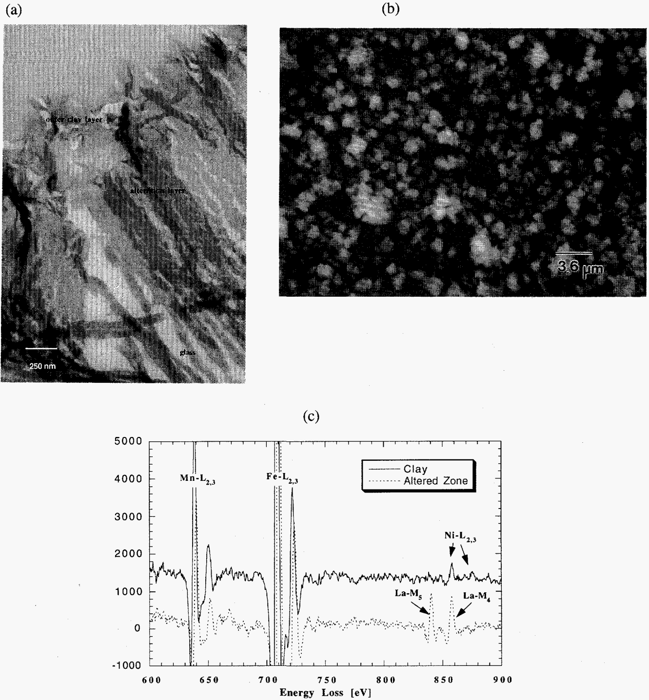
Fig. 21. (a) AEM Cross-Sectional View of Sample Reacted for 28 Days, (b) an SEM Image of Glass Reacted at 70°C in a Vapor Environment for 91 Days, and (c) Analysis of Iron, Manganese, and Lanthanum in the Clay Layer and Altered Zone Shown in (a) Using AEM/Electron Energy Loss Spectroscopy
