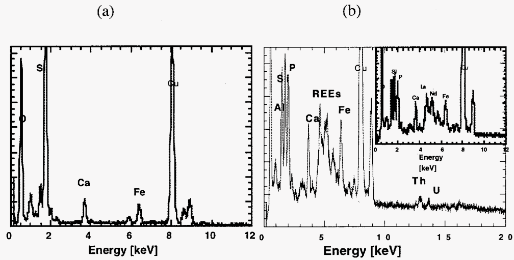
Fig. 54. (a) EDS Analysis of Clay Material from 200R Drip Test and (b) EDS Analysis of Rare Earth-Bearing Phase, Which Also Contains Trace Thorium and Uranium
