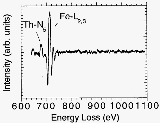
Fig. 34. (a) AEM Micrograph of Thorium-Iron-Titanium Precipitates under a Layer of Clay from the N3-5 Glass Monolith. The clay had pulled away from the glass in this region of the sample, but the glass was originally located on the side of the clay containing the precipitates. The EELS spectra (b, c) reveal that the precipitates do not contain rare earth elements (compare Fig. 32).
