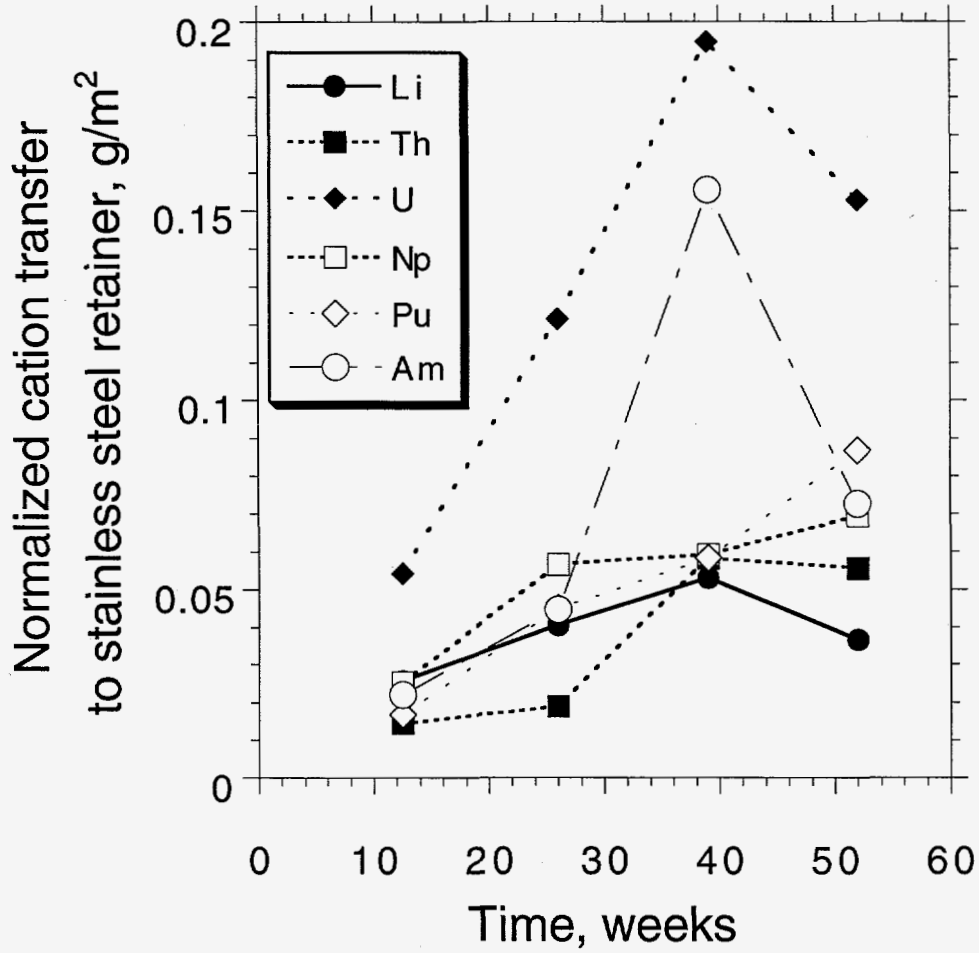
Fig. 36. Cations from the Acid Strip of the Waste Form Supports as Measured by ICP-MS. These values are normalized to the concentrations of each element present in the original ATM-10 glass and are divided by the surface area of the monolith.
