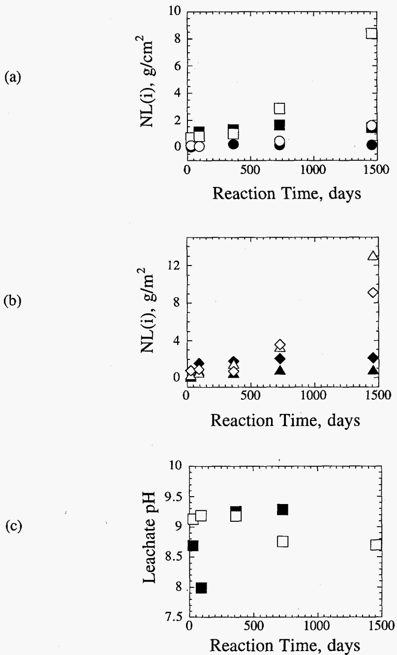
Fig. 9. Normalized Mass Losses of (a) Li (■ and □) and Si (● and ○) and (b) B (▲ and △) and Na (◆ and ◇) from SRL 131/11 Glasses Reacted in Static Tests at 90°C and 340 m -1 . In (c) the solution pH is shown. The filled symbols represent the results of tests with the fully radioactive glass; the open symbols represent the results of tests with the simulated glass.
