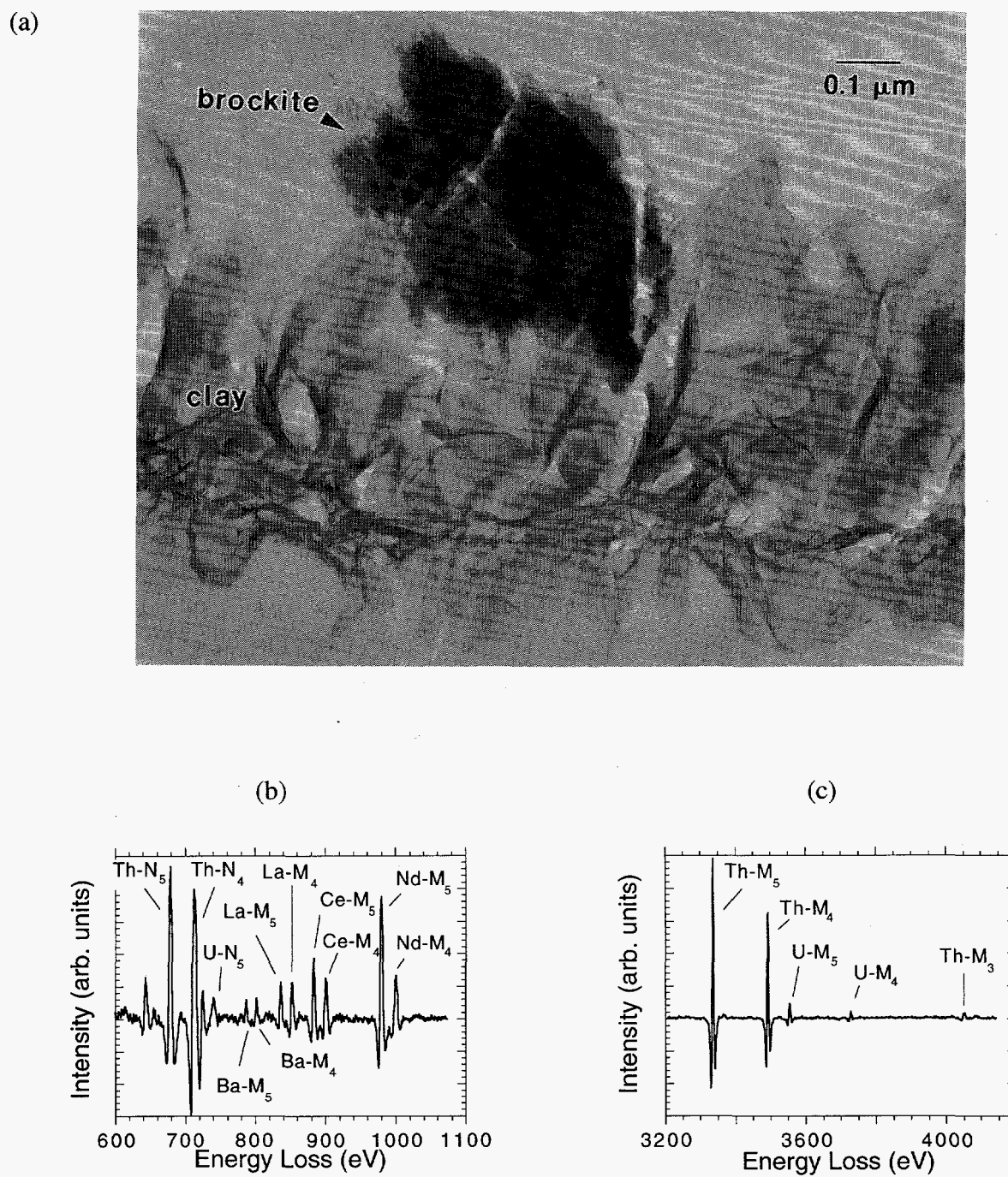
Fig. 32. (a) AEM Micrograph of a Brockite Particle Attached to Clay from the Top Surface of the N3-5 Glass. The clay has separated from the glass in this region, which is not visible in the micrograph; it was originally located on the side of the clay opposite the brockite. (b,c) EELS spectra of the rare earth and actinide elements in the brockite.
