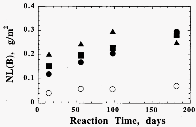
Fig. 12. Normalized Mass Loss for PCT Tests with 51S Glass in EJ-13 at (a) 2000 \text{ m}^{-1} and (b) 20,000 \text{ m}^{-1} Based on B (●), Li (■), Na (▲), and Si (○). Results are the average of duplicate tests.
