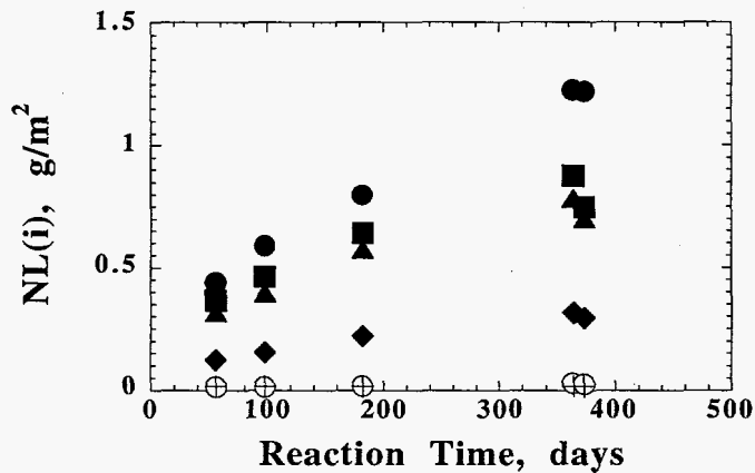
Fig. 17. Normalized Mass Loss from Static Tests with WV6 Glass at (a) 2000 \text{ m}^{-1} , (b) 20,000 \text{ m}^{-1} with -100+200 Mesh Glass, and (c) 20,000 \text{ m}^{-1} with -200+325 Mesh Glass: B (●), Li (■), Na (▲), K (◆), Si (○), and U (+).
