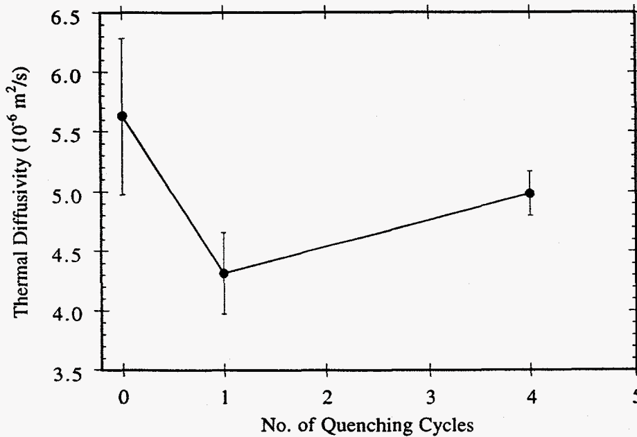
FIG. 3--Effect of number of quench cycles (@ \Delta T = 800^\circ\text{C} ) on thermal diffusivity of 2-D weave Nicalon/CVI SiC CFCC.
