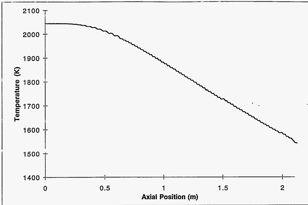
Figure 2. Axial centerline temperature profile
