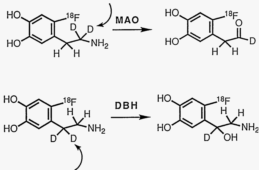
Figure 6. Specifically deuterated 6-[ 18 F]FDA derivatives for probing MAO and DBH.
