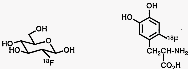
6-[ 18 F]fluoro-DOPA (dopamine metabolism)
