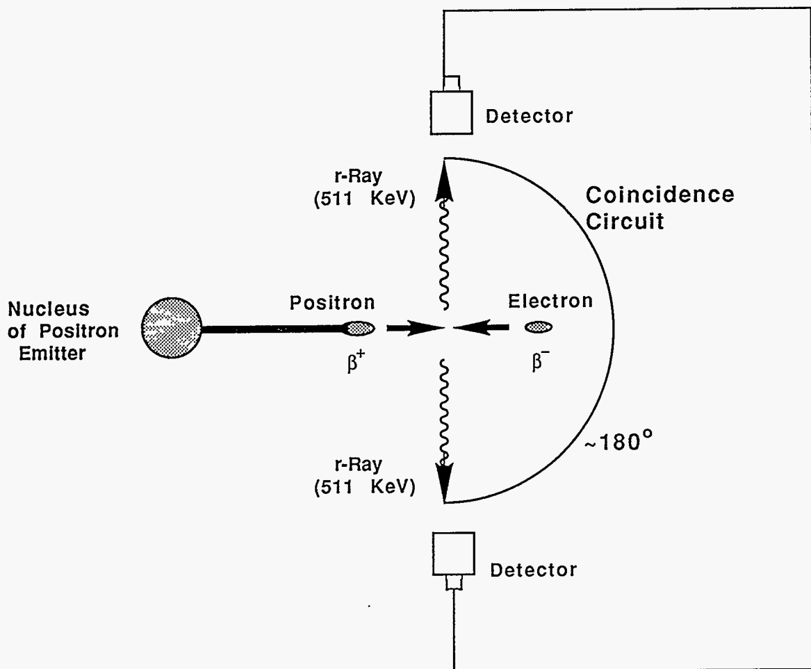
Figure 1 Diagram showing decay of positron emitter. The positron annihilates with an electron generating two 511 KeV r-rays at ca. 180° which penetrate the body barrier and are detected by coincidence detection.
