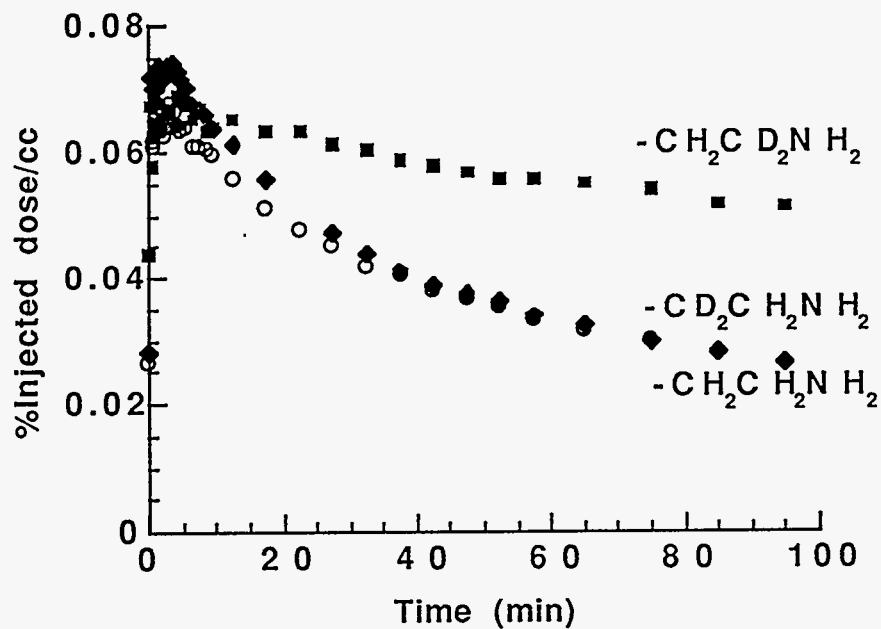
Figure 7. Uptake and clearance of 18 F after injection of 6-[ 18 F]FDA (open circles) and 6-[ 18 F]FDA-α,α-D 2 (squares), and 6-[ 18 F]FDA-β,β-D 2 (diamonds) in baboon heart.
