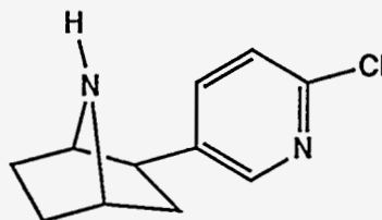
(±) Epibatidine (nicotinic receptor agonist)
