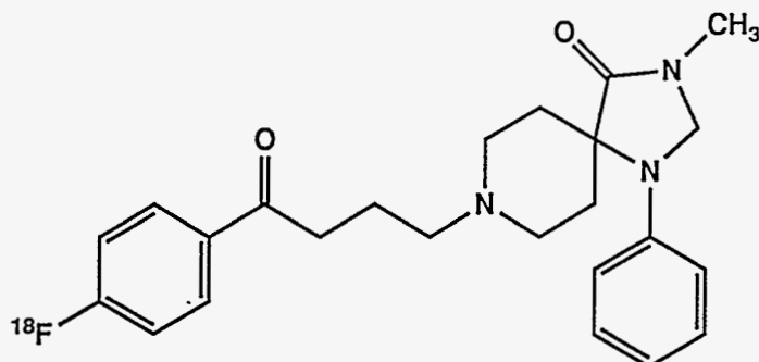
[ 18 F]N-methylspiroperidol (dopamine D 2 ligand)
