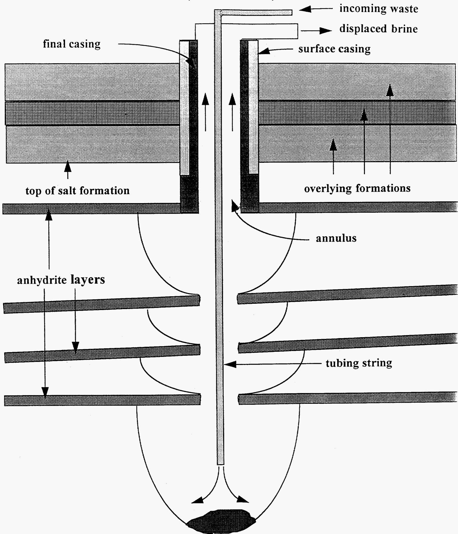
Figure 7 - Idealized Cavern in a Bedded Salt Formation (not to scale)
