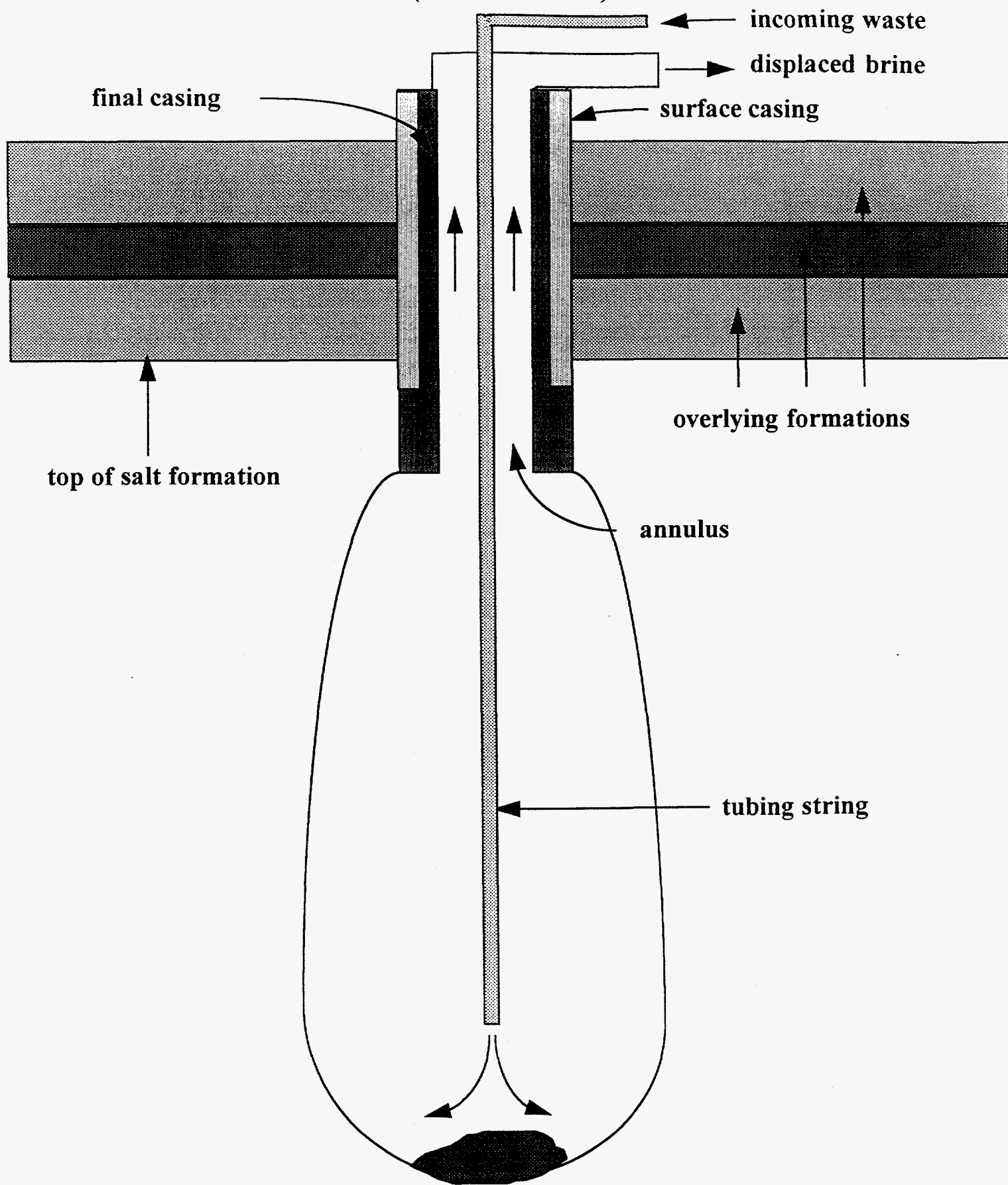
Figure 6 - Idealized Cavern in a Salt Dome Formation (not to scale)
