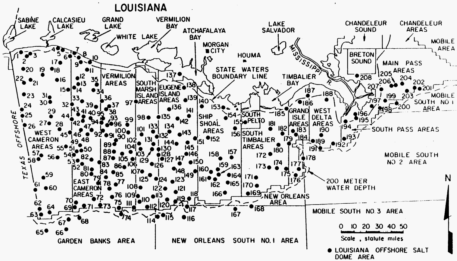
Figure 3 - Location of Louisiana Offshore Salt Domes (from Jirik and Weaver 1976)
