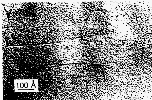
Fig. 9. Transmission electron microscopy (TEM) plan-view lattice image of a typical diamond nanocrystallite deposited from a \text{C}_{60}/\text{Ar} microwave discharge.
