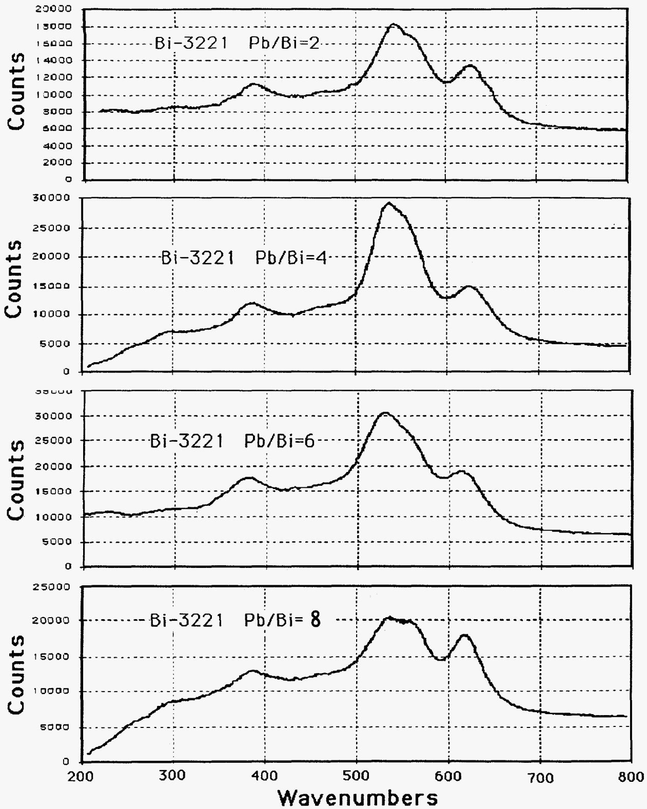
Figure 4. Raman spectra of four "3221" compositions as indicated in the figure.
