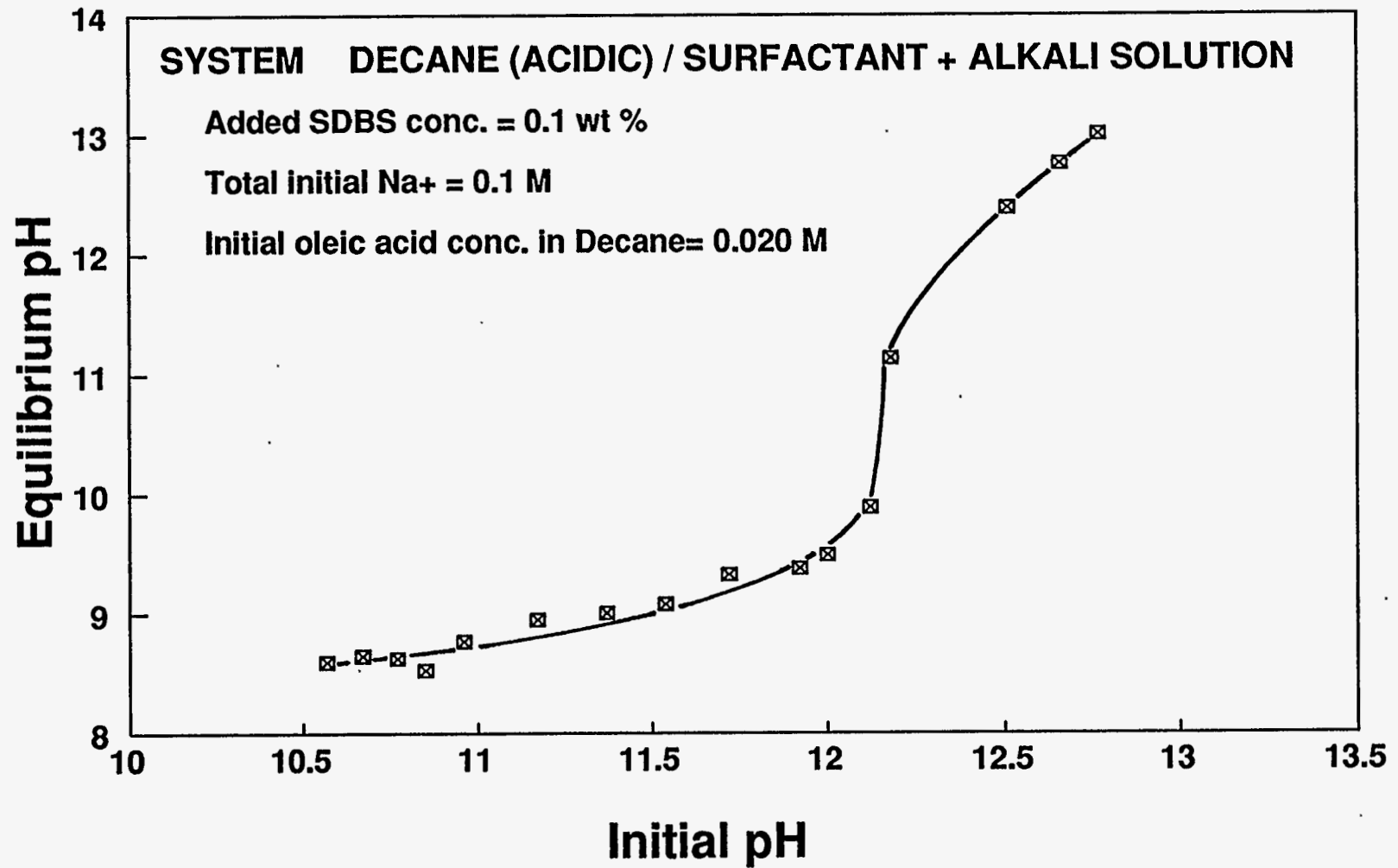
Figure 2-2. Experimentally Determined Variation in Equilibrium pH with Initial pH of the Aqueous Phase
