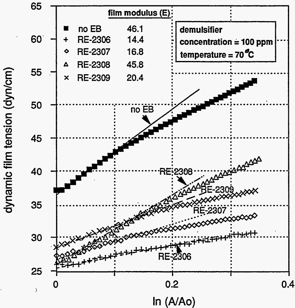
Figure 3-3. Film tension as a function of film area at 100 ppm demulsifier, 70°C. The initial slope represents film modulus at 2.7 \times 10^{-2} mm 2 /sec film expansion rate.
