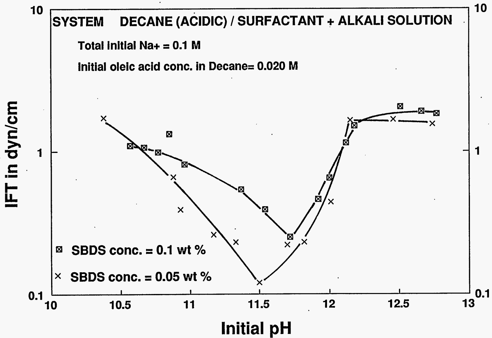
Figure 2-3. Experimentally Determined Effect of Surfactant Concentration on the Variation of IFT Over pH of the Aqueous Phase
