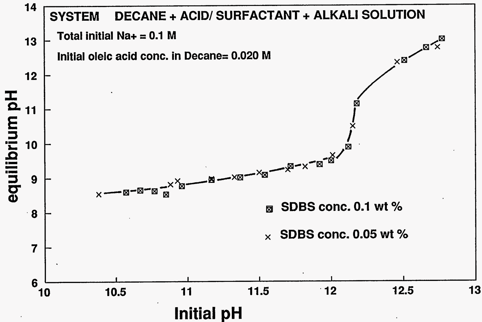
Figure 2-4. Experimentally Determined Effect of Surfactant Concentration on the Variation of Equilibrium pH Over Initial pH of the Aqueous Phase
