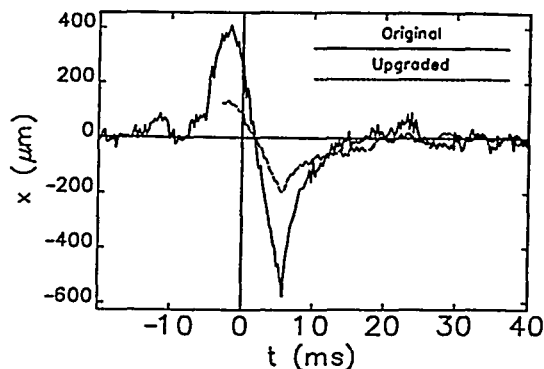
Figure 2: Closed orbit bump due to septum leakage
