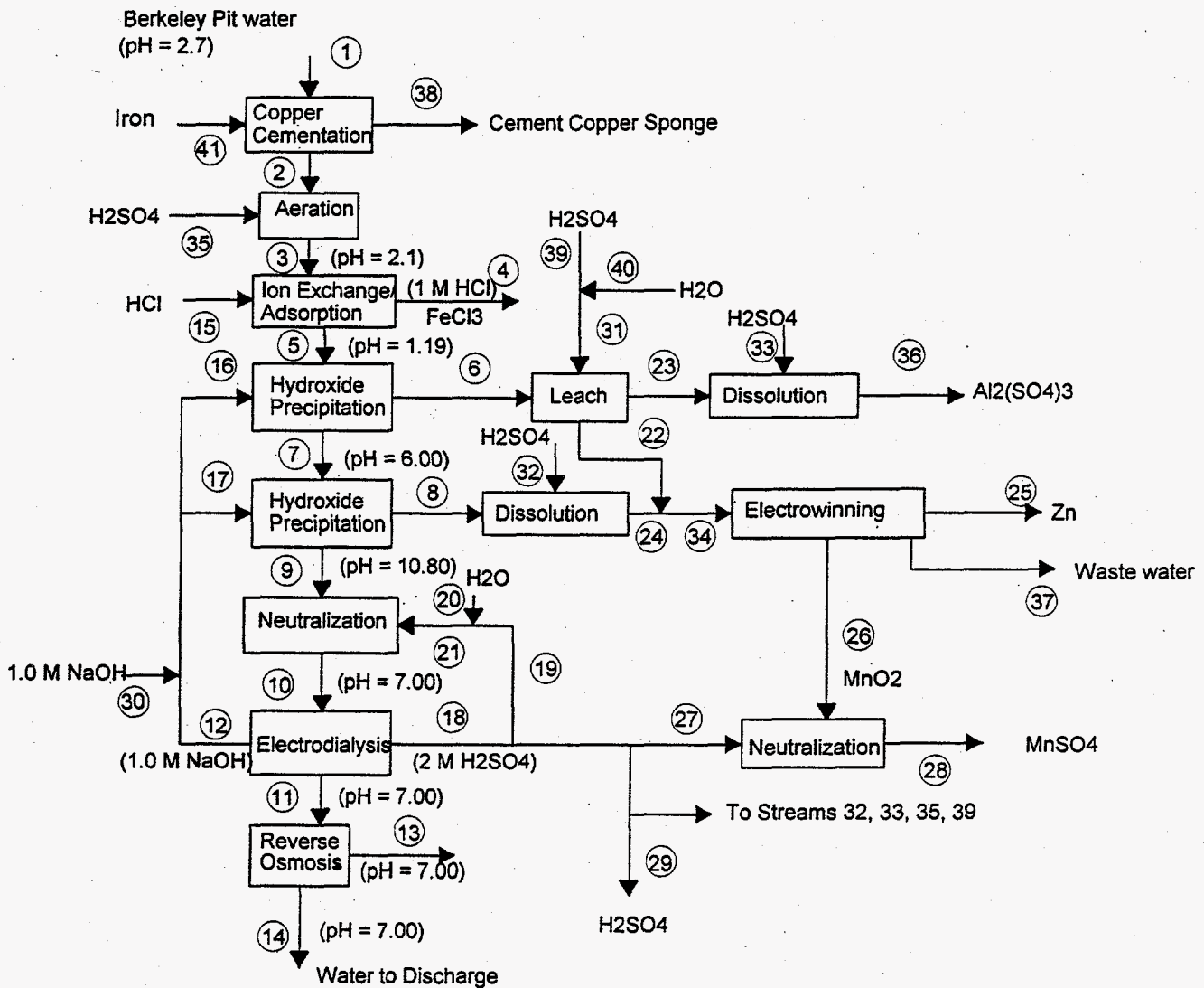
Figure 2. Flowsheet Showing Series Separation of Constituents
