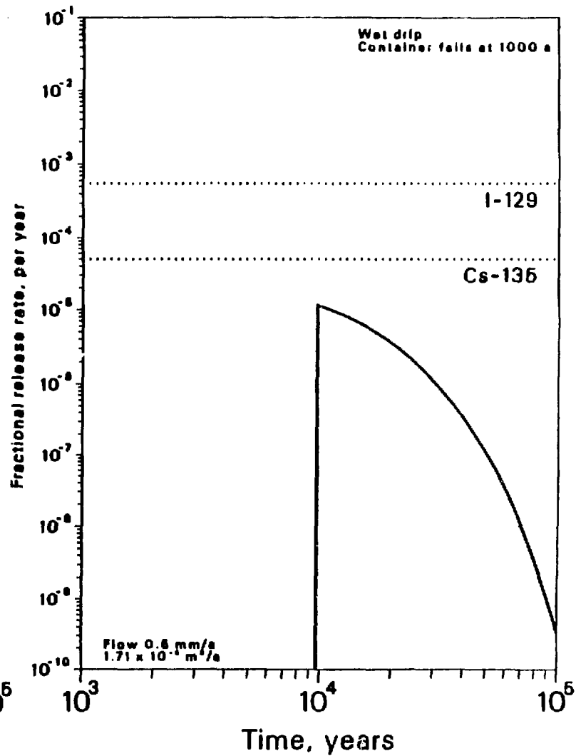
Figure 7. The Fractional Release Rates of Soluble Species
