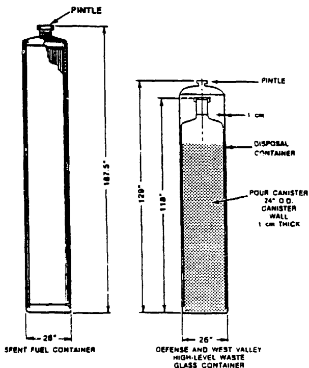
Figure 1. Typical Waste Packages
