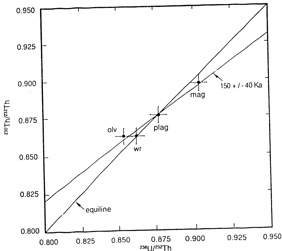
Figure 3: Plot of ^{230}\text{Th}/^{232}\text{Th} versus ^{238}\text{U}/^{232}\text{Th} for the \text{QI}_4 lava of the Lathrop Wells center.
