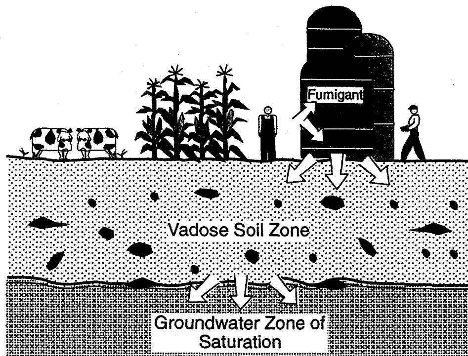
FIGURE 1 Source of Carbon Tetrachloride and Chloroform in Soils and Groundwater at Former CCC/USDA Grain Storage Sites
