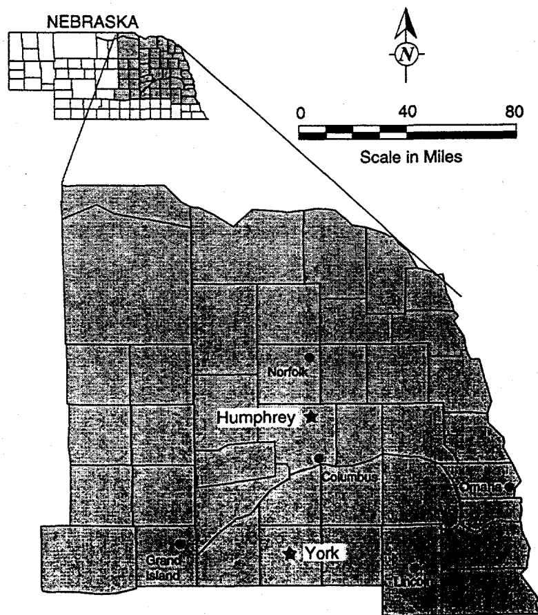
FIGURE 3 Locations of York and Humphrey, Nebraska
