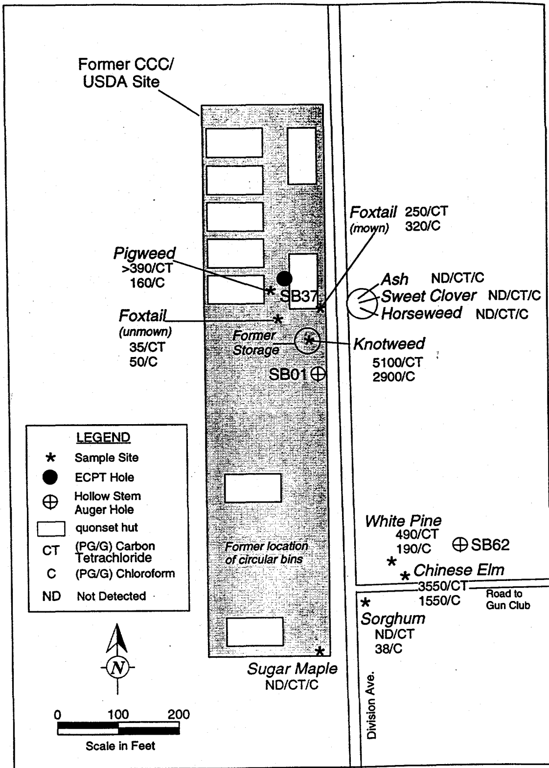
FIGURE 5 Distribution of Carbon Tetrachloride and Chloroform in Various Plant Species at York
