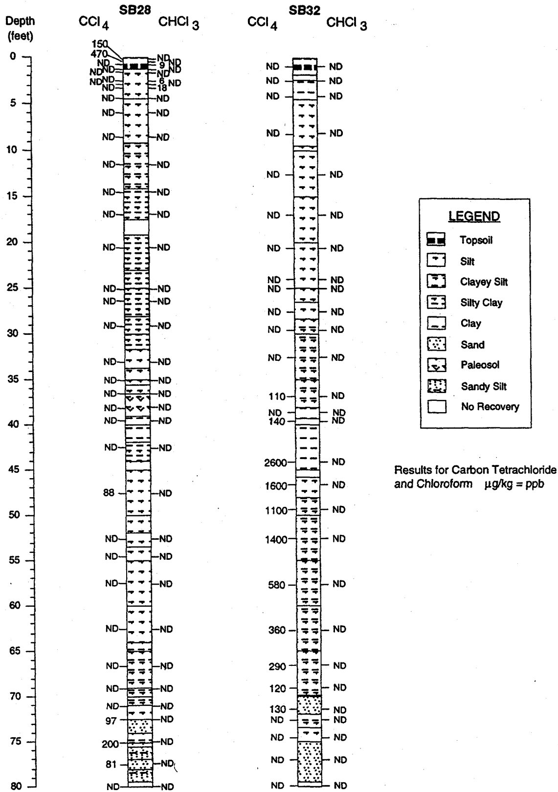
FIGURE 9 Vertical Distribution of Carbon Tetrachloride and Chloroform Concentrations in SB28 and SB32 at Humphrey
