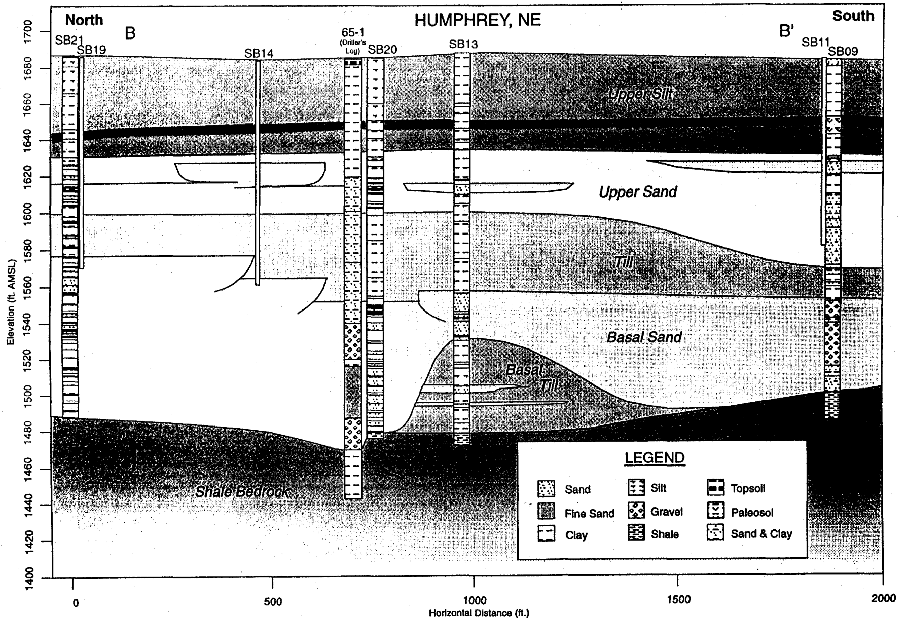
FIGURE 2 Geologic Cross Section B-B' at Humphrey, Nebraska
