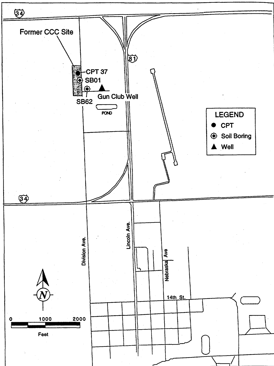
FIGURE 4 Locations of Soil Borings Used for Vadose Zone Soil Sampling at York
