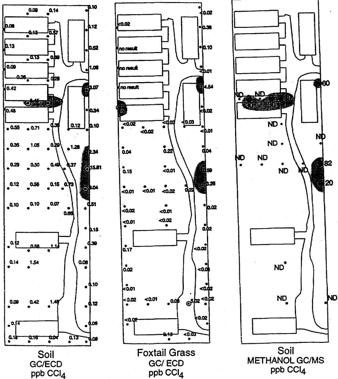
FIGURE 6 Carbon Tetrachloride Concentration Patterns in Soil and Vegetation at York
