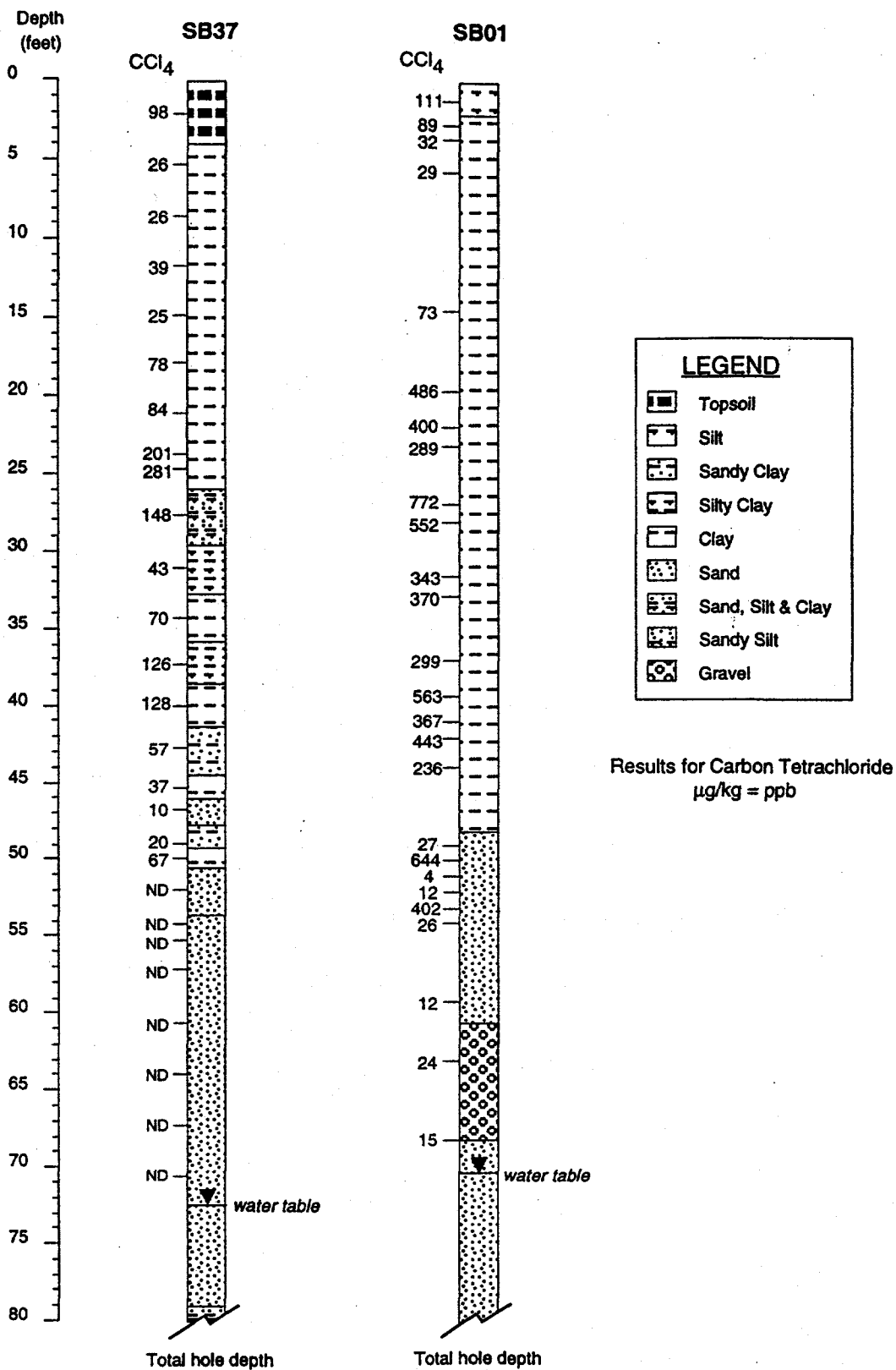
FIGURE 7 Vertical Distribution of Carbon Tetrachloride Concentrations in SB01 and SB37 at York
