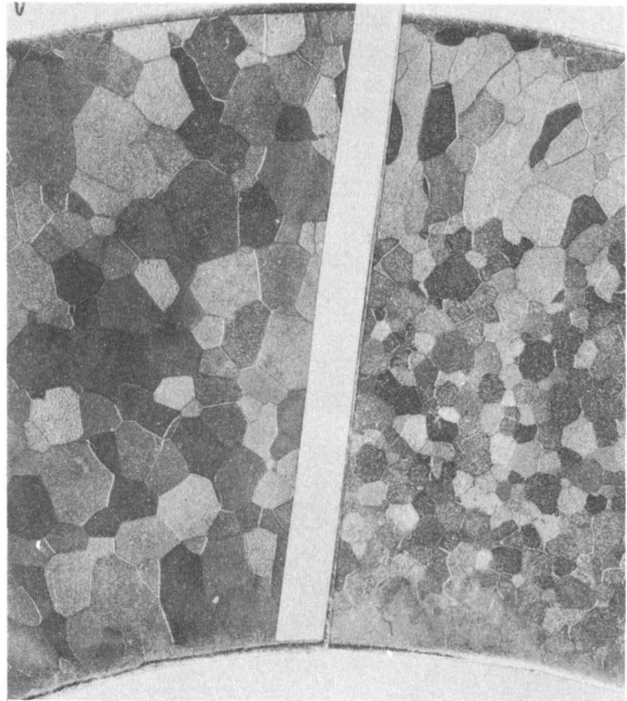
Figure 159.—Sections taken from opposite ends of cylinder, showing variation in grain size ( \times 6 ).
