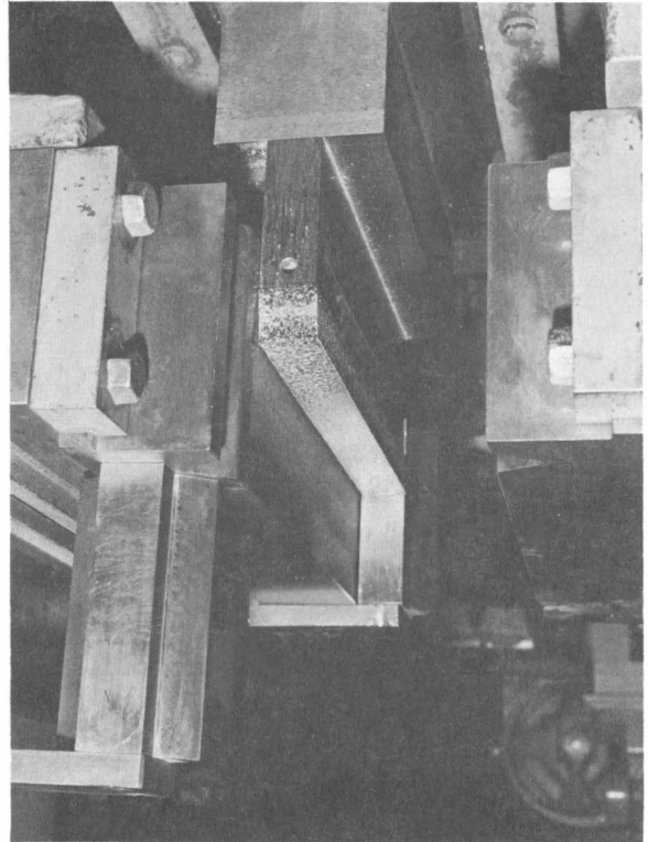
Figure 66.—Briquetting die for 2- by 2- by 20-in sponge electrodes.
