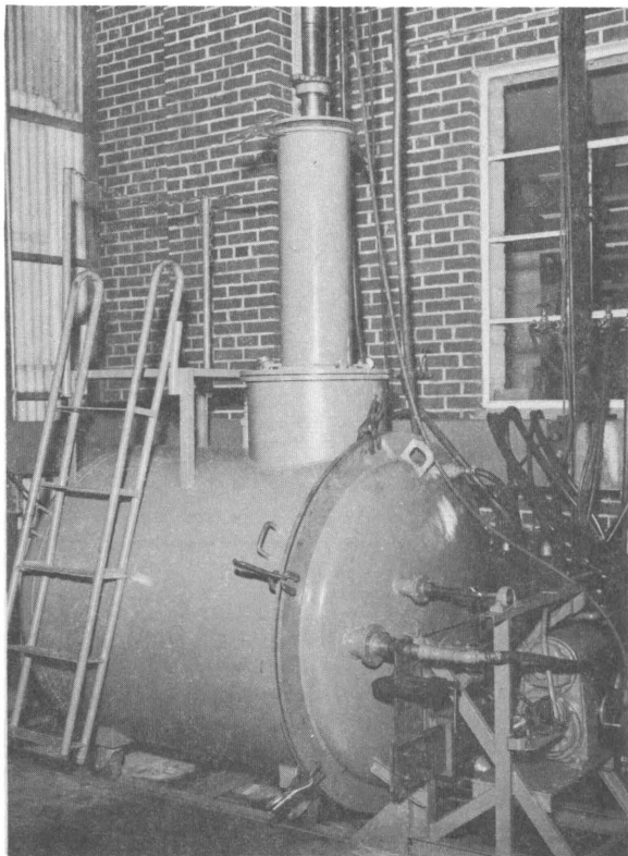
Figure 95.—Improved over-the-lip casting furnace (as installed).
