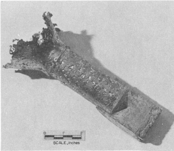
Figure 29.—Static-cast oxygen-free copper, graphite mold.
