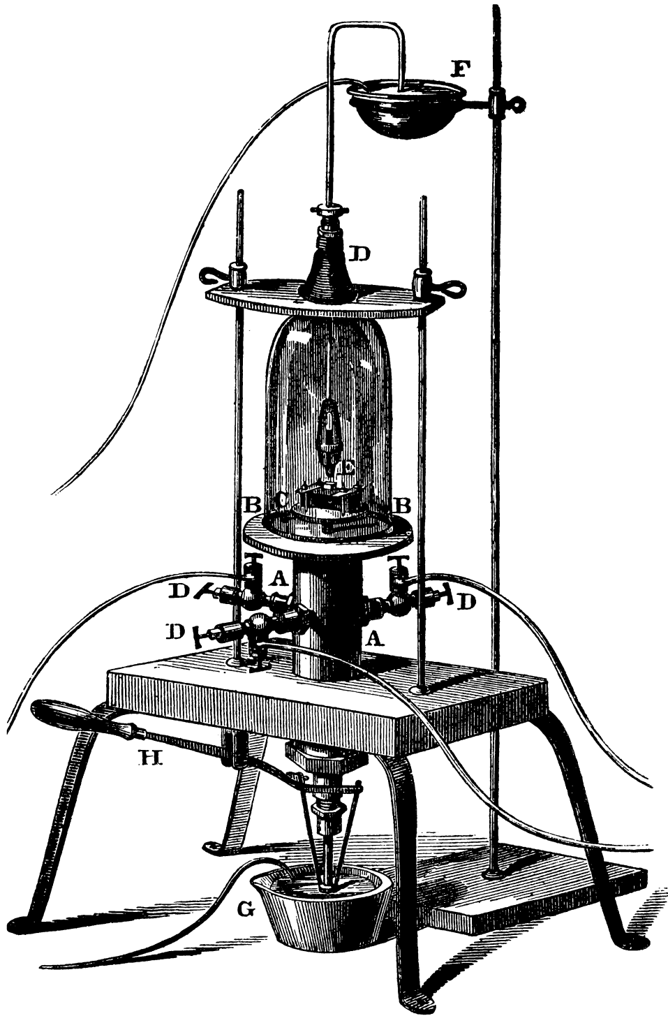
Frontispiece.—Robert Hare's deflagrator. The first controlled atmosphere arc furnace. (Reproduced from article published in 1839.)
