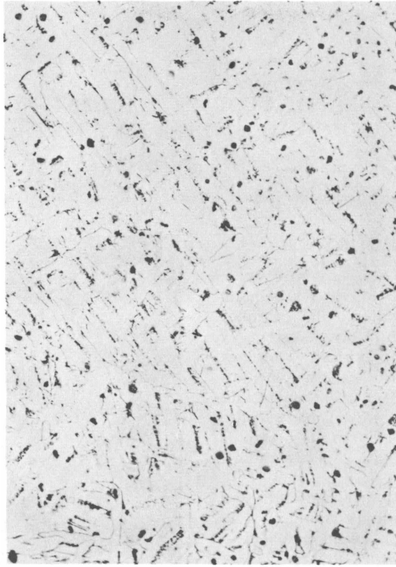
Figure 143.—Microstructure of zirconium ingot used as feed material for casting SA 21,674. Etch: 45 ml H 2 O, 45 ml HNO 3 , 10 ml HF (× 100).
