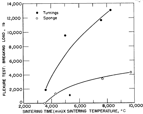
Figure 70.—Strength of electrodes vs. sintering time and temperature (4-in-diam compacts; 8½-in anvil separation).
