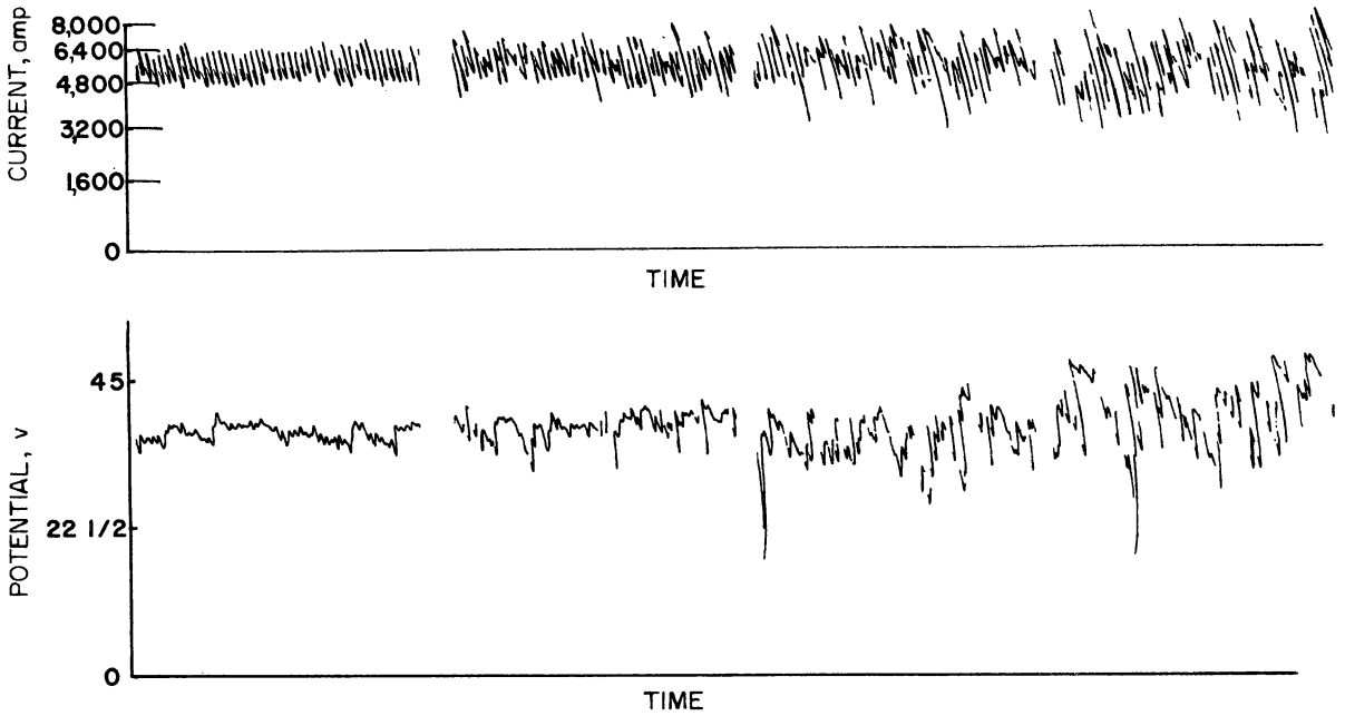
Figure 45.—Potential and current (recorded at 5 cm/sec).
