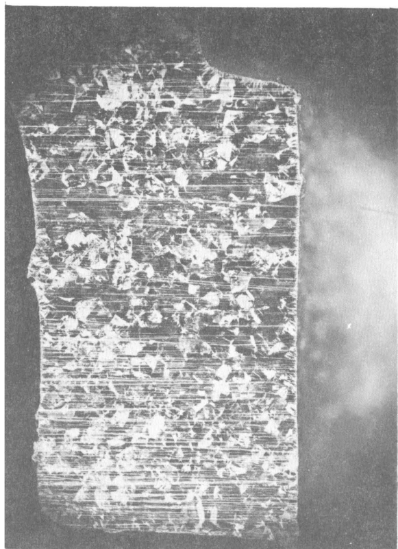
Figure 130. —Grain structure of cast titanium in mold material XM-64. Etch: 45 H 2 O, 45 HNO 3 10 HF (× 10).
