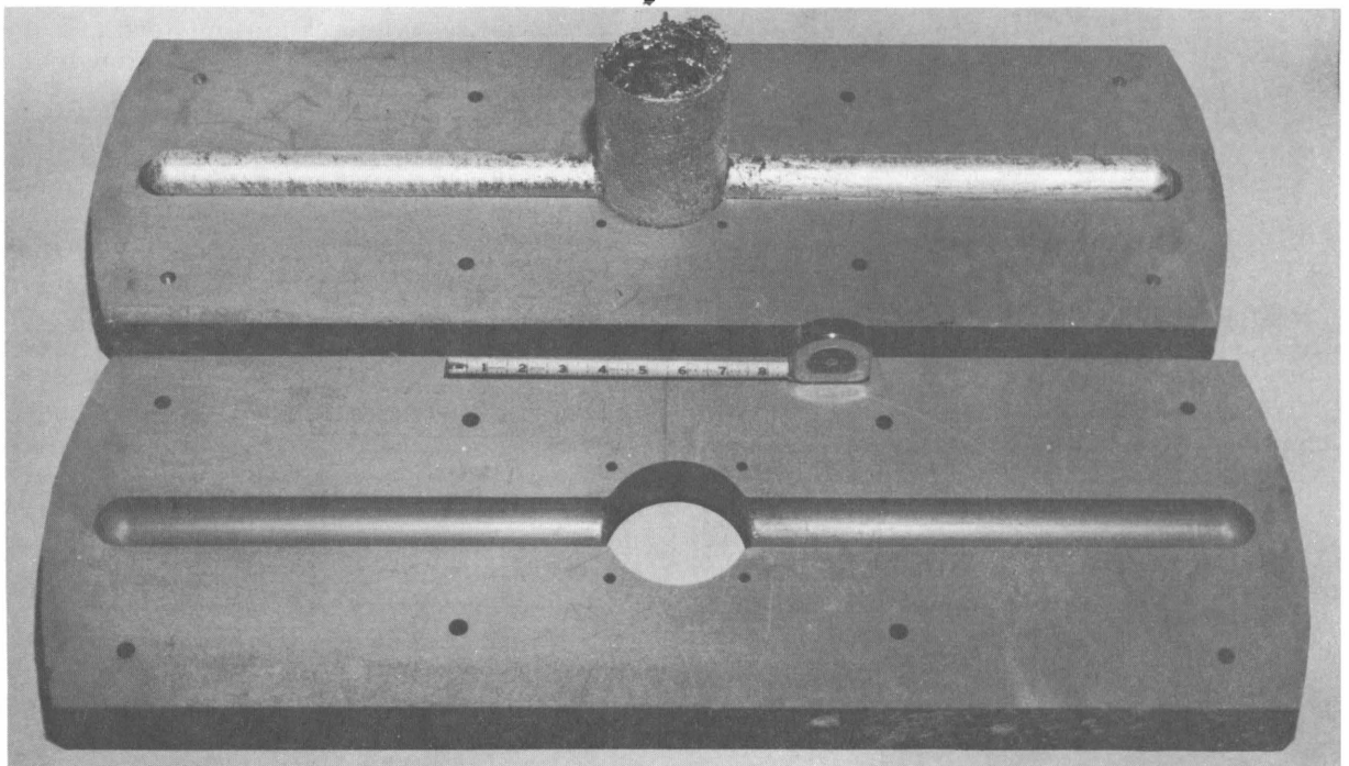
Figure 166.—Pressure casting tungsten rods.
