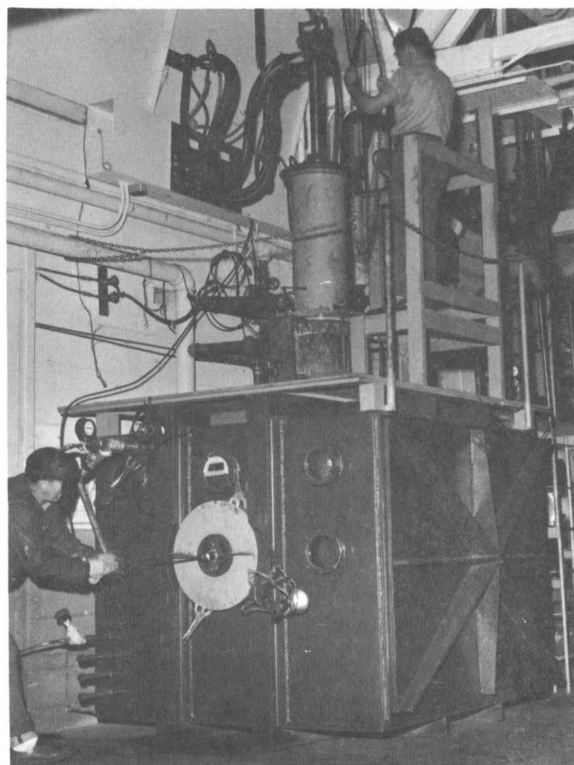
Figure 85.—Large-scale bottom-pour casting furnace.
