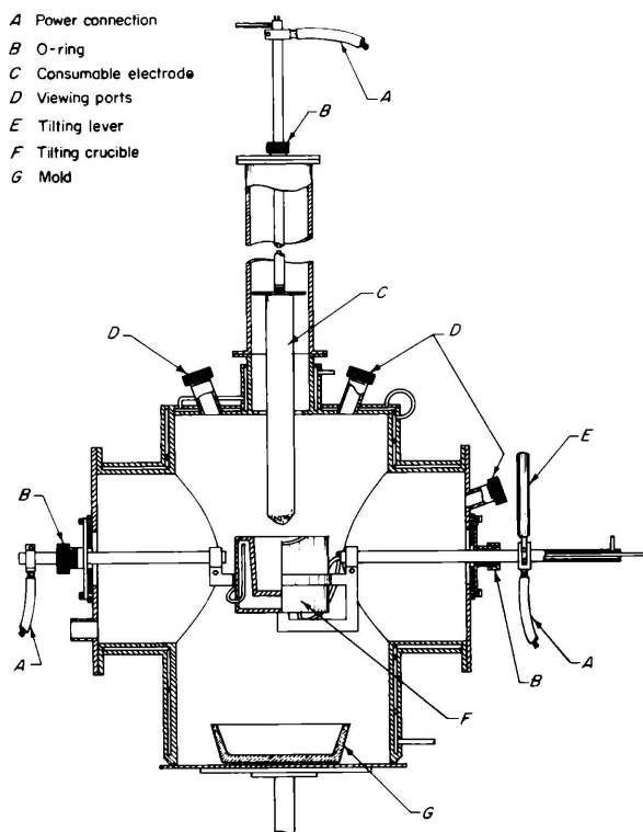
Figure 87.—Schematic diagram of pour-over-the-lip furnace.
