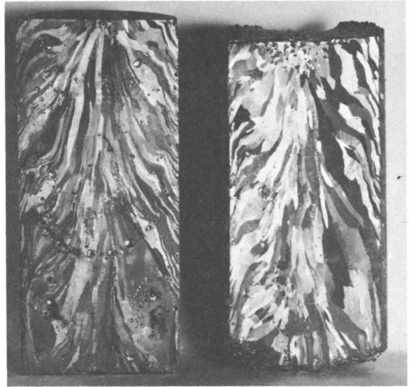
Figure 17.—Chromium ingots illustrating effect of premelting degassing treatment.
