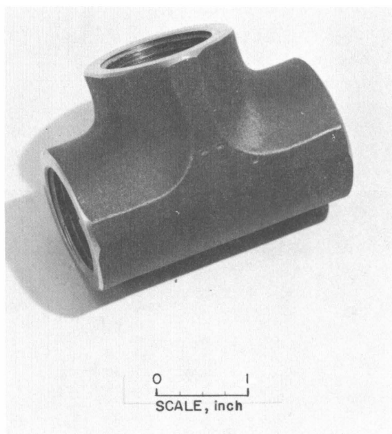
Figure 140.—Finished zirconium pipe tee with sandblasted surface, cast in mold material XM-71.
