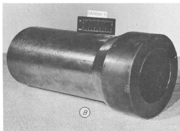
Figure 84.— A , cast titanium tools; B , cast titanium breech liner.
