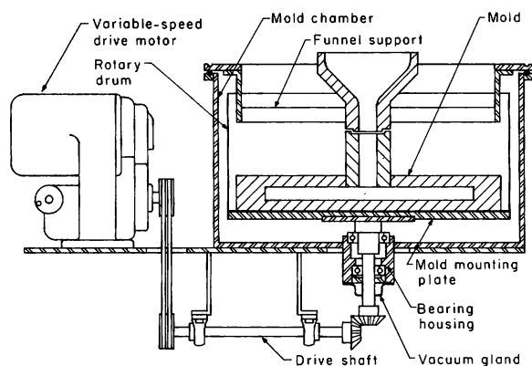
Figure 162.—Vertical axis casting mechanism.
