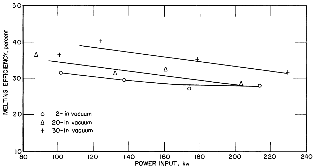
Figure 42.—Melting efficiency vs. power input, series 5 (reverse polarity).
