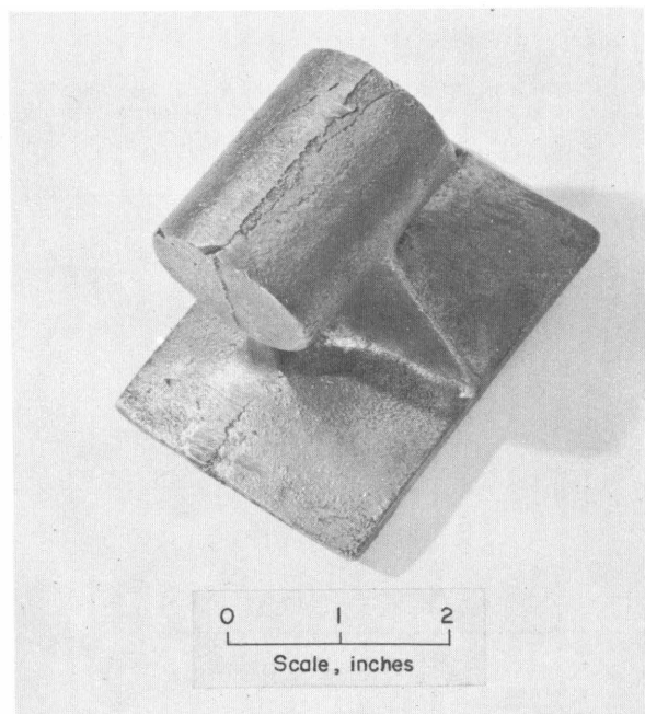
Figure 110.—Zirconium torsion-bar bracket.
