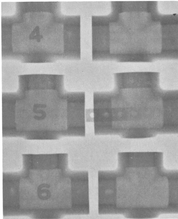
Figure 127.—Radiograph of castings from vented molds.
