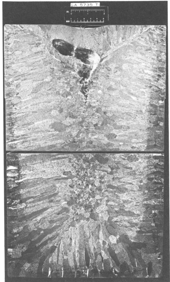
Figure 81.—Longitudinal section of a titanium ingot, showing deep pool.
