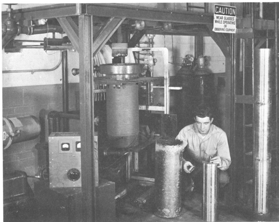
Figure 9.—Large furnace with ingot and electrode made of first-melt ingots.
