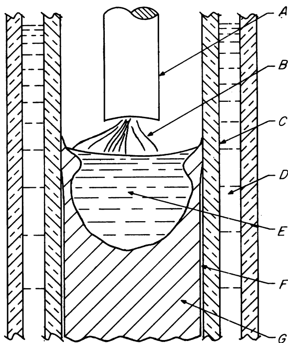
A Electrode B Direct current arc C Copper crucible wall D Water jacket E Molten pool F Shrinkage gap G Ingot
