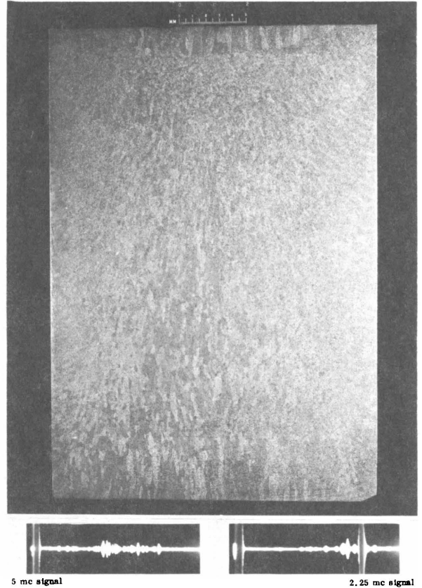
Figure 80.—A concentration of porosity near the top of this ingot was delineated in the reflectograms shown.
