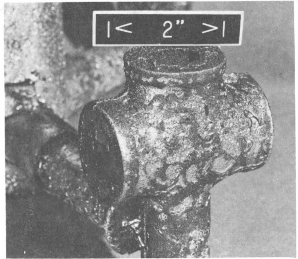
Figure 155.—Molybdenum pipe tee, cast in expendable graphite.
