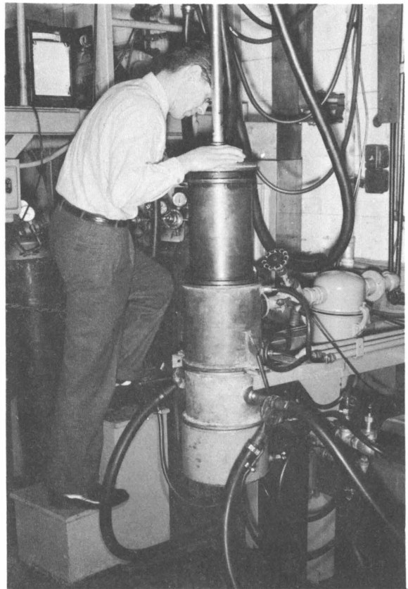
Figure 144.—Overall view of casting furnace.
