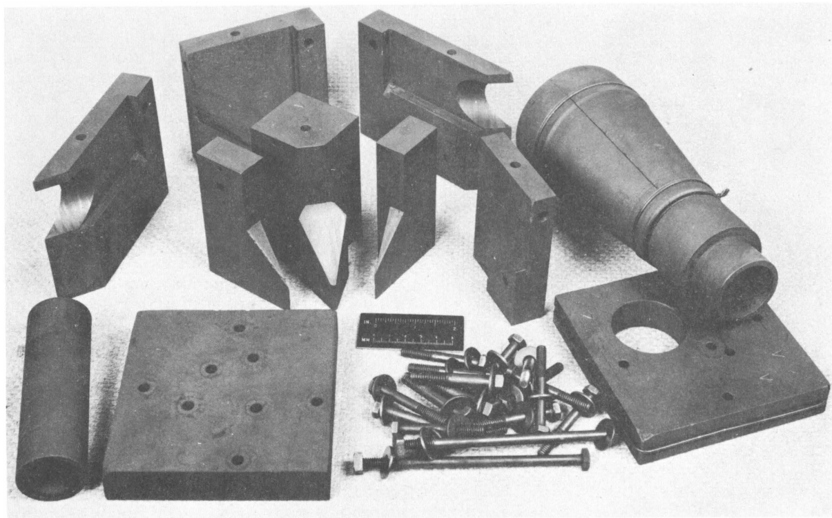
Figure 108.—Machined graphite mold with laminated core, disassembled.
