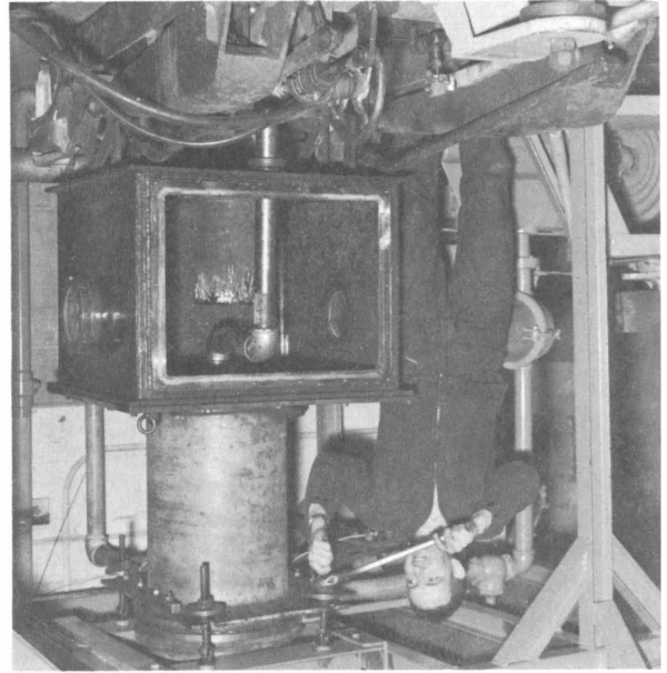
Figure 83.—Crucible and mold box, bottom-pour furnace.
