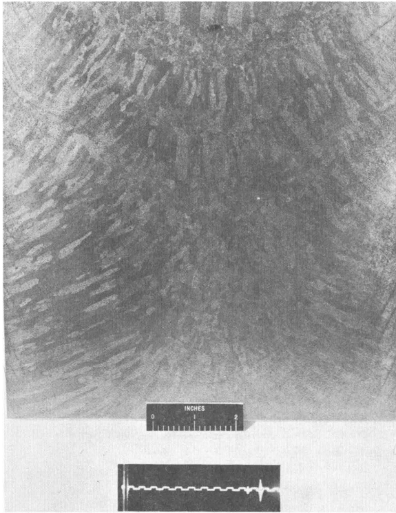
Figure 79.—Ingot containing shrink hole and typical square-wave sweep signal used in locating similar flaws.
