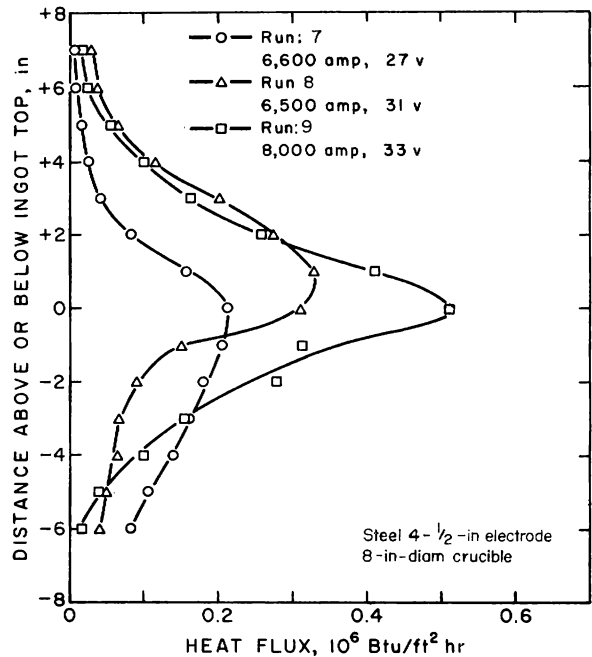
Figure 62.—Effect of arc current and arc potential on heat flux to crucible wall during melting of steel electrodes.
