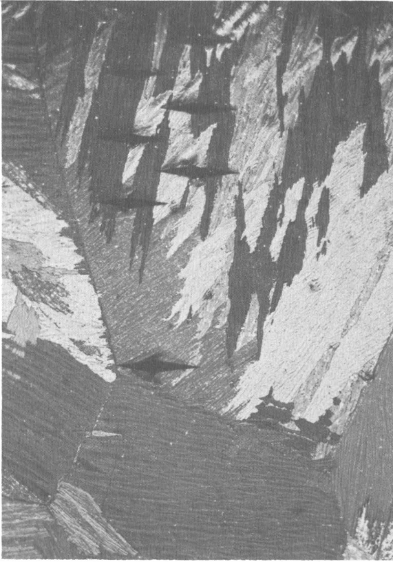
Figure 137.—Microstructure of titanium cast in XM-76 near cast surface. Etch: 45 ml H 2 O, 45 ml HNO 3 , 10 ml HF ( \times 50).
