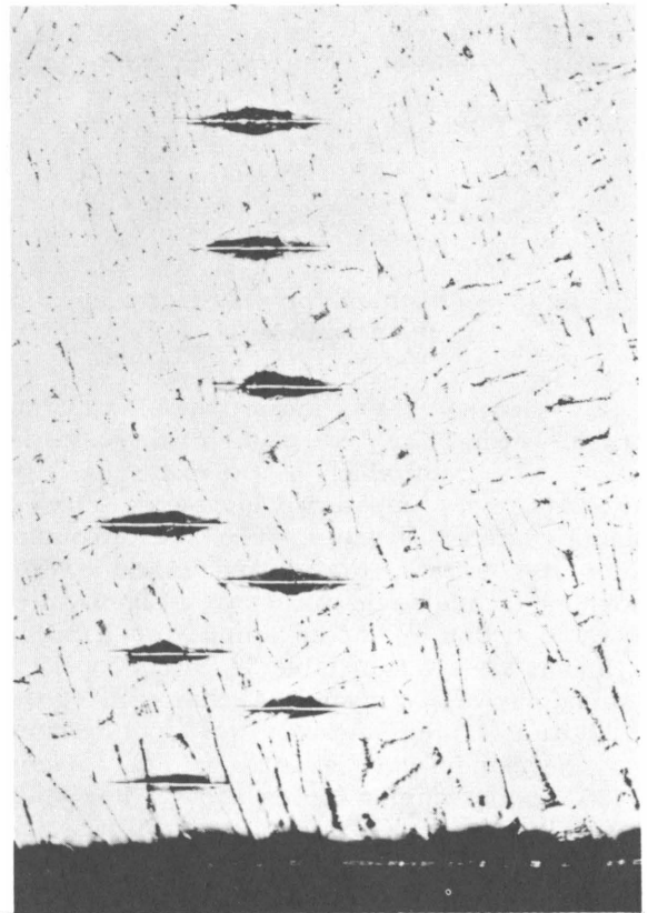
Figure 142.—Microstructure of zirconium cast in mold material BW near cast surface (SA 21,674). Etch: 45 ml H 2 O, 45 ml HNO 3 , 10 ml HF ( \times 100 ).
