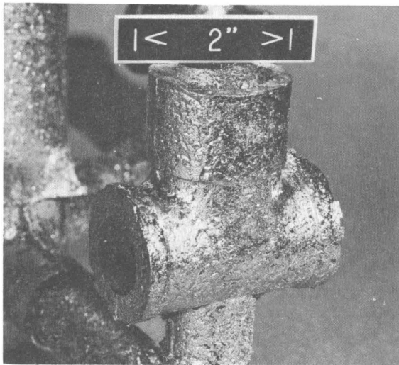
Figure 156.—Molybdenum pipe tee, cast in machined graphite.
