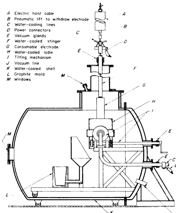
Figure 92.—Improved over-the-lip casting furnace (schematic).
