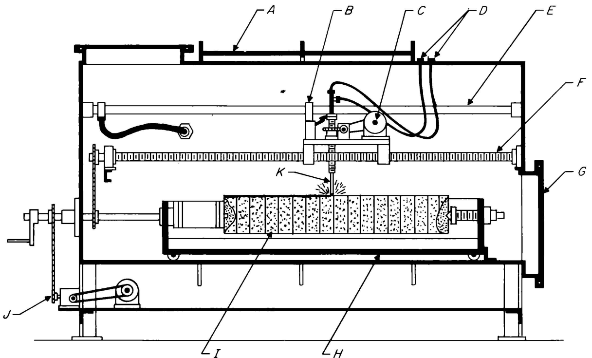
Figure 72.—Inert atmosphere automatic welding box.
