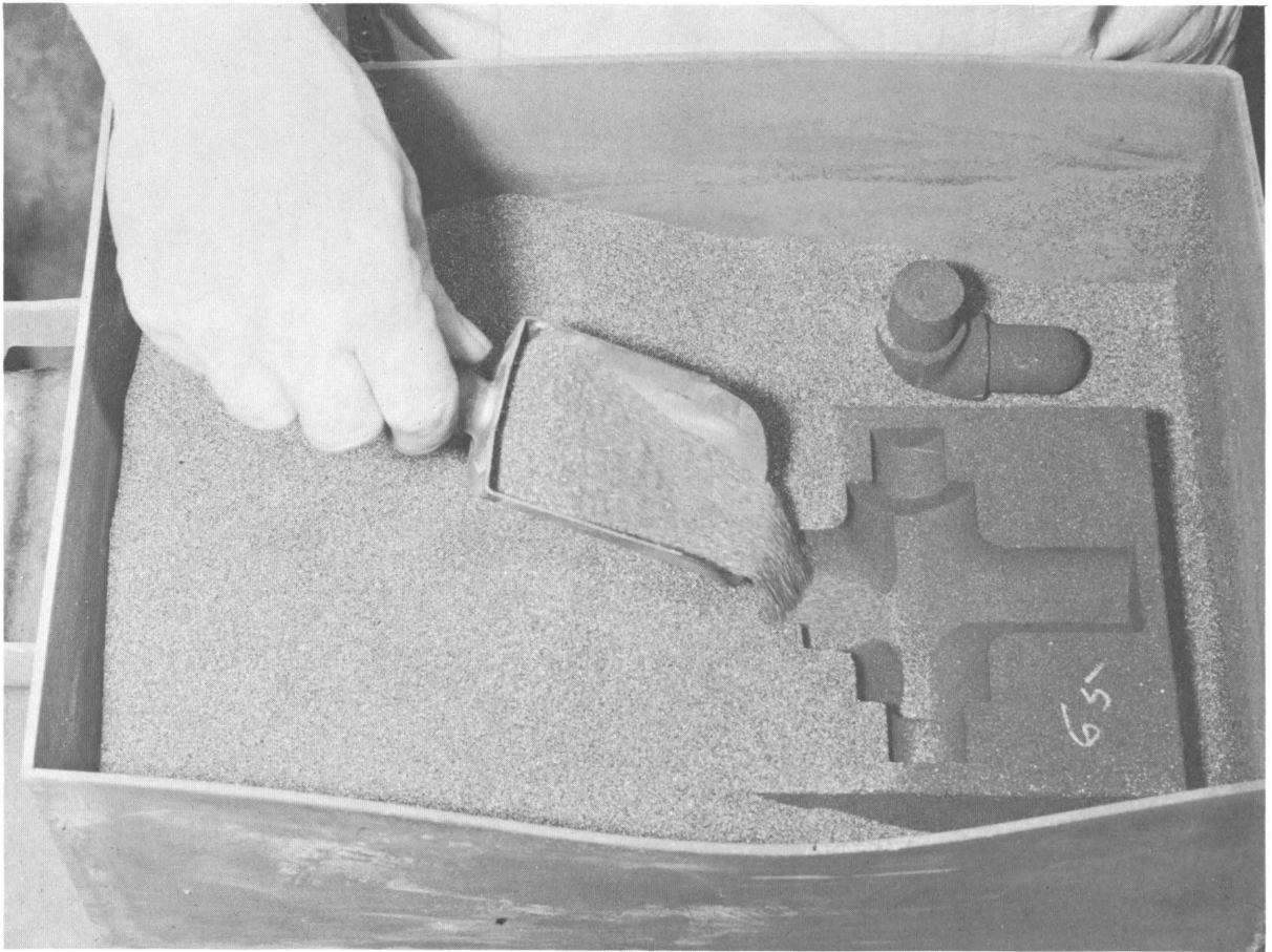
Figure 123.—Mold and core bedded in coke prior to firing.
