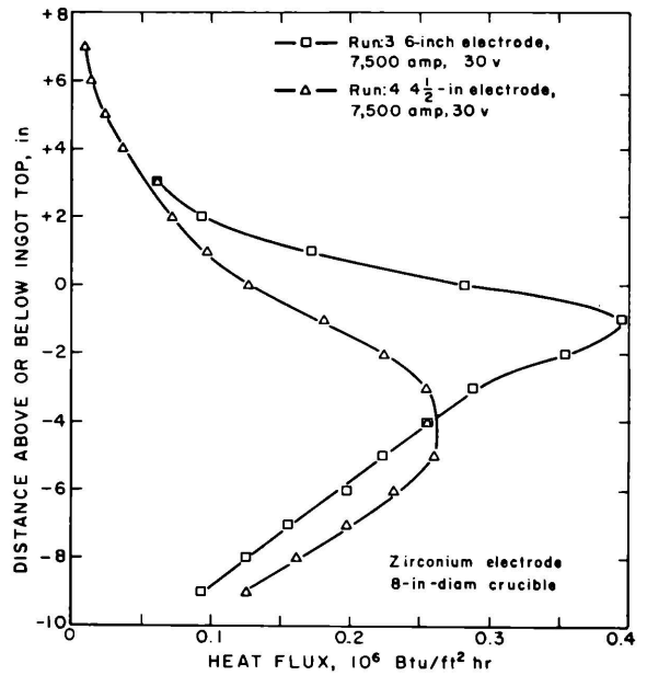
Figure 58.—Effect of electrode diameter on heat flux to crucible wall.
