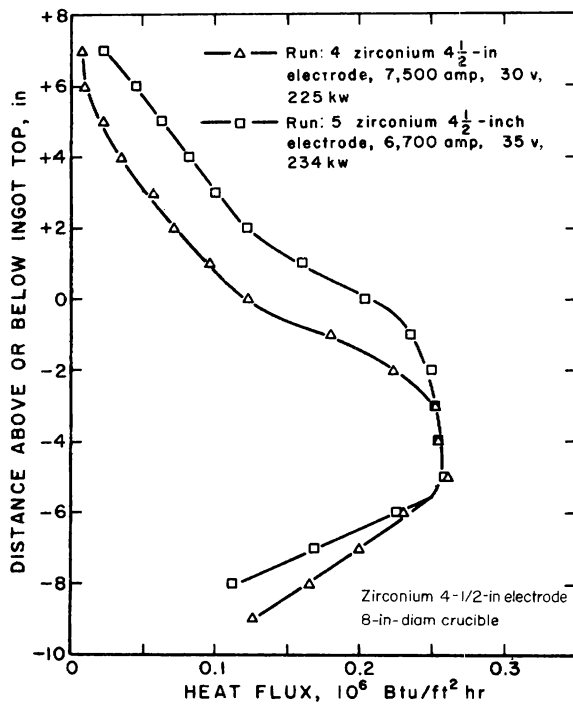
Figure 61.—Effect of arc current and arc potential on heat flux to crucible wall during melting of zirconium electrodes.
