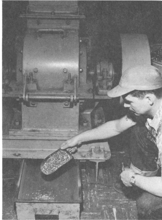
Figure 74. —Hammer mill for processing machine chips.
