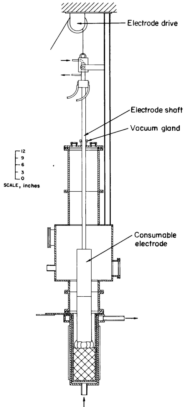
Figure 8.—Large furnace capable of remelting 6-in-diam ingots.
