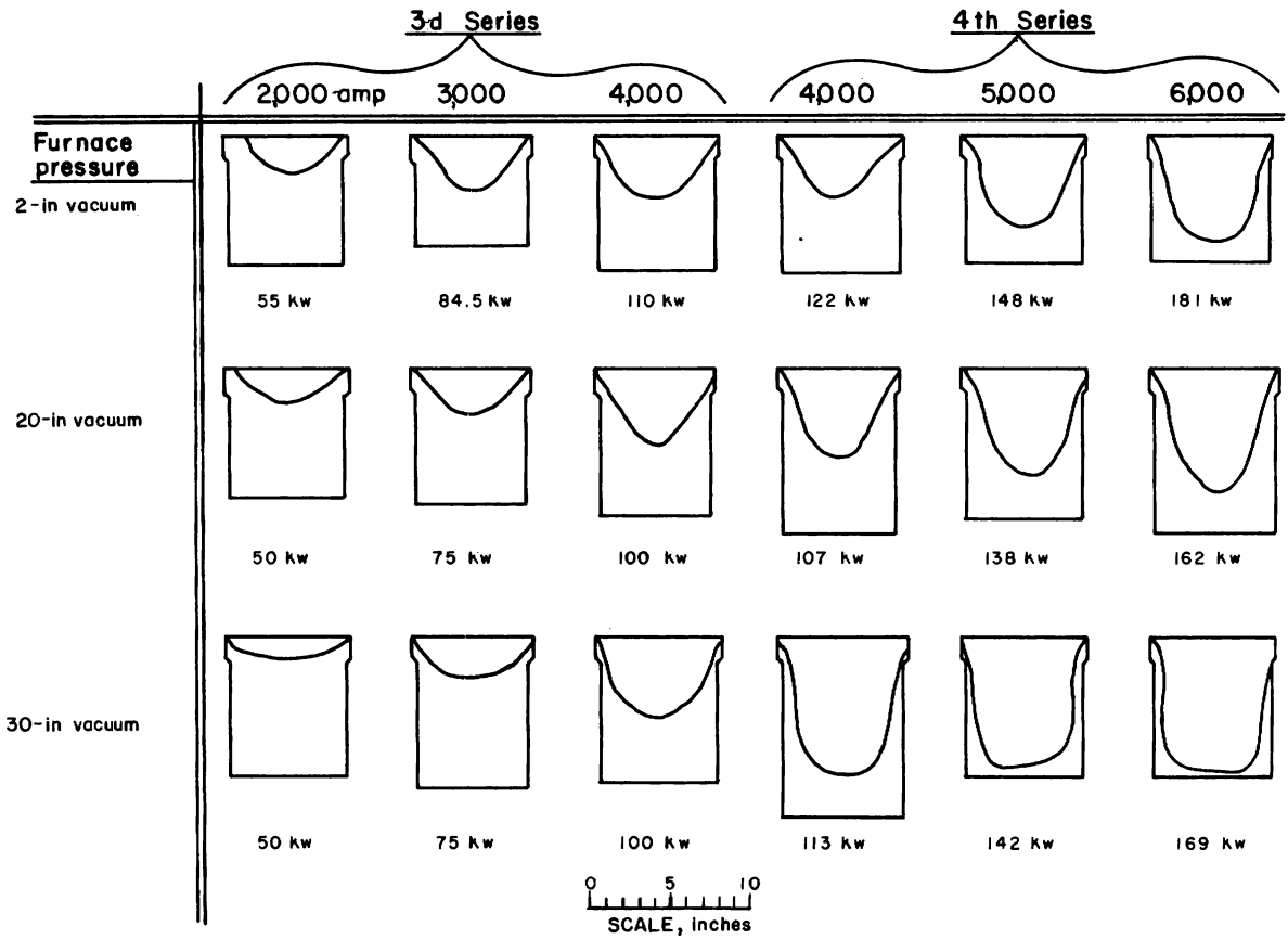
Figure 32.—Pool shapes for series 3 and 4 (straight polarity).
