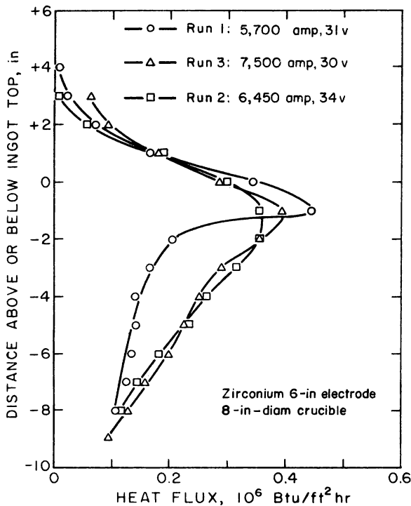
Figure 63.—Effect of arc current and arc potential on heat flux to crucible wall during melting of 6-in-diam zirconium electrodes.
