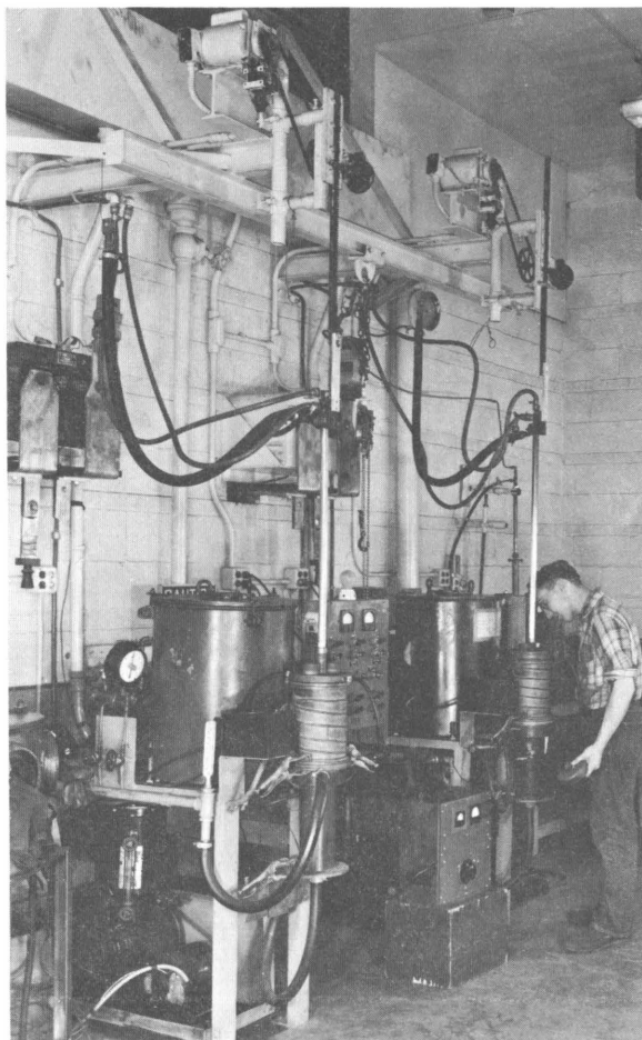
Figure 1.—Two laboratory arc furnaces.
