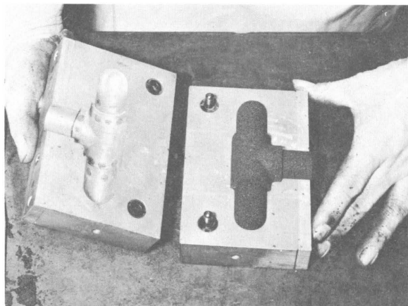
Figure 121.—Core blow box and core for 1-in pipe tee.
