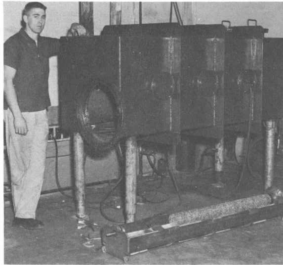
Figure 72.—Inert atmosphere automatic welding box.
