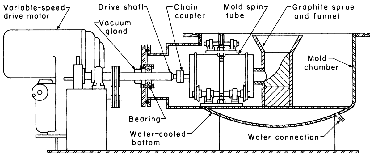
Figure 163.—Horizontal axis casting mechanism.
