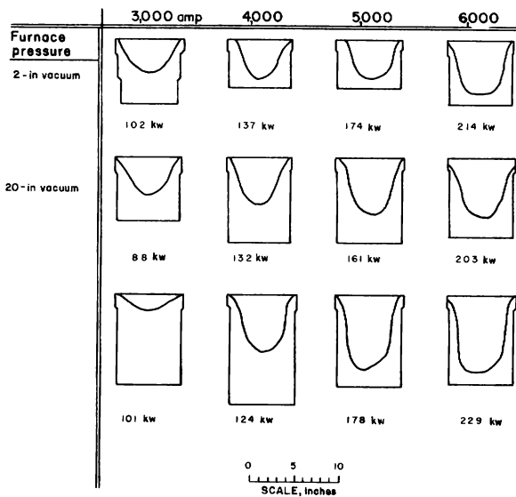
Figure 33.—Pool shapes for series 5 (reverse polarity).
