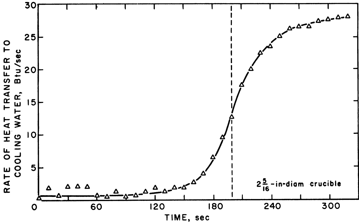
Figure 54.—Rate of heat transfer to upper crucible section during consumable electrode arc melting. Zirconium electrode.
