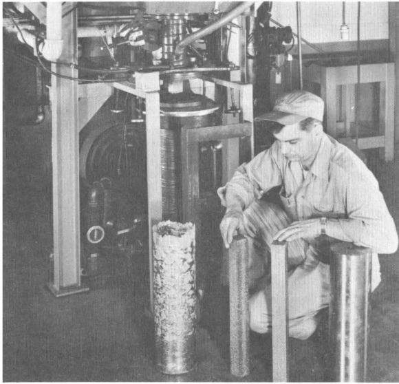
Figure 3.—Melting section of furnace with consumable pressed electrodes and ingots in foreground.
