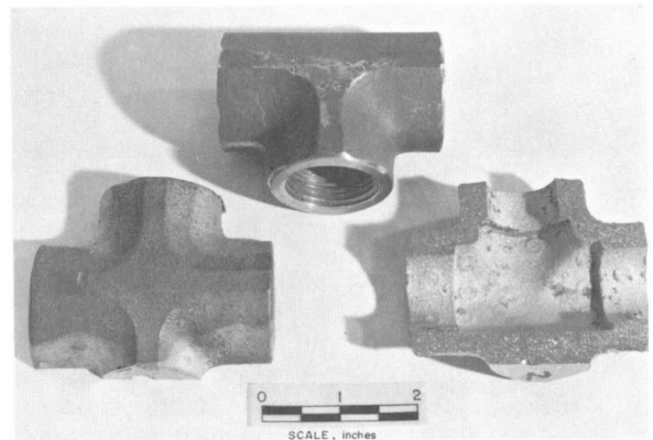
Figure 129.—Sectioned cast titanium pipe tees (SA 22,511) from CO 2 mulled expendable mold material XM-64.
