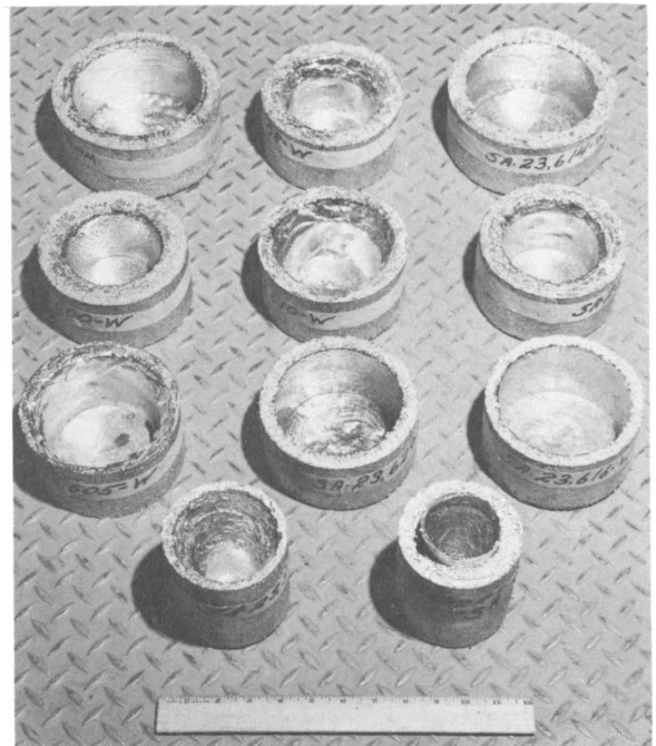
Figure 164.—Group of spin castings: Note the differences inside the bores of the cylinders.
