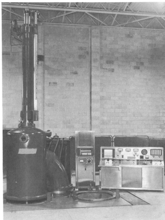
Figure 11.—Consarc 30-12 production vacuum arc furnace in test bay before shipment.
