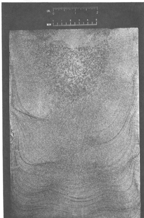
Figure 6.—Single melt ingot using 1.4 amp for solenoid stirring causing centrifuging of tin to sidewalls.
