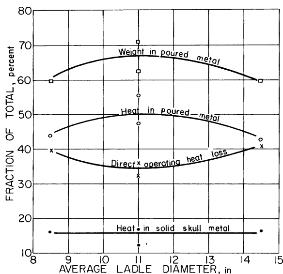
Figure 104.—Heat distribution and metal yield as functions of ladle diameter.
