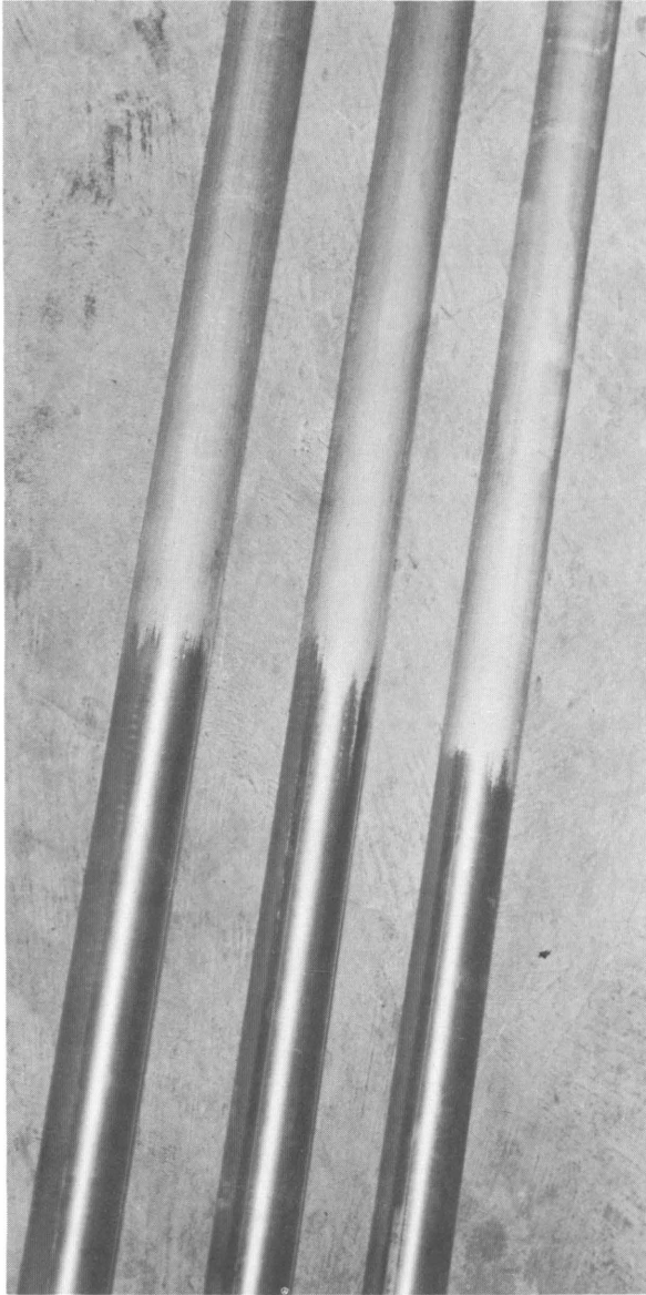
Figure 100.—Extruded Zircaloy-2 tubing directly from as-cast billet, showing original surface and ground finish.
