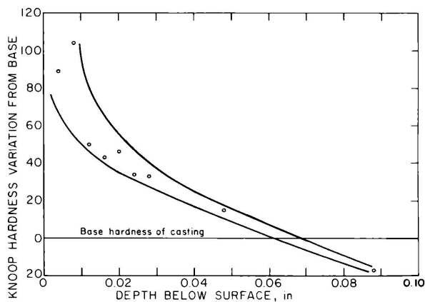
Figure 134.—Average depth of surface hardening effect in eight titanium castings.
