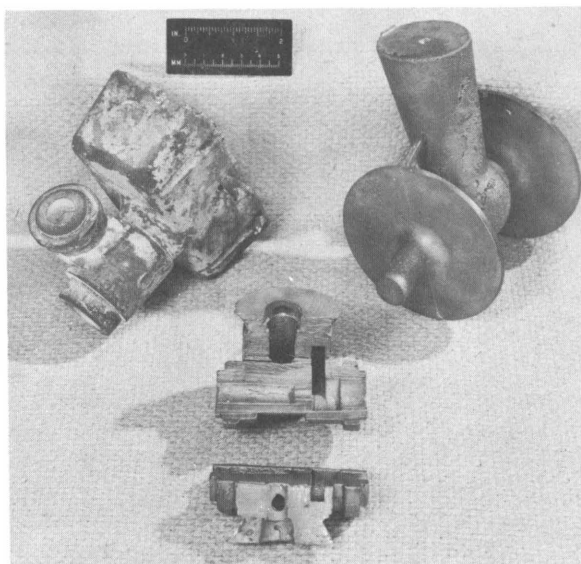
Figure 111.—Titanium castings from frozen mercury molds provided by Alloy Precision Casting Co.
