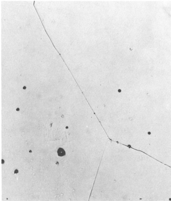
Figure 26.—Photomicrograph of oxygen-free copper vacuum-arc-melted in graphite-lined crucible ( \times 250 ).
