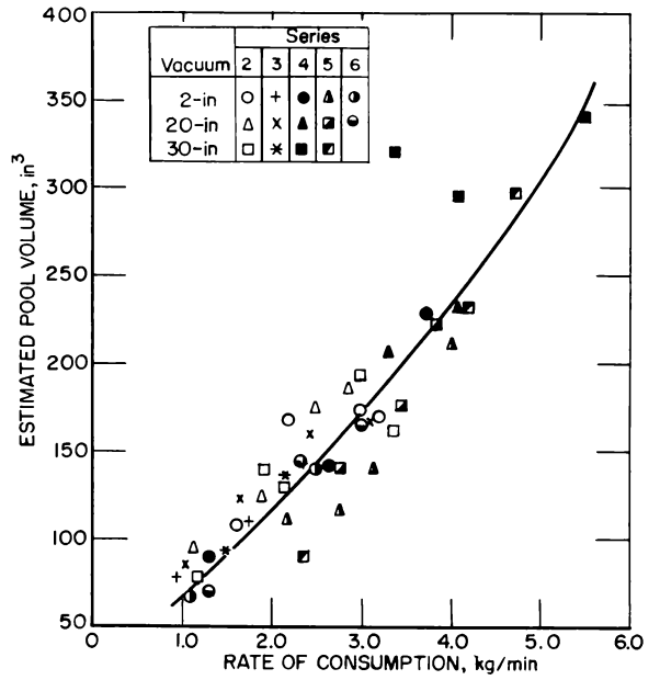
Figure 38.—Estimated pool volume vs. rate of consumption.
