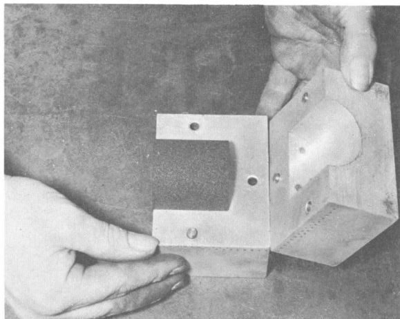
Figure 120.—Core blow box and core for 2- by 2-in permeability specimen.
