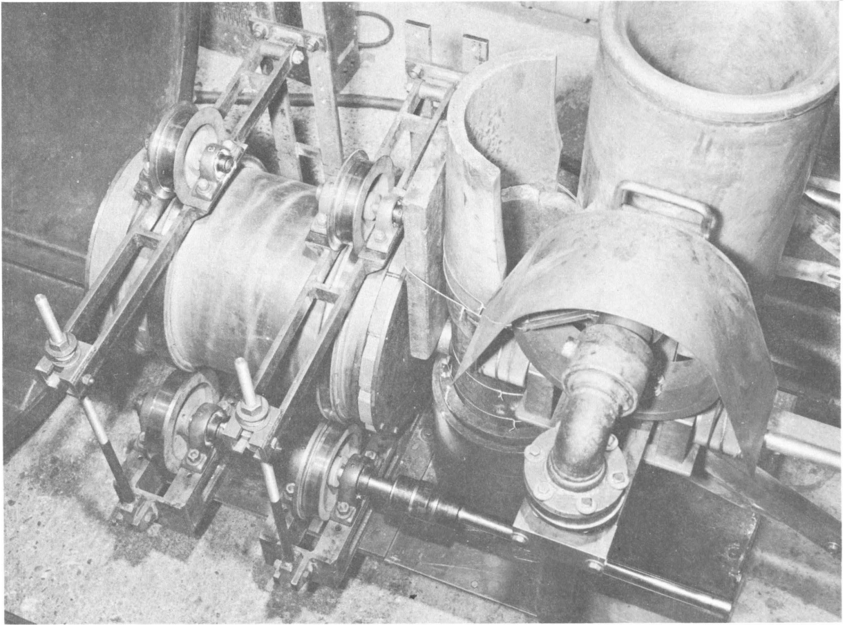
Figure 98.—Spin casting mechanism, showing crucible and pouring funnel on right.
