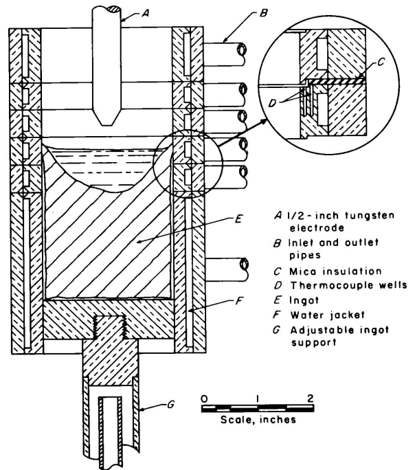
Figure 49.—Six-piece crucible for heat transfer studies during nonconsumable electrode arc melting.
