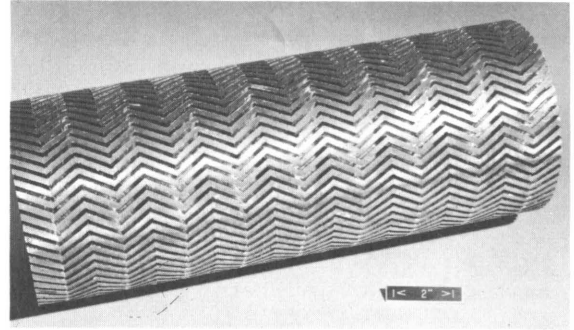
Figure 22.—Finned copper casting after machining.
