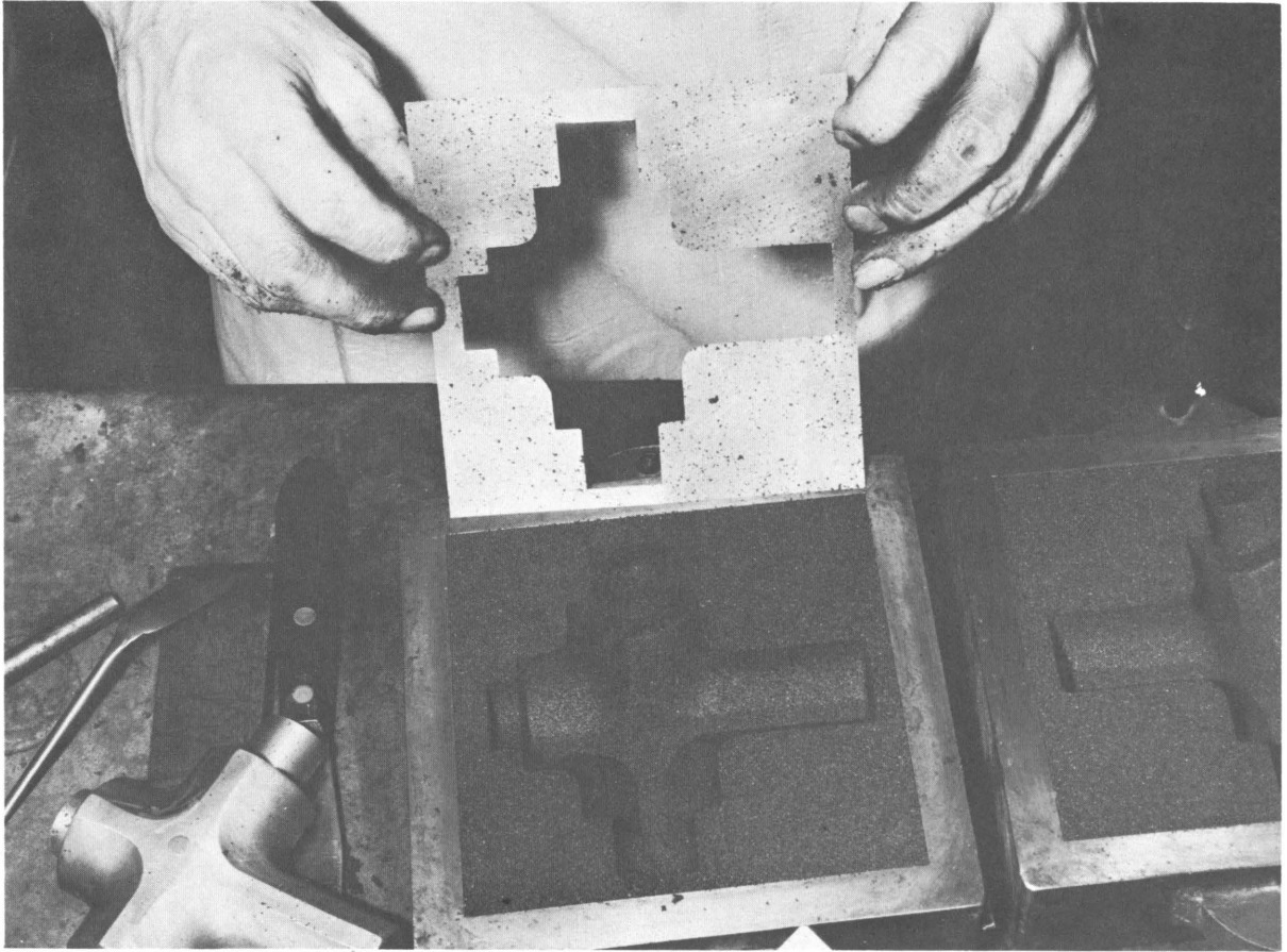
Figure 119.—Metal shim stock is removed after the mold has been rammed.
