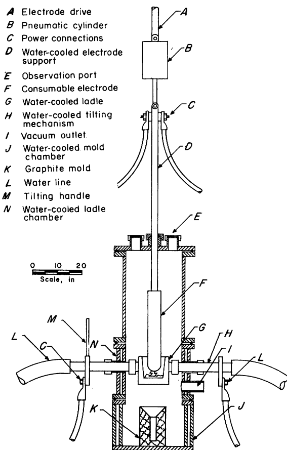
Figure 145.—Laboratory-scale casting furnace.
