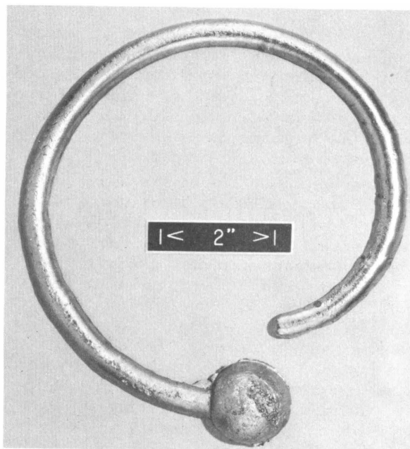
Figure 150.—Fluidity spiral of columbium.
