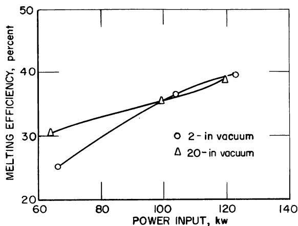
Figure 43.—Melting efficiency vs. power input, series 6 (alternating current).
