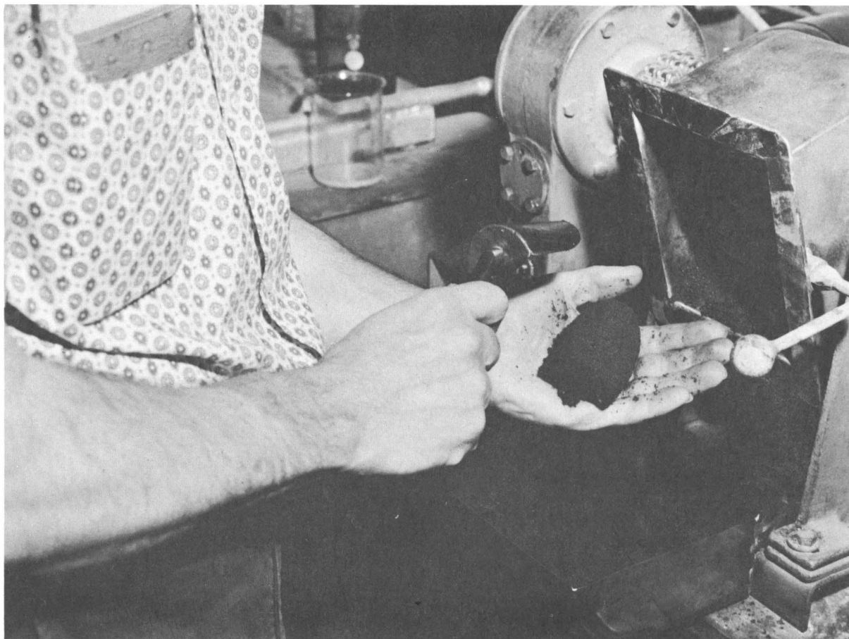
Figure 118.—Test of mold material moist consistency.
