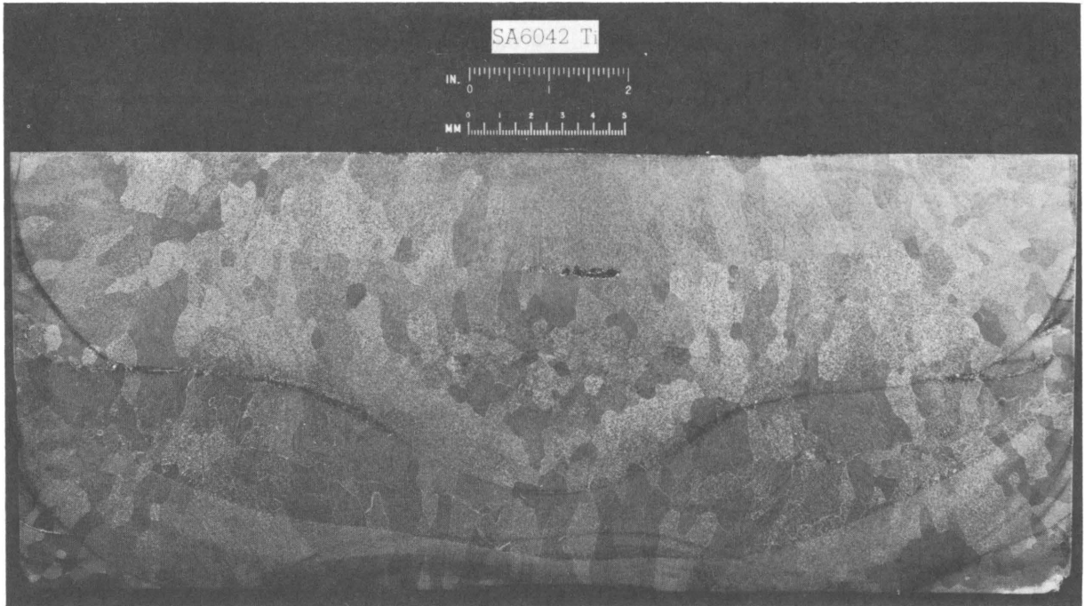
Figure 86.—Longitudinal section of a chilled ingot.
