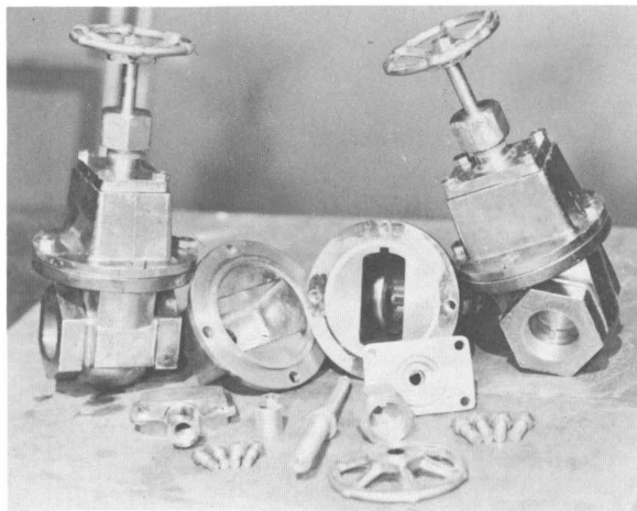
Figure 101.—Cast titanium gate valves.
