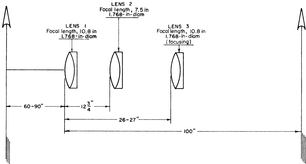
Figure 97.—Optical diagram for arc furnace projection system.
