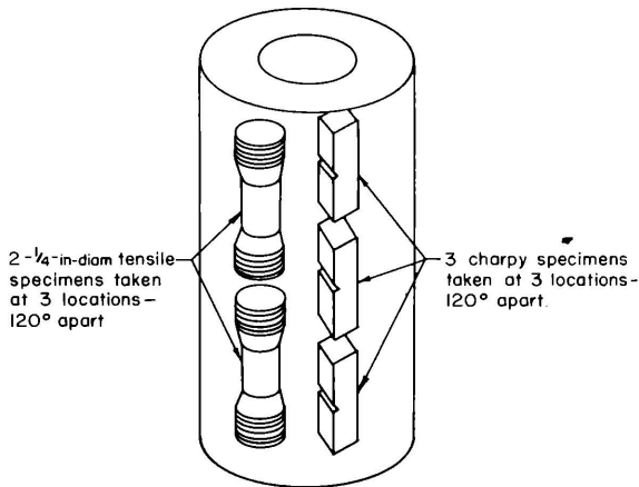
Figure 157.—Location of test specimens.
