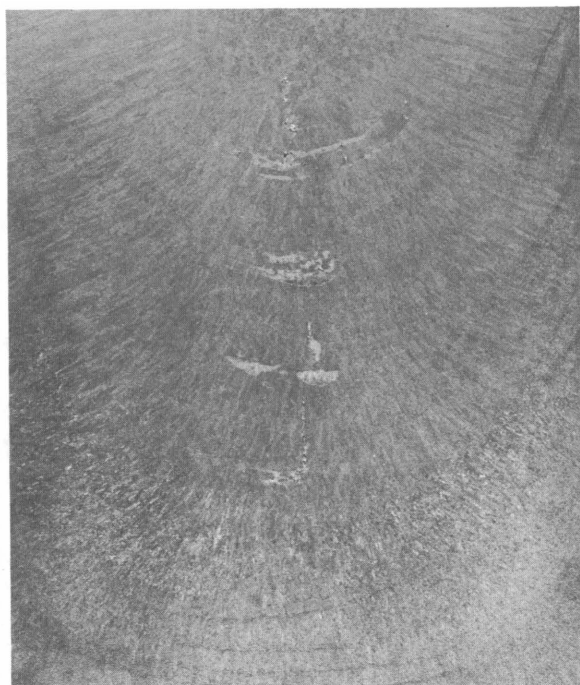
Figure 5.—Single melt ingot showing segregation of unmelted tin beads.
