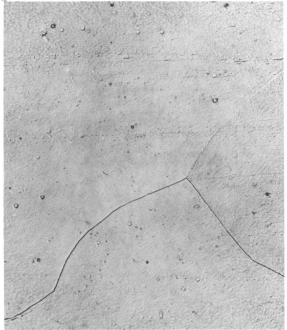
Figure 27.—Photomicrograph of oxygen-free copper vacuum-arc-melted in water-cooled copper crucible ( \times 250 ).
