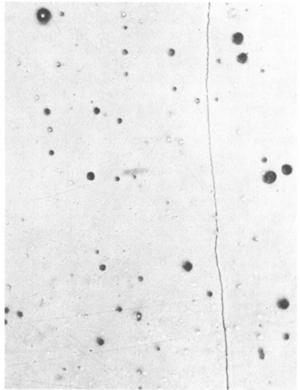
Figure 25.—Photomicrograph of electrolytic cathode copper vacuum-arc-melted in water-cooled copper crucible ( \times 250 ).
