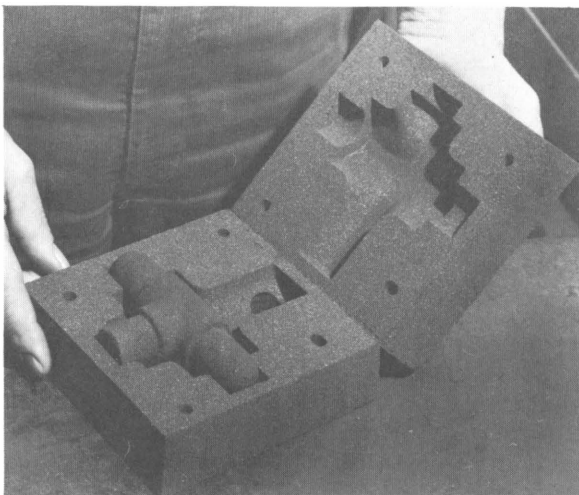
Figure 124.—Mold assembly with core in position.
