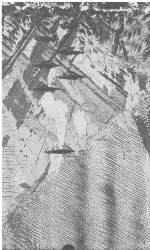
Figure 135.—Microstructure of titanium cast in XM-74 near cast surface. Etch: 45 ml H 2 O, 45 ml HNO 3 , 10 ml HF ( \times 50).
