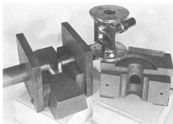
Figure 107. —Laminated mold for titanium diaphragm valve.
