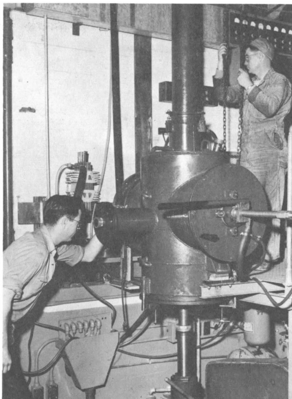
Figure 88.—Pour-over-the-lip furnace.
