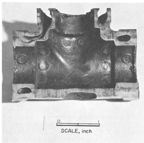
Figure 113.—Titanium casting from mold fired to 750° C.
