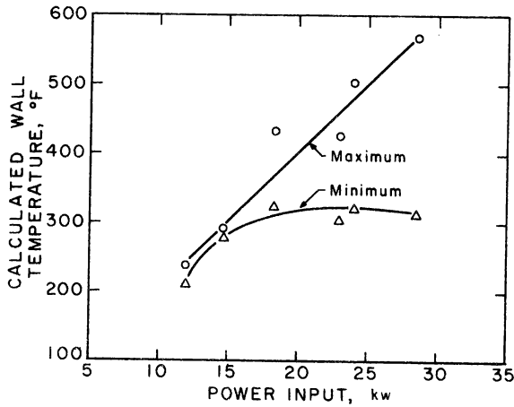
Figure 51.—Calculated temperatures of inside surface of crucible vs. power input. Non-consumable electrode, 2.5/16-in zirconium ingot.
