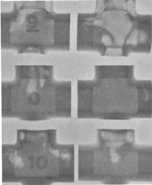
Figure 126.—Radiograph of castings from unvented molds.
