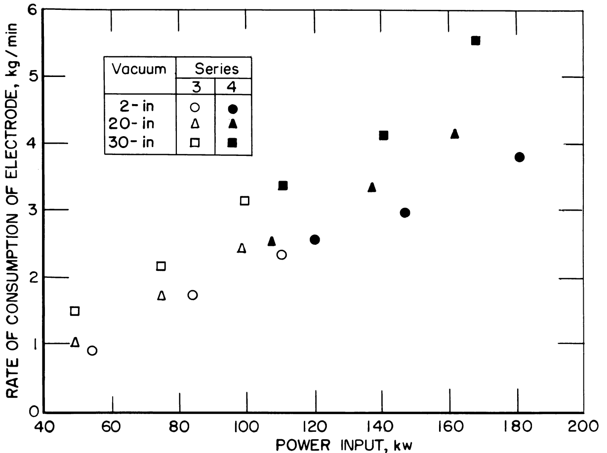
Figure 39.—Rate of consumption vs. power input.
