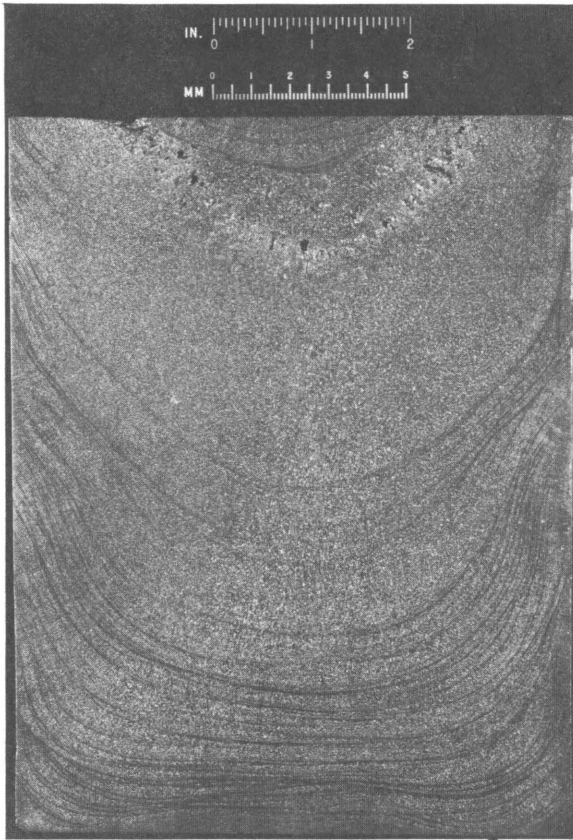
Figure 7.—Single melt solenoid stirred ingot of 0.2-amp type.
