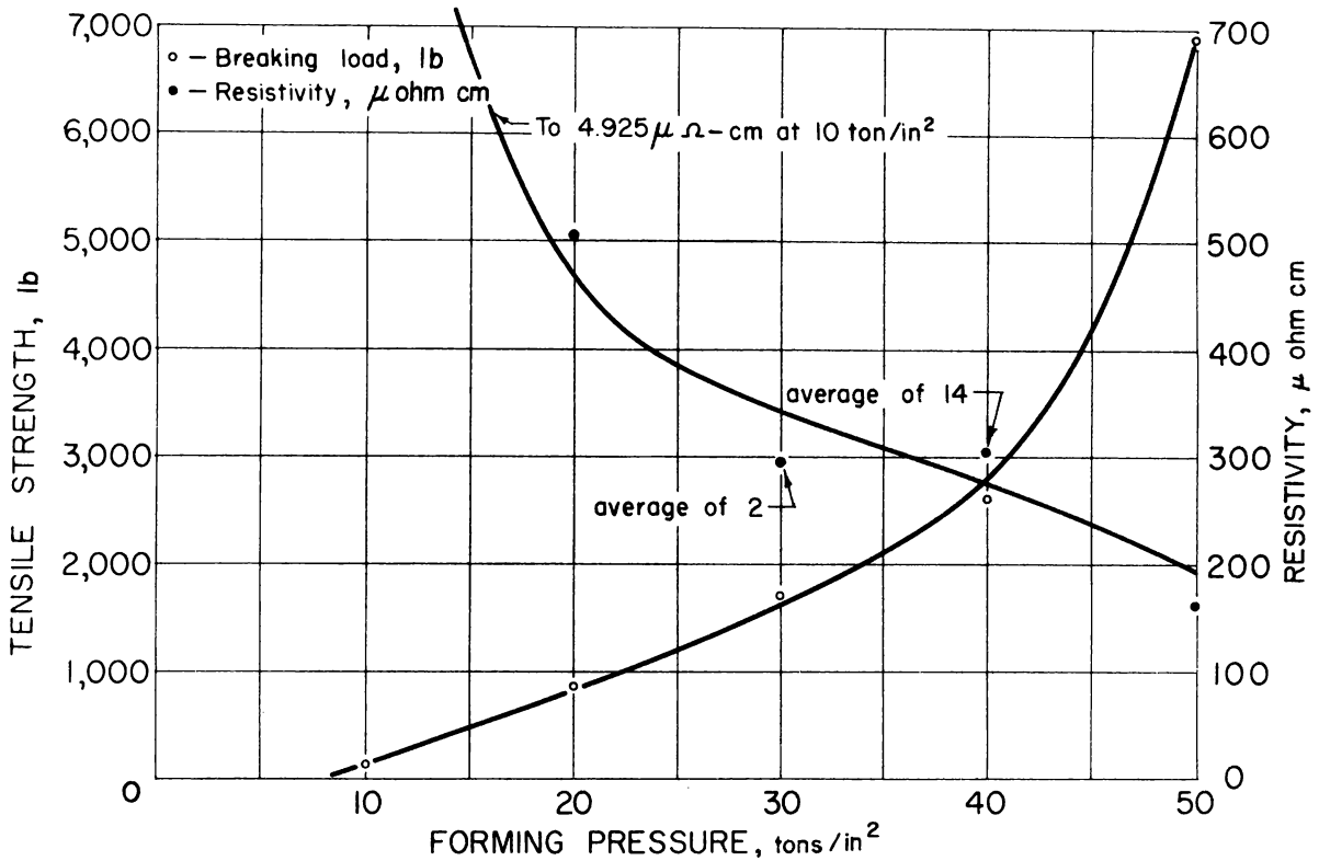
Figure 67.—Tensile strength and resistivity vs. forming pressure 2- by 2- by 20-in electrode compact.
