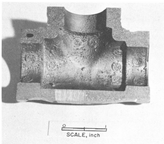
Figure 114.—Titanium casting from mold fired to 960° C.
