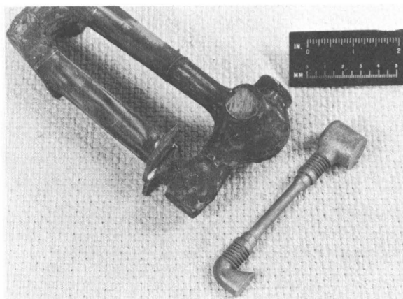
Figure 112.—Titanium castings from frozen mercury molds provided by Kolkast, Inc.
