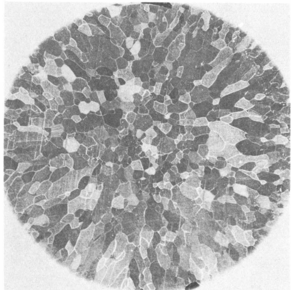
Figure 158.—Cross section of fluidity runner ( \times 6 ).
