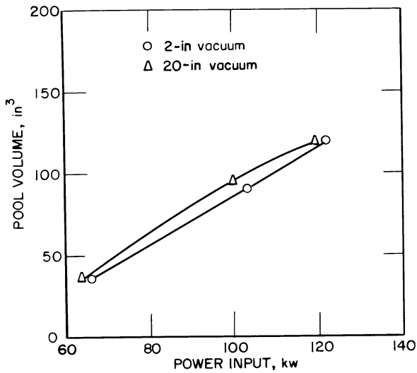
Figure 37.—Pool volume vs. power input, series 6 (alternating current).
