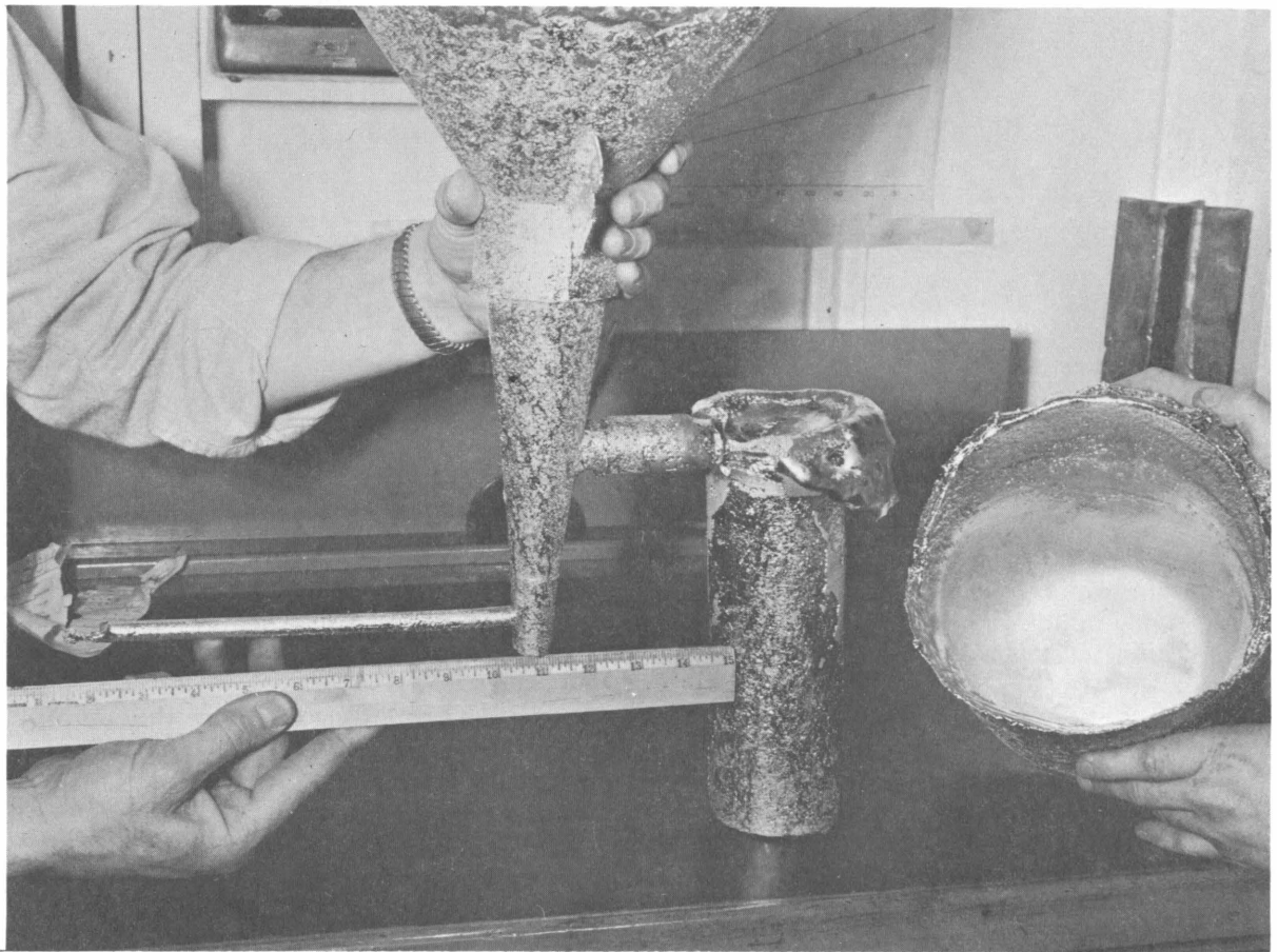
Figure 152.—Fluidity test runner and melting crucible skull, both of cast molybdenum.
