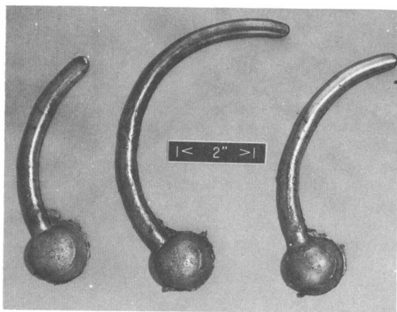
Figure 149.—Three fluidity spirals of zirconium run (left to right) at 3,500, 4,500, and 5,000 amp.
