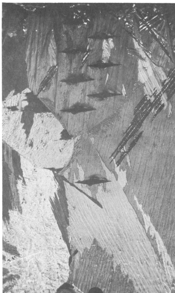
Figure 136.—Microstructure of titanium cast in XM-75 near cast surface. Etch: 45 ml H 2 O, 45 ml HNO 3 , 10 ml HF ( \times 50).
