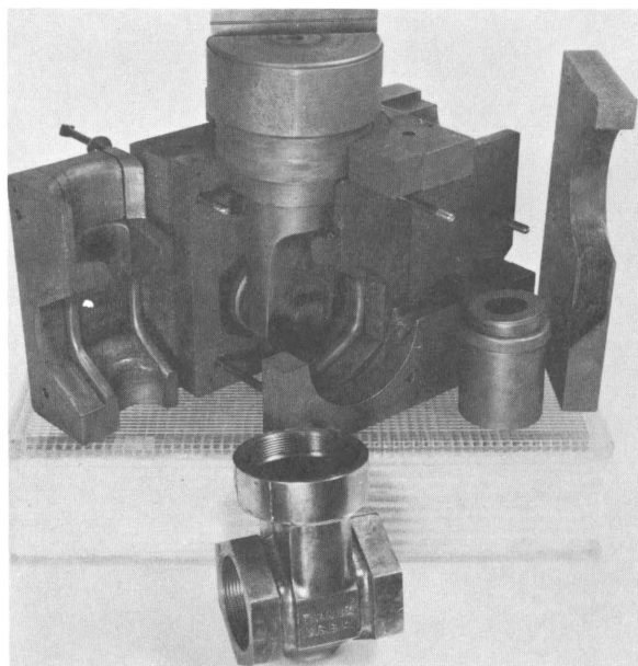
Figure 106. —Laminated mold for titanium gate valve.
