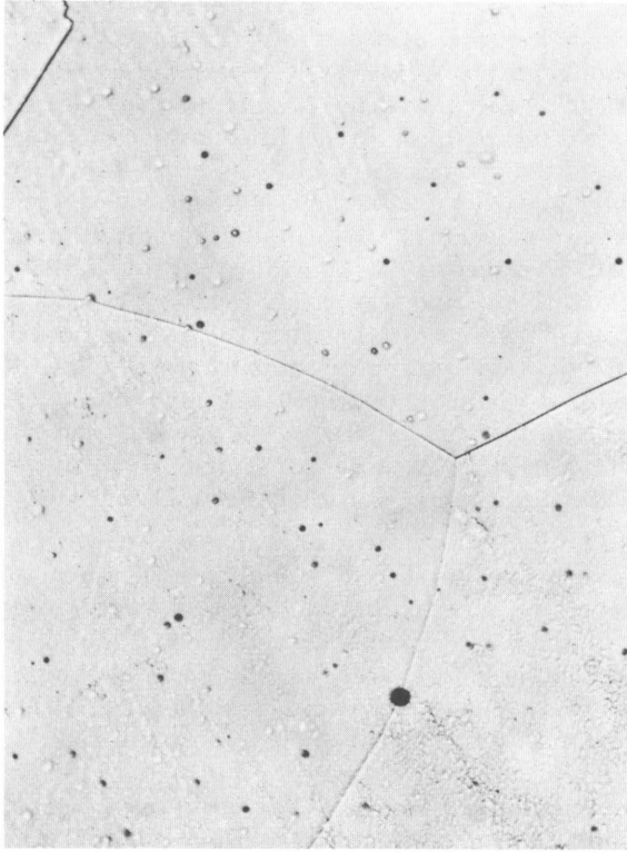
Figure 24.—Photomicrograph of electrolytic cathode copper vacuum-arc-melted in graphite-lined crucible ( \times 250 ).
