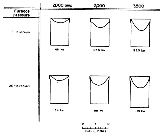
Figure 34.—Pool shapes for series 6 (alternating current).
