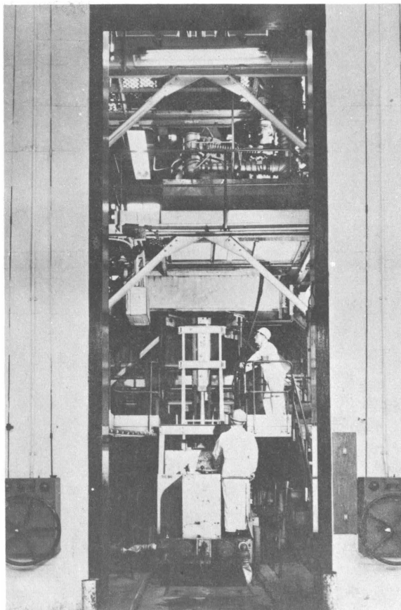
Figure 14.—An Imperial Metals Industries Ltd. arc furnace during unloading operation.
