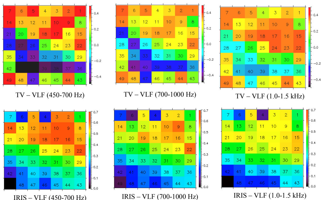
Figure 5. Spatial distribution of correlation between particle precipitation and ELF/VLF waves in three frequency bands during event of January 8, 1997, 02:20-02:35UT: top row- for TVASC data, bottom row - for IRIS data. Value of linear Pearson correlation coefficient presented by color coding in IRIS beams array. Note, that for bottom row the scintillation due to Cassiopeia is located in beam 4, and due to Cygnus - in beams 6 and 7.
