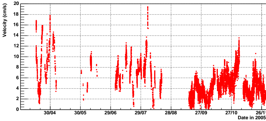
Fig. 11. Velocity of the water current flow measured by the Doppler current profiler, as a function of time over a period of eight months.
