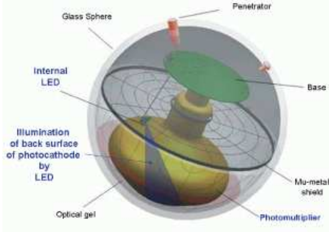
Fig. 2. Sketch of the ANTARES Optical Module (for a complete description, see ref [2]).
