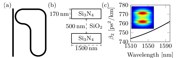
Fig. 2. (a) A top view of the layout of the resonator, with a bus waveguide-resonator gap of 1000 nm and a total length of 6031.86 \mu\text{m} . (b) A schematic of the 2D cross section of the waveguide geometry. (c) Dispersion simulation around 1550 nm for the fundamental TE mode with the inset showing the simulated power distribution of the mode.
