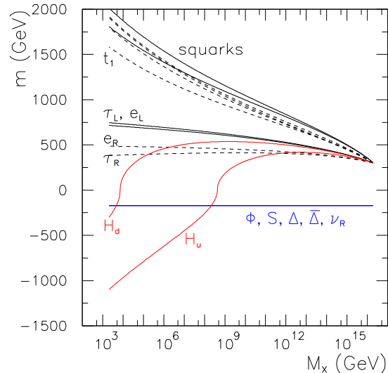
FIG. 2: Renormalization group evolution of the scalar masses (with m \equiv \text{sign}(m_o)\sqrt{|m_o^2|} ) for a representative choice of parameters (see text).
