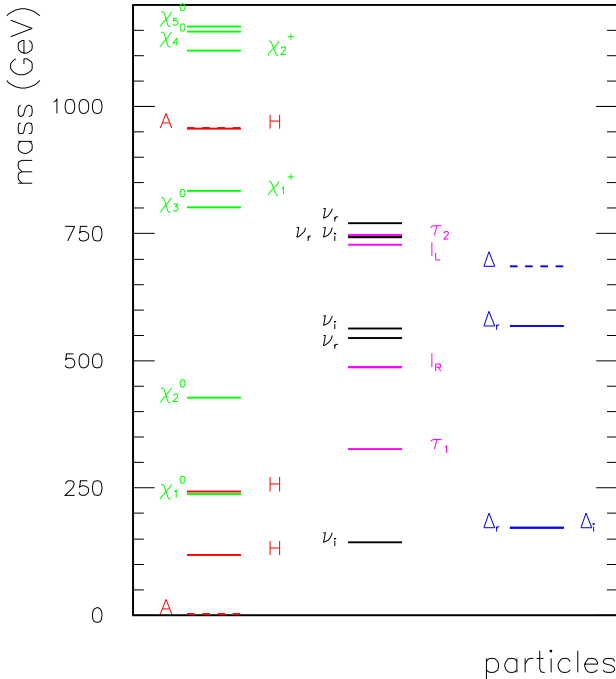
FIG. 3: Supersymmetric spectrum for the same choice of parameters as in Fig. 2. The real(imaginary) sneutrino state is labelled as \nu_r(\nu_i) , the scalar(pseudoscalar) of the secluded sector is indicated as \Delta_r(\Delta_i) and the singlino as \Delta . Gluino and squark masses are larger than 1.5 TeV and not shown.
