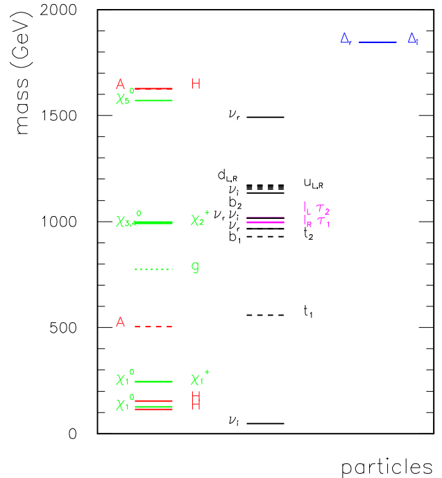
FIG. 4: Same as in Fig. 3, but for a different choice of input parameters, with larger \lambda_1 and \lambda_2 , and a small \tan\beta , as described in the text.
