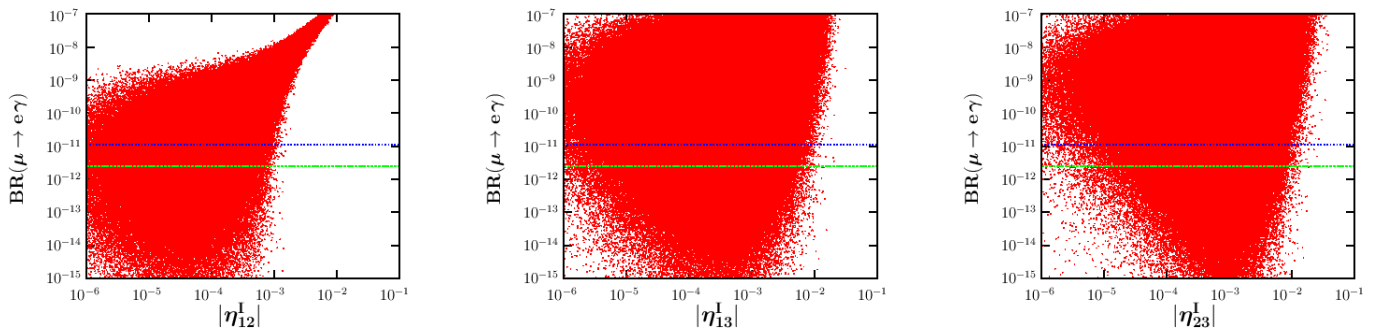
FIG. 4: Same as Fig. 3 for the Inverted Hierarchy (IH) case.
